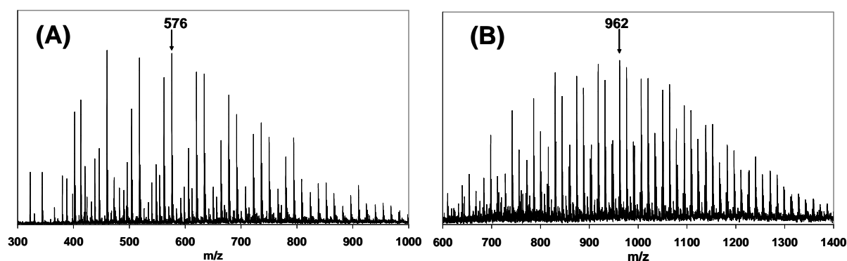
FIGURE B.1 – Spectres MALDI-TOF de (A) la Jeffamine M600 et (B) la Jeffamine M1000.
