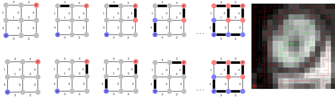
Figure 1.7: Illustration of two Maximum Spanning Forest (MSF) algorithms behavior, and segmentation result on a real image.
