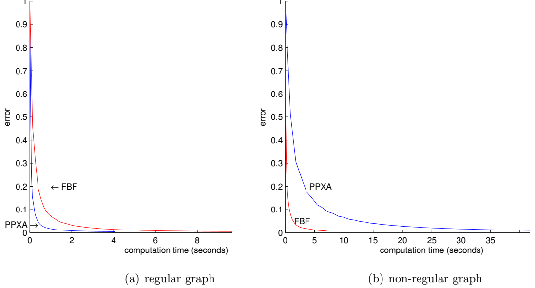
Figure 3.7: Comparison of convergence speed of the PPXA (blue) and M+SFBB (red) algorithms for denoising an image.
