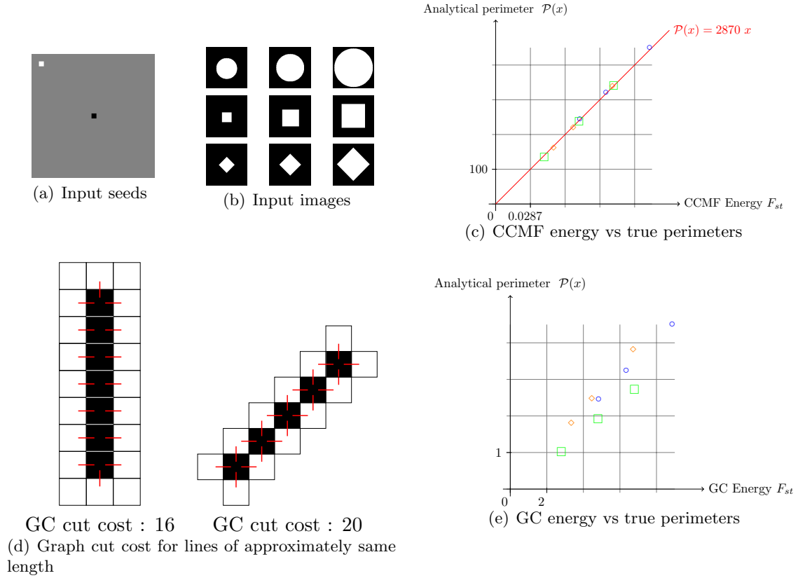
Figure 2.6: Comparison of perimeters computed analytically and with Graph cuts and CCMF. To estimate the boundary length with CCMF, segmentations have been produced using the input images in (b) with the foreground and background seeds that appears in (a). (c) : plot showing the linear relation between the true perimeters and the energies obtained with CCMF. The symbols used to represent the dots correspond to the objects segmented in the images. A similar relation of proportionality is obtained with CP-TV. (d) : value of the cut obtained for a diagonal and a vertical line of approximately same length using graph cuts. The difference observed explains (e) : plot showing the nonlinear relation between the true perimeters and the energies obtained with Graph cuts.
