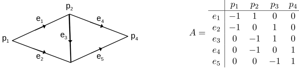
Figure 1.2: A graph and its incidence matrix A \in \mathbb{R}^{m \times n} .
