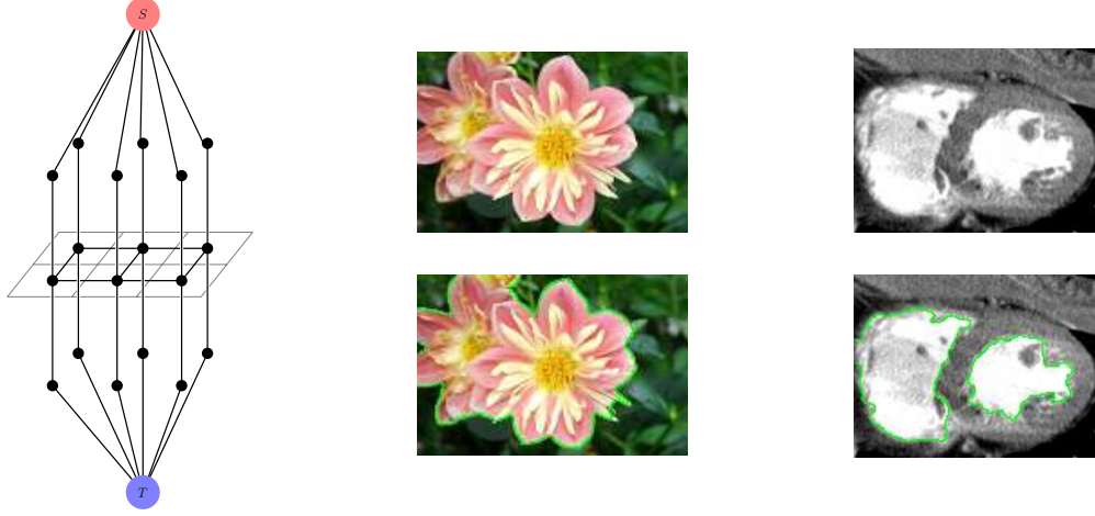
Figure 2.9: Example of graph construction to incorporate unary terms for unsupervised segmentation.
