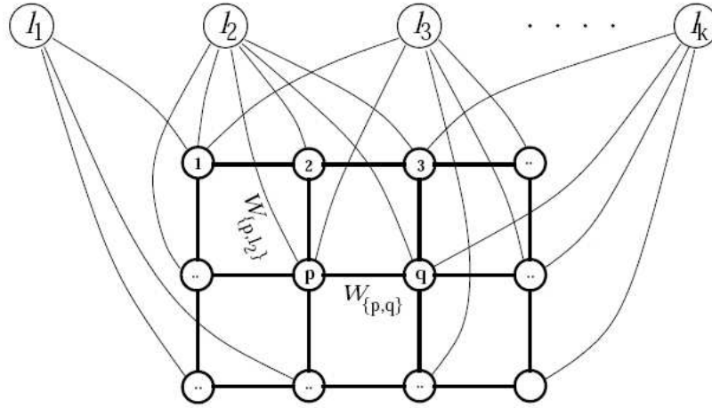
Figure 5.7: Possible graph construction for the stereo application.
