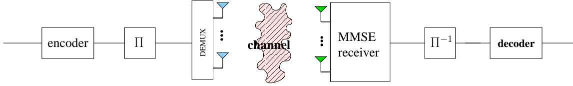
Figure 2.1: Considered MIMO system
