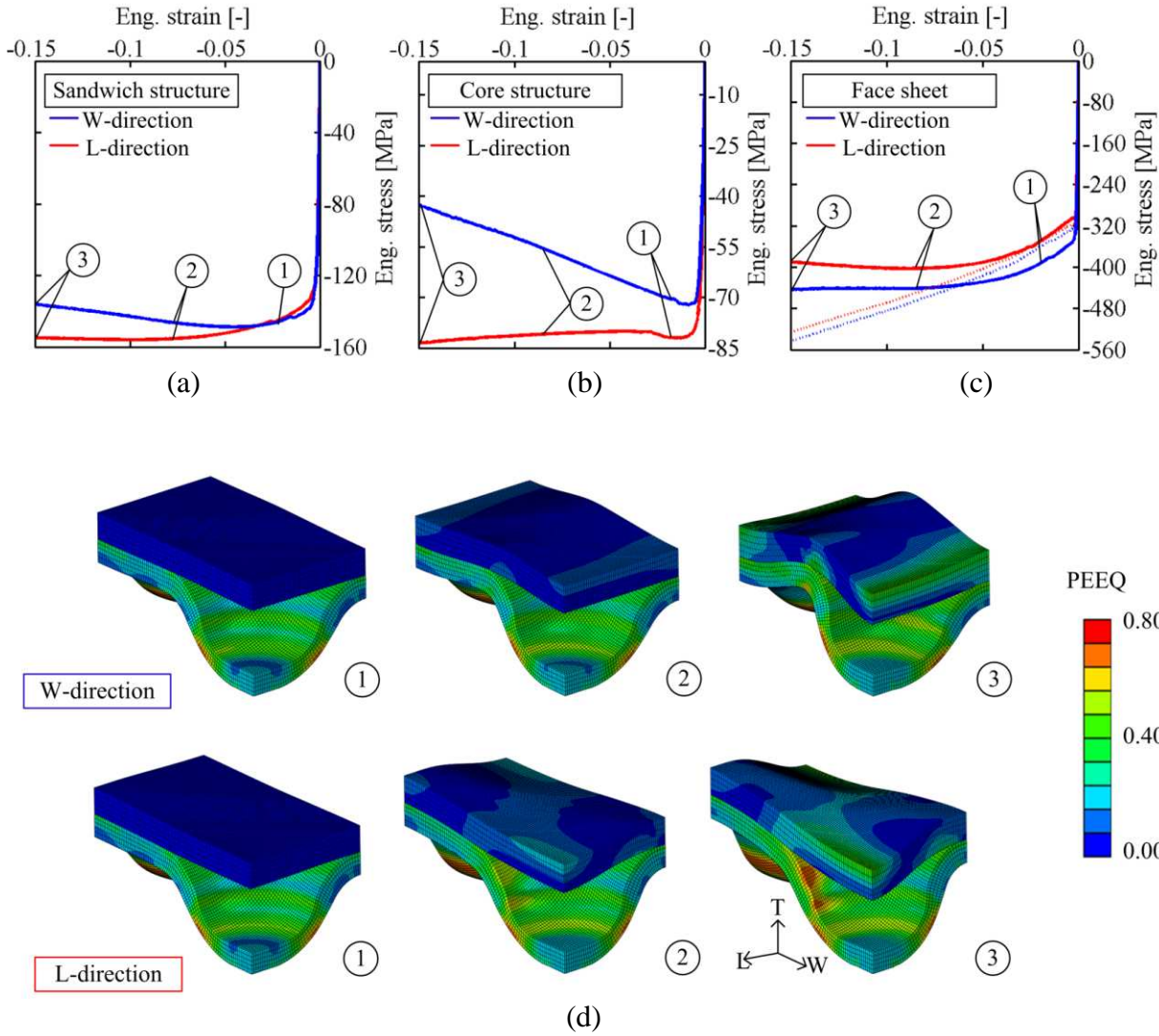
Fig. 3.7 : Uniaxial in-plane compression: engineering stress-strain curves for (a) entire sandwich cross-section, (b) the core structure, and (c) the face sheets; (d) 3D views of the deformed configurations corresponding to the points labeled in the stress-strain curves.
