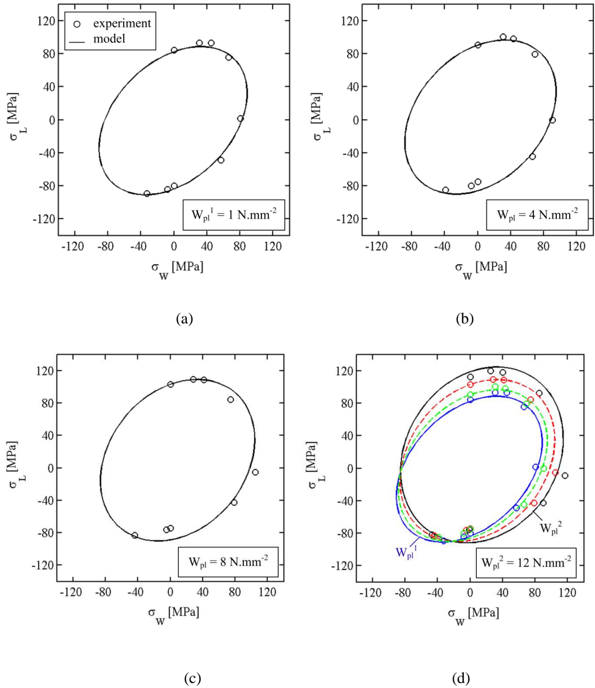
Fig. 3.11 : Envelopes of equal plastic work (per unit initial volume) for the core structure in the true stress plane ( \sigma_W, \sigma_L ). The open dots present the results from virtual experiments, the black solid lines in (a) and (d) represent the least square fit of the yield function given by Eq. (3.16). The solid envelopes in (b) and (c) have been computed based on the isotropic-distortional hardening model given by Eq. (3.25).
