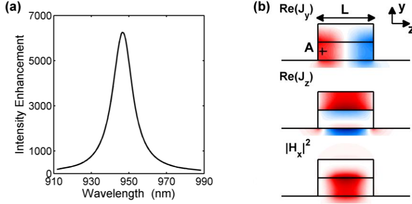
Figure 6-2. Magnetic resonance of a single MIM nanoresonator. (a) Spectrum of the intensity enhancement |\mathbf{E}|^2/|\mathbf{E}_{\text{inc}}|^2 at the point A in (b) for a resonator ( w = 40 nm, t_d = 20 nm and L = 70 nm) illuminated by a plane wave impinging from air at normal incidence and polarized along the z -direction. (b) Distribution of the induced current \mathbf{J} (see the text for its definition) and of the magnetic field |\mathbf{H}_x|^2 at resonance in the (y, z) plane ( x = 0 ). Blue and red colors correspond to negative and positive values. The induced current is localized under the resonator and forms a loop in the (y, z) plane.
