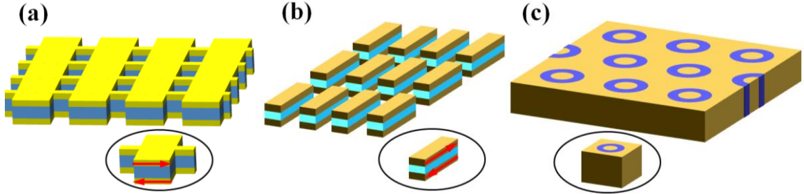
Figure 1-8. Negative index metaterial designs for optical frequencies and their corresponding metaatoms (in the circles). (a) Sketch of fishnet metamaterial that consists of alternating layers of metallic and dielectric thin films perforated by a hole array [Zha05]. (b) Cut-wire pair array as negative index metamaterial. Cut-wire pair array composed of pairs of metallic cut-wires separated by an insulator [Sha05, Lin05]. (c) Hexagonal array of subwavelength coaxial waveguides. The coaxial waveguide consists of a dielectric annular channel embedded in metal [Bur10]. In (a) and (b), the red arrows indicate the intuitive picture of current loops that are supported by the functional unit.
