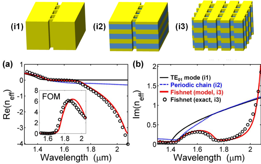
Figure 4-6. Model predictions for (a) the real part and (b) the imaginary part of the effective index. For building up the negative index of the fishnet, we study successively with the model the TE_{01} super-mode of a 1D hole chain [inset (i1)], solid black curves], the Bloch mode of a single z-periodic hole-chain [inset (i2), dashed blue curves] and the Bloch mode of the fishnet [inset (i3), solid red curves]. Results of fully-vectorial calculations of the fishnet Bloch mode are marked with circles. The figure of merit (FOM) |\text{Re}(n_{\text{eff}})|/\text{Im}(n_{\text{eff}}) is shown in the inset of (a).
