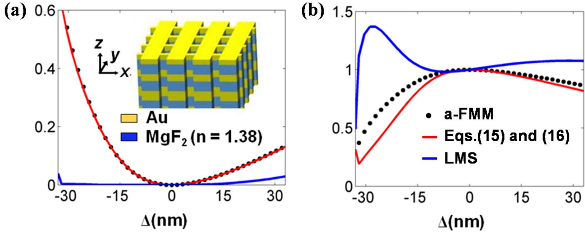
Figure 3-4. Test of closed-form expressions for an interface between two fishnet metamaterials. (a) |r_1|^2 . (b) |t_1|^2 . The fishnet parameters are those in [Val08]: the periodicity in the x - and y -directions is a_x = a_y = 860 nm, the rectangular hole dimensions are w_x = 295 and w_y = 595 nm. The refractive index of \text{MgF}_2 is 1.38 and the gold permittivity is -142 + 18.7i at \lambda = 1.9 \mu\text{m} . The calculation is performed for Bloch modes with H_y(x) = H_y(-x) . The inset sketches the fishnet geometry.
