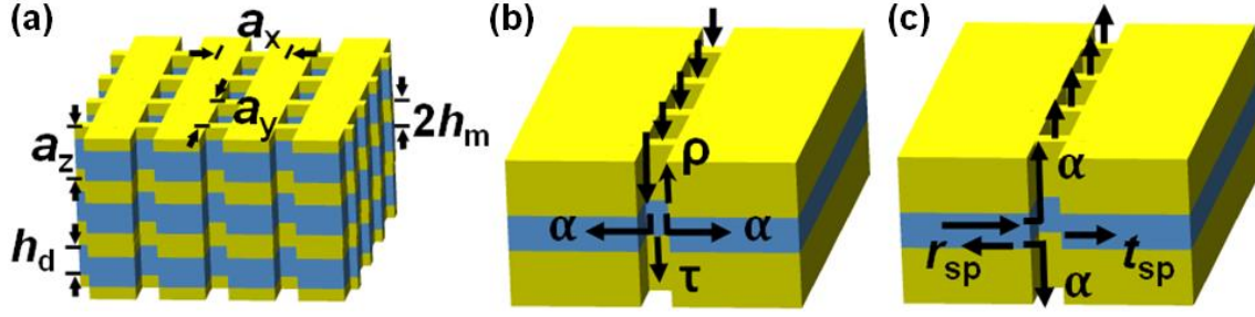
Figure 4-1. Elementary scattering events involved in a fishnet. (a) The fishnet under study is a two-dimensional array (period a_x = a_y = 860 nm) of rectangular holes (width w_x = 295 nm and w_y = 595 nm) etched into an Ag ( h_m = 50 nm)-MgF 2 ( h_d = 50 nm)-Ag ( h_m = 50 nm) periodic stack. The refractive index of MgF 2 is n_d = 1.38 and the frequency-dependent permittivity of silver is taken from [Pal85]. (b) Scattering of the super-mode of a 1D metallic hole chain. (c) Scattering of the gap-SPP mode supported by a MIM waveguide. The scattering processes depicted in (b) and (c) define five elementary scattering coefficients, the reflection \rho and transmission \tau of the super-mode, the reflection r_{sp} and transmission t_{sp} of the gap-SPP, and the coefficient \alpha of coupling between the gap-SPP and the super-mode.
