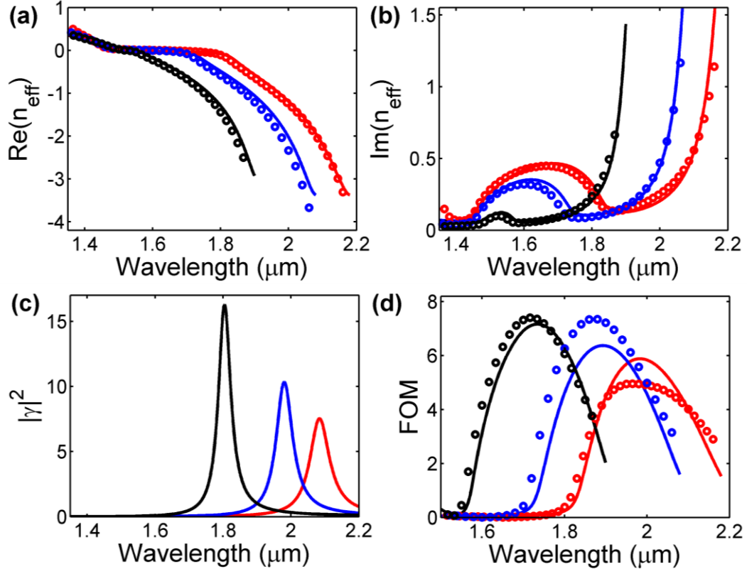
Figure 5-2. Real (a) and imaginary part (b) of the fishnet effective index for different dielectric spacer thickness h_d = 40 nm (red), 50 nm (blue) and 75 nm (black). The x-period is fixed as a_x = 860 nm. Corresponding multiple-scattering parameter |\gamma|^2 (c) and Figures of Merit |\text{Re}(n_{\text{eff}})|/\text{Im}(n_{\text{eff}}) (d). In (c), the three Q factors are 30 (red), 35 (blue) and 40 (black) respectively. In (a), (b) and (c), the model predictions and the fully-vectorial calculations are shown as solid curves and circles, respectively.
