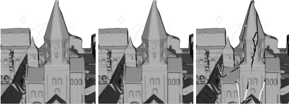
Figure 7.6: Cluny-26-Big: (Level 1) refined meshes are smoothed with 30 Laplacian operations. Left to right: mesh with serial refinement, mesh is merged from 8 partial refined sub-meshes, union of these 8 refined sub-meshes. There is visually no crack in merged mesh, which prove the success of the merging algorithm.
