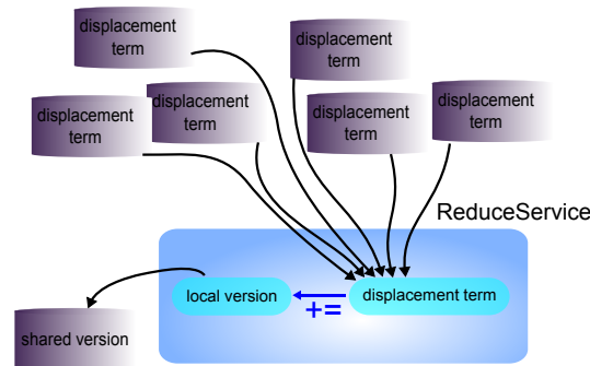
Figure 7.2: Overview of the ReduceService instance processing the “reducing task”. This QueueService builds the shared version by computing the sum of all the available displacement terms sent by the ProcessService instances in the BlobStorage.
