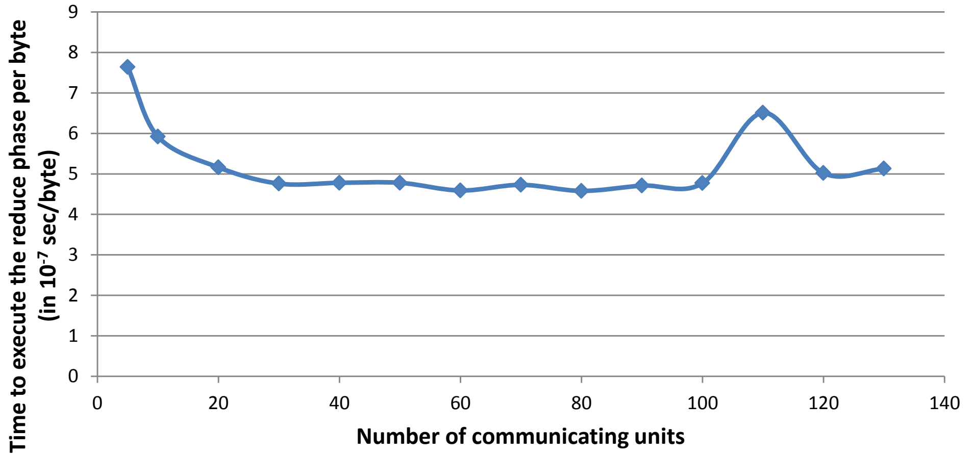
Reduce phase duration per byte in function of the number of communicating units
