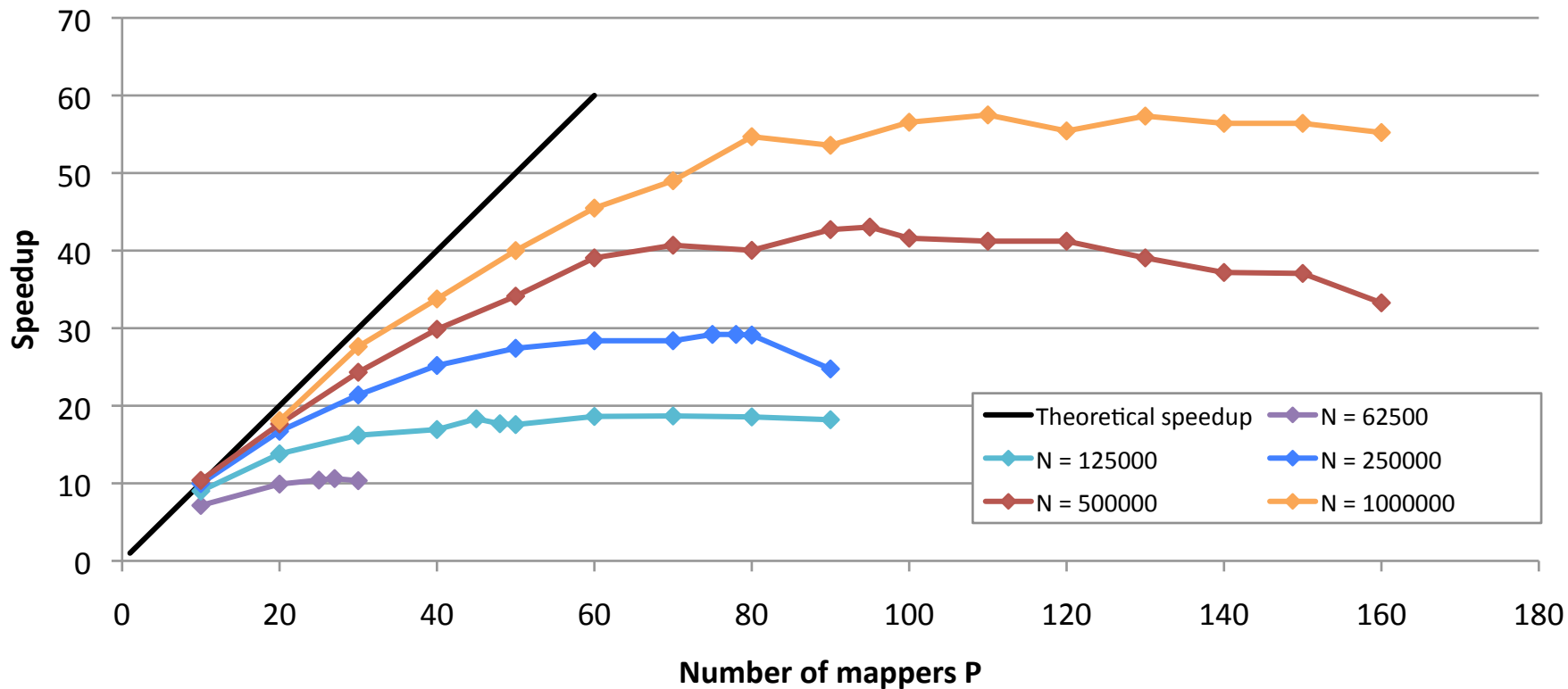
Speedup in function of the number of mappers
