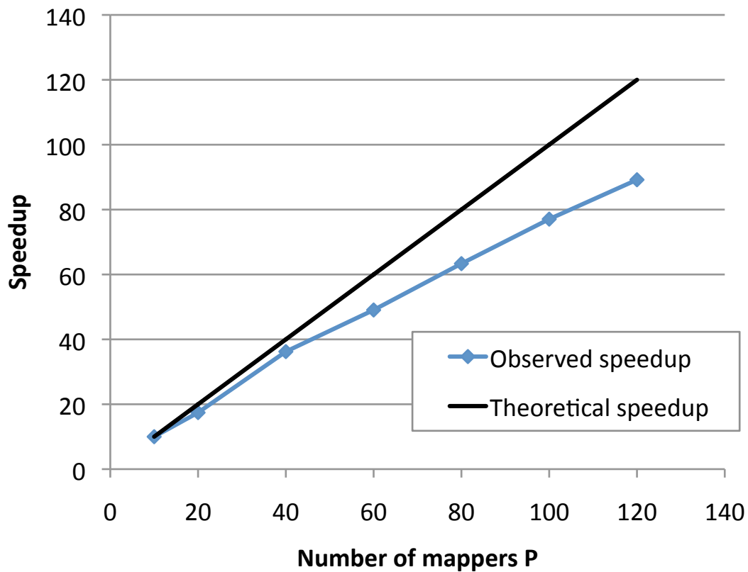
Speedup in function of the number of mappers
