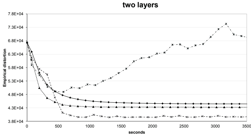
Figure 7.5: Normalized quantization curves with M = 8, 16, 32, 64 instances of ProcessService and with an extra layer for the so called “reducing task”. Our cloud DAVQ algorithm has good scalability properties for the quantization performance up to M = 32 . However, the algorithm behaves badly when the number of computing instances is raised to M = 64 .
