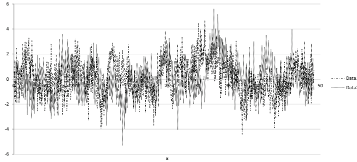
Figure 6.4: Plot of two independent realizations of the random variable \mathbf{Z} defined by equation (6.4): \bar{B}_1, \dots, \bar{B}_4 where G = 1500 , d = 1500 , \chi = 50 , sc = 10 .
