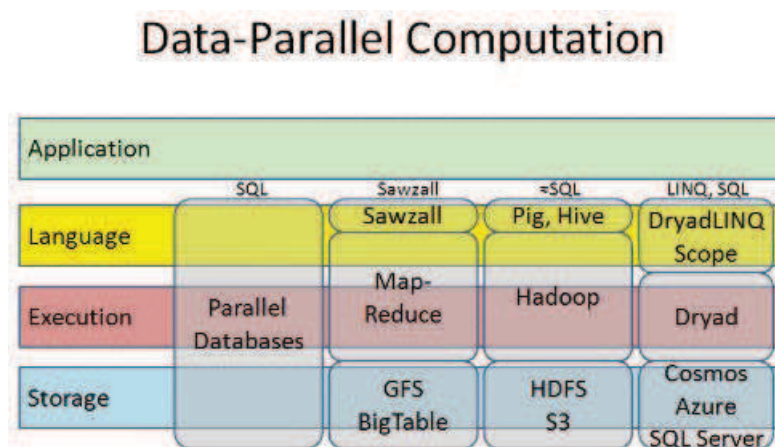
Figure 2.1: Illustration of the Google, Hadoop and Microsoft technology stacks for cloud applications building. For each stack, the DSL Level, the Execution Level and the Storage Level are detailed. In this scheme, SQL is also described as a stack in which the three levels are merged together and cannot be used independently.
