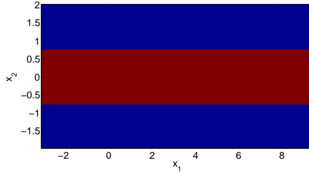
Figure 2.5: Strip structure with constant contrast plotted in (-\pi, 3\pi) \times (-2, 2) .
