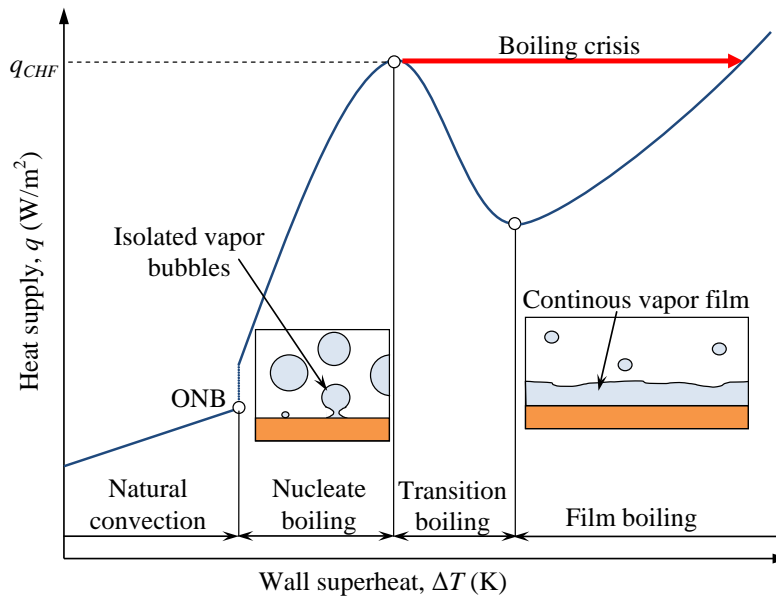
Figure 1.4: Boiling curve
