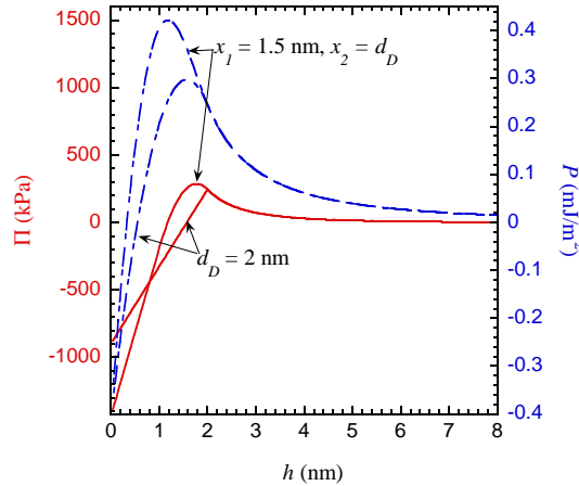
Figure C.1: The two shapes of disjoining pressure (Eqs. (2.106) and Eqs. (C.1)) and corresponding surface energies for water at 10 MPa, \theta_Y = 15^\circ , \theta_{micro} = 1^\circ and A = 3.7 \cdot 10^{-20} J.
