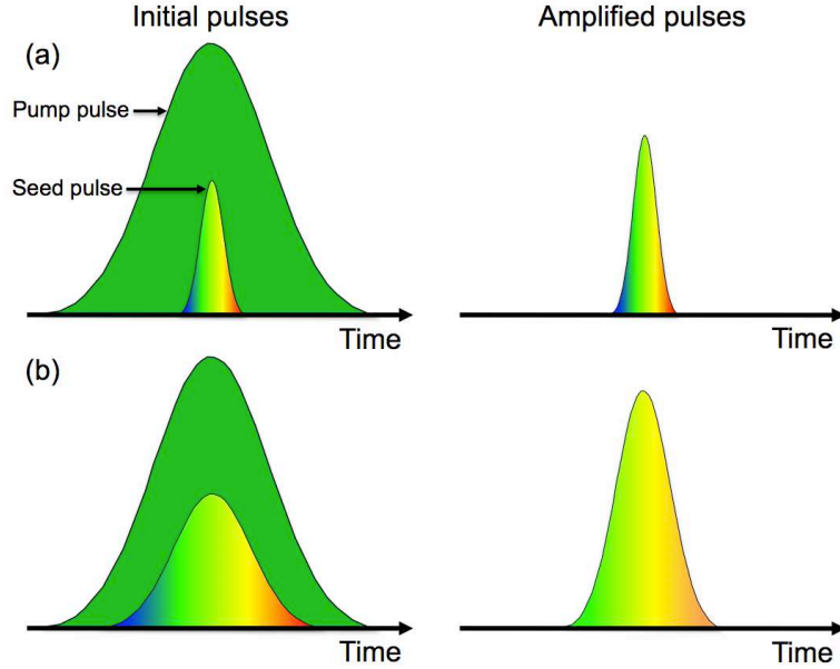
Figure 4.1.1. Demonstration of the effect of the pump and seed pulse duration on the bandwidth and conversion efficiency of OPCPA. The seed pulse is chirped and its color gradient represents the bandwidth. (a) The bandwidth of the seed is conserved when its duration is short and falls within the peak of the pump where the seed pulse experiences a more or less, constant intensity. (b) When the seed pulse is significantly stretched, the edges of the seed will experience a lower gain, owing to the lower intensities at the wings of the pump. Although higher conversion efficiencies are achieved, the bandwidth of the amplified pulse decreases simultaneously.
