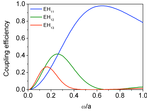
Figure 3.2.5. Coupling efficiencies of the first three EH_{lm} modes with respect to the ratio of the beam waist and bore radius.
