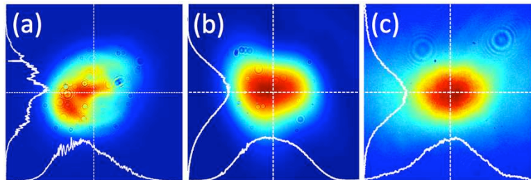
Figure 3.5.2. Spatial profiles in the hollow waveguide setup. (a) Unfiltered, out of focus spatial profile and (b) filtered, out of focus profile of the beam incident on the BaF 2 crystal, (c) XPW spatial profile.
