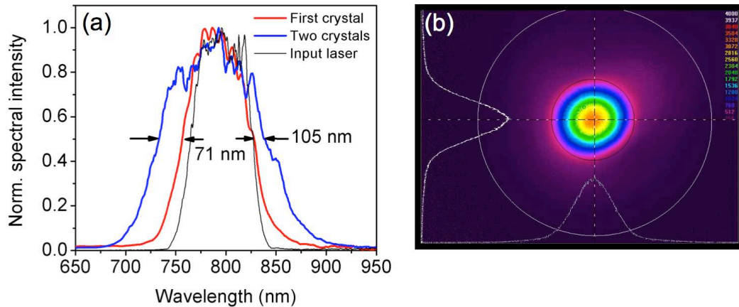
Figure 3.6.9. (a) Spectra from the first crystal (red), two-crystal setup (blue) and input laser (black, FWHM = 60 nm) and (b) spatial profile of the XPW beam.
