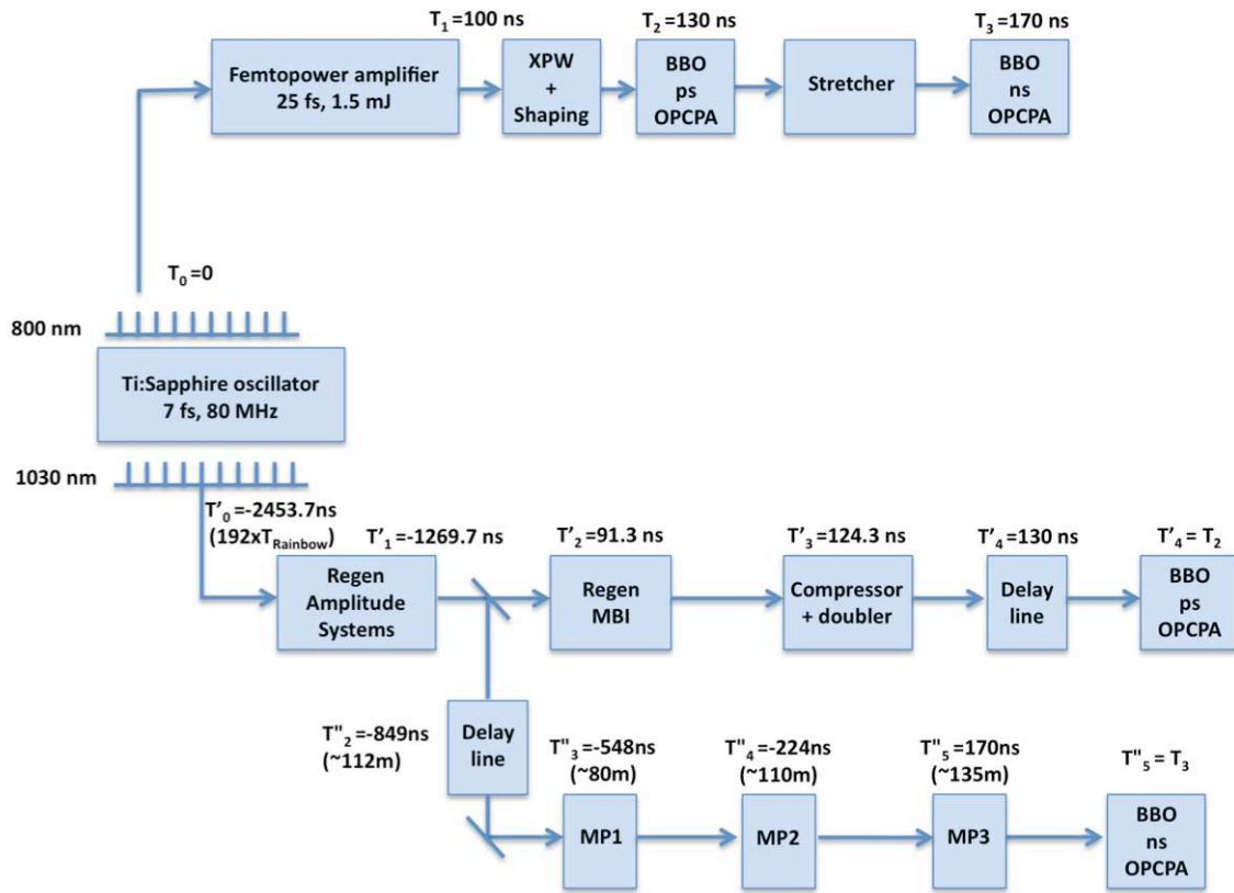
Figure 2.4.1. Timing diagram for the synchronization of seed and pump pulses at the picosecond and nanosecond OPCPA stages.
