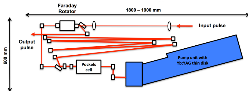
Figure 2.3.4. Schematic of the MBI amplifier which consists of a regenerative cavity built around a Yb:YAG thin disk gain medium.
