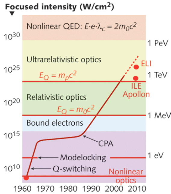
Figure 1.1.2. Curve depicting the increase in laser intensity through the years and different regimes accessible with higher intensities.
