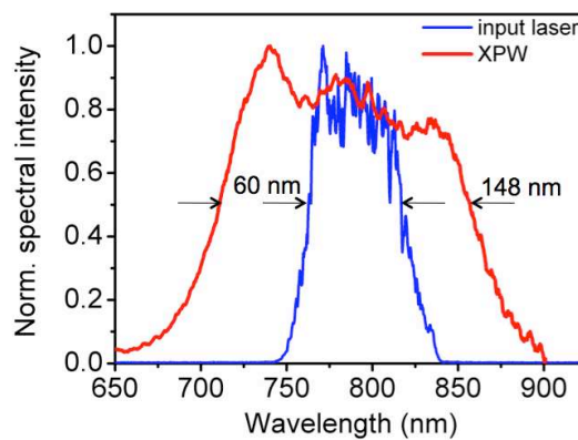
Figure 3.5.6. The input laser spectrum with a FWHM of 60 nm is broadened via XPW and SPM to >140 \text{ nm} .
