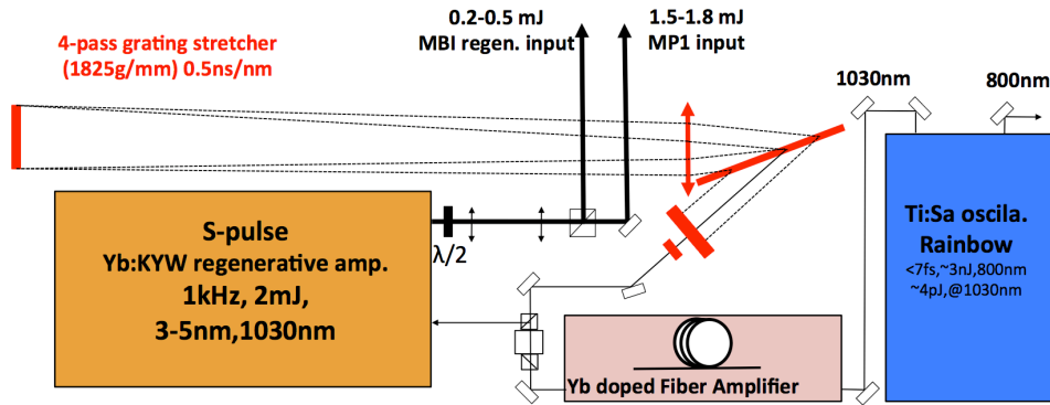
Figure 2.3.1. Schematic of the amplification of the 1030 nm output from the ultrabroadband oscillator. Pre-amplification occurs in a Yb-doped fiber amplifier, the pulse is stretched and then further amplified in a commercial regenerative amplifier.
