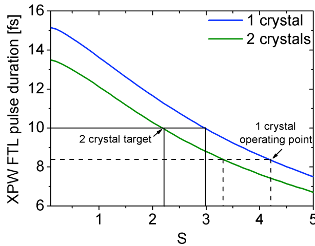
Figure 3.6.7. XPW FTL pulse durations obtained from a single crystal (2 mm, blue) and two-crystal (1mm-2mm, green) setup. The experimental operating point (8.4 fs FTL) for the single crystal setup is indicated by the dashed lines and is obtained at S = 4.2 for the single crystal setup and at S = 3.3 for the two-crystal setup. The target for the two-crystal setup was 10-fs pulses which shown by the solid lines is achievable at S = 3 for the single crystal setup and at S = 2 for the two-crystal setup.
