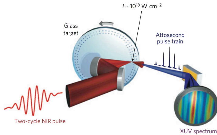
Figure 1.1.4. Generation of an attosecond pulse train with a few-cycle, high intensity pulse. When laser intensities reaching \sim 10^{18} W/cm 2 are incident on a glass target, a plasma is formed which is capable of reflecting the laser pulse. Simultaneously, attosecond light bursts are emitted as a result of coherent wake emission [Tha 07]—a process involving the interaction of the laser with the electrons in the plasma. The image is from [Bor 12].
