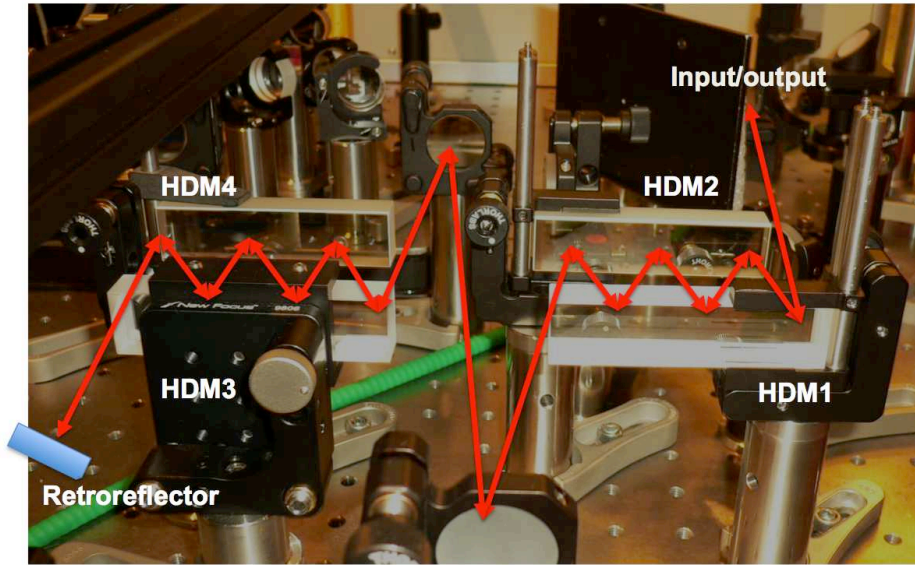
Figure 5.4.4. High dispersion mirror compressor for the first stage. The input enters the compressor at small angle to have at total of 36 bounces in the first pass and an additional 36 bounces after retroreflection, for a total of 72 reflections. A simplified beam path is represented by the red lines.
