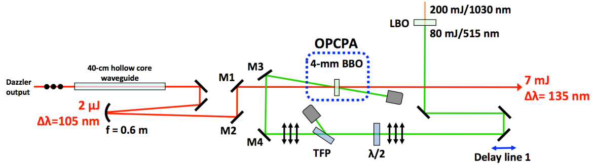
Figure 5.3.1. Setup for single stage OPCPA. The 2- \mu\text{J} signal beam is indicated in red and was s -polarized (dot). The 1030 nm, compressed output of the MBI (orange) was converted into 515 nm (green) by an LBO crystal. The pump beam was p -polarized (arrows) and its energy was controlled with a half waveplate ( \lambda/2 ) and thin film polarizer (TFP).
