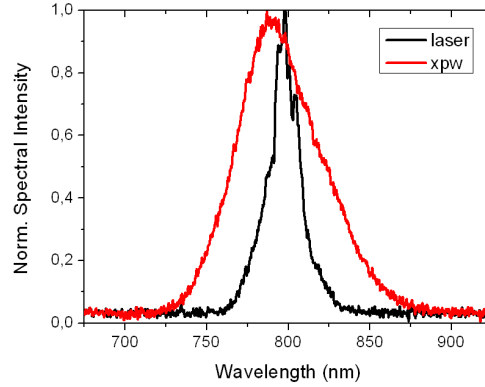
Figure 3.5.10. Spectrally broadened laser via XPW and SPM. The initial spectrum (black) supports 50-fs pulses while the Fourier transform limit of the XPW spectrum (red) is 20 fs.
