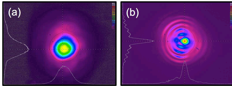
Figure 4.4.2. (a) Spatial profile of the beam before it entered the Dazzler (diameter = 1.5 mm). (b) Spatial profile of the fundamental beam as it was compressed from -6.9 \text{ ps} down to -500 \text{ fs} due to the positive dispersion introduced by the \text{TeO}_2 crystal of the Dazzler.
