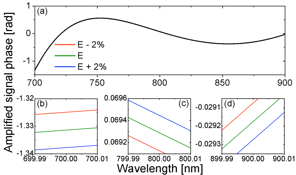
Figure 5.2.4. (a) Signal phase of the whole spectrum after amplification with a pump intensity of 12 \text{GW}/\text{cm}^2 . The phase with variations in input intensity of \pm 2\% are overlapped in the graph, represented by a single black curve. Zoomed in plots of the signal phase at (b) 700 nm, (c) 800 nm and (d) 900 nm show their slight differences.
