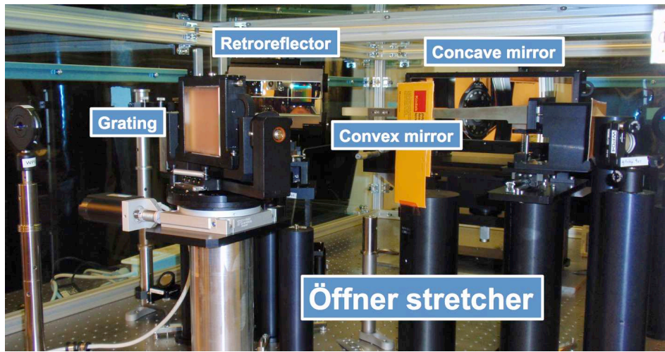
Figure 2.1.5. Öffner stretcher which will stretch the ps-pulses to 1 ns for the nanosecond OPCPA stage.
