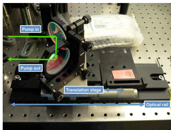
Figure 2.4.2. Picture of the delay line for the picosecond OPCPA stage. Two mirrors are mounted on a translation stage for fine delay adjustment of and coarse adjustment with translation on an optical rail.
