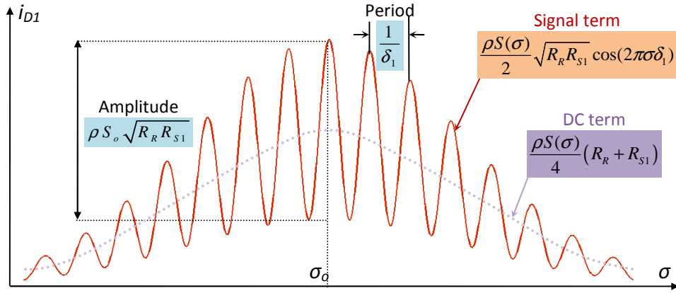
Figure 3.2 The detected current at the output of the spectrometer for a single reflector in air.
