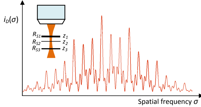
Figure 3.4 Illustration of the spectral interferogram corresponding to multiple sample reflectors with various reflectivities R_{S1} , R_{S2} and R_{S3} located at different axial positions z_1 , z_2 and z_3 . The signal term is the superposition of the spectral interferograms related to the individual reflectors.
