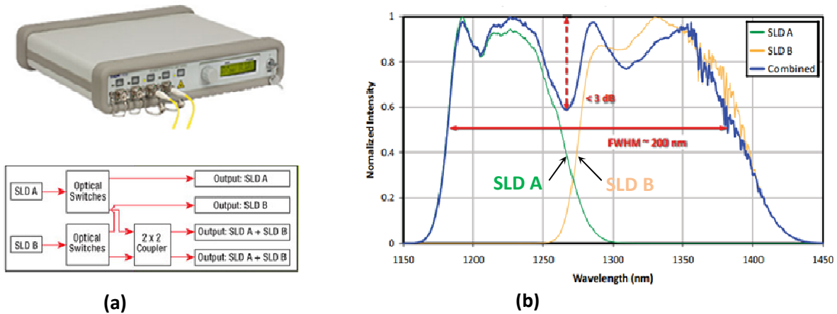
Figure 3.9 (a) Compact SLD broadband light source (Thorlabs, LS2000B), (b) typical mission power spectra: SLD A (green curve) and SLD B (yellow curve) and the spectrum of the combined shown in blue. An Effective spectral bandwidth ~ 200 nm at FWHM can be achieved.
