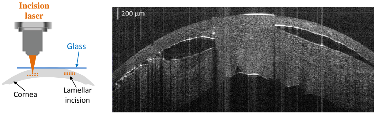
Figure 5.12 OCT image of two lamellar laser incisions in cornea realized by 0.4 NA objective and a laser pulse energy of around 2 \mu\text{J} .
