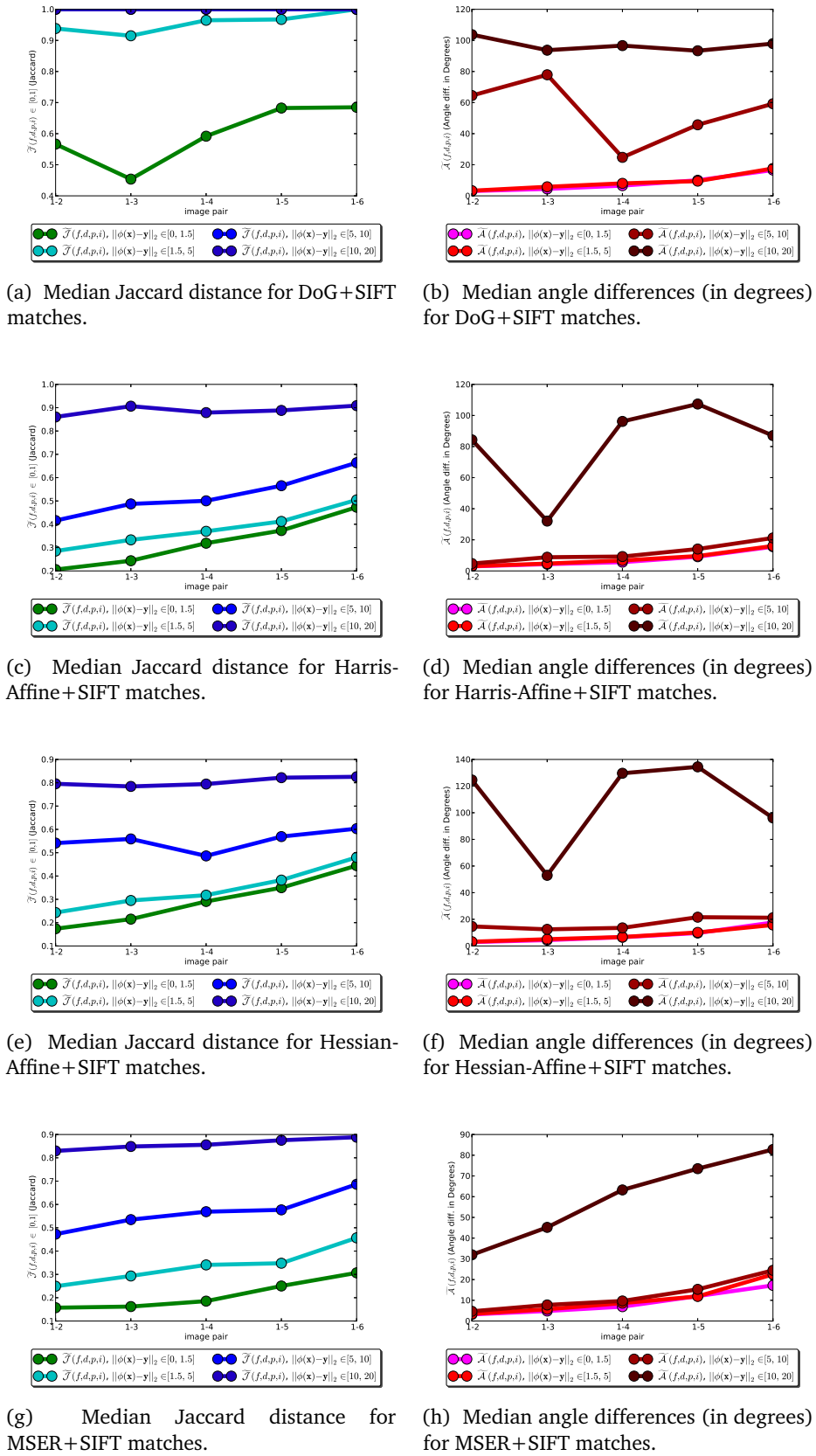
Figure D.10: Median values for Wall dataset.
