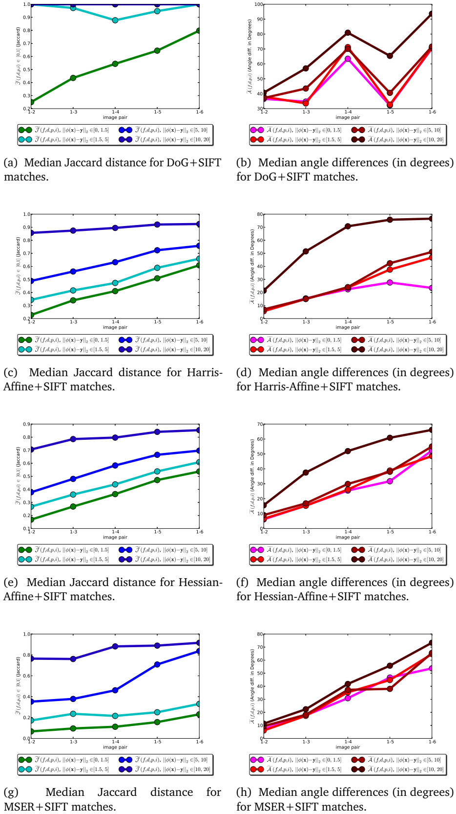
Figure D.6: Median values for Graffiti dataset.
