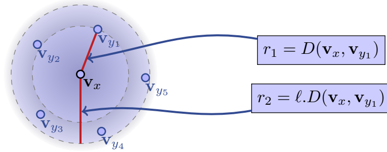
Figure 5.1: Illustration of the distrust score L . Nearest neighbors \{v_{y_i}\}_{i=2}^5 in \mathcal{Y} to v_x lie in the annulus with center v_x , inner radius r_1 = D(v_x, v_{y_1}) and outer radius r_2 = \ell \cdot D(v_x, v_{y_1}) . As a reminder: L(x, y_1) \leq 1 and 1 \leq L(x, y_i) \leq \ell for i \geq 2 .
