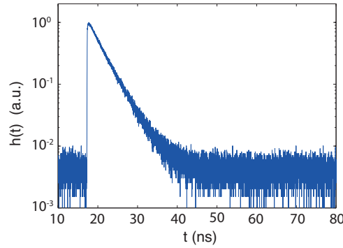
Figure 2.4: Histogram of the photons arrival times h(t) for one fluorescent bead at one position. This figure is taken from Ref. [66].
