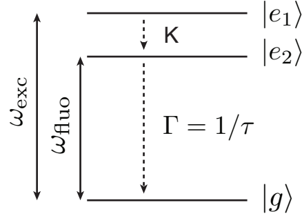
Figure 2.2: Three-level system.
