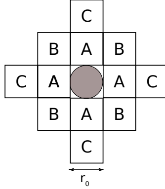
Figure D.3: Closest neighbours of a particle.
