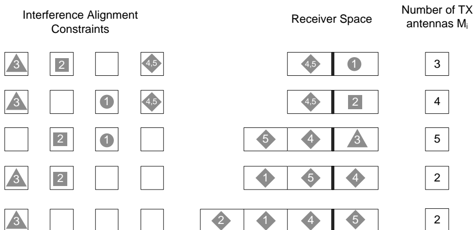
Figure 8.1: Symbolic Representation of the IA algorithm with incomplete CSIT for the tightly-feasible IC (2, 3).(2, 4).(3, 5).(3, 2).(4, 2) .
