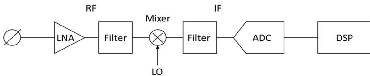
Fig.1. 11 - Common and simplified receiver architecture
