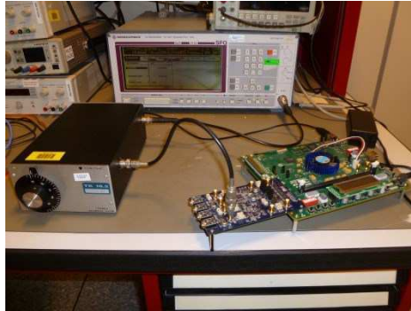
Fig.4. 12 - Overview of the testbench
