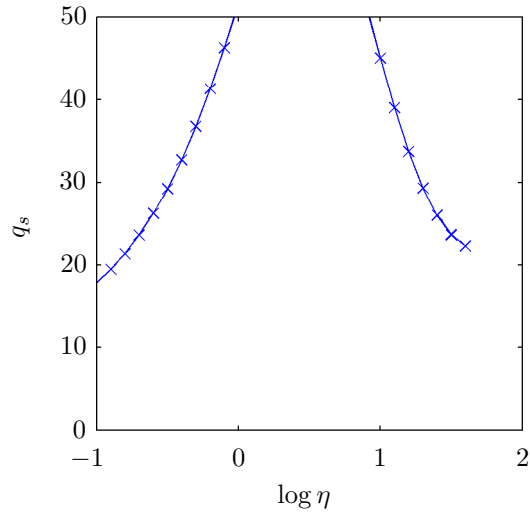
Figure 5.7: Plot of q_s estimated from the \hat{\alpha}(\eta) s and \hat{C}_1(\eta) s of the DTMs of the fractionally differentiated velocity.
