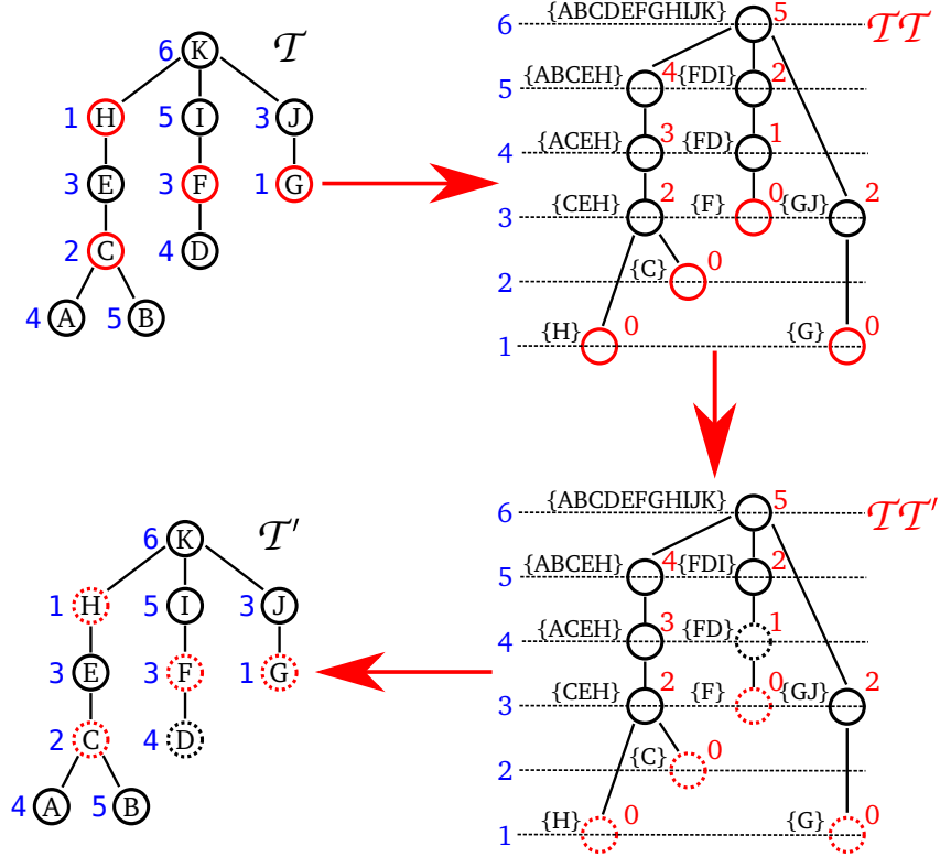
Figure 3.3: An example of the workflow of shape-based morphology with \mathcal{TT} being the Min-tree of \mathcal{T} . Circles with capital letter inside: nodes \mathcal{N} ; Blue values: first attribute \mathcal{A} ; Circles without letter inside: nodes \mathcal{NN} ; Red values: second attribute \mathcal{AA} (being the height of the first attribute \mathcal{A} in this example); Dashed circles: filtered nodes with a given threshold 2 for the second tree pruning.
