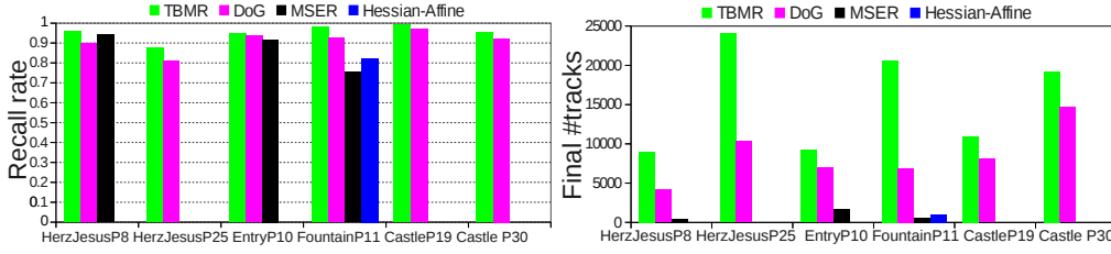
Figure 4.16: Recall rate (left) of the tracks and the absolute number (right) of final maintained tracks used to yield the sparse 3D points.
