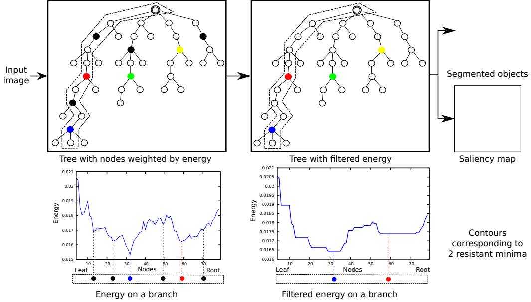
Figure 3.11: An example of the object detection scheme by spotting local minima of an attribute function \mathcal{A}_o as meaningful objects. The underlying tree representation is the topographic map, and \mathcal{A}_o is the context-based energy estimator (see Chapter 7). Filled circles: local minima; Colorized filled circles: resistant local minima after connected filtering in the shape space. Top right: detected meaningful objects surrounded by the colorized contour and a hierarchy of object detection result; Bottom: Evolution of attribute \mathcal{A}_o and filtered attribute \mathcal{A}'_o along the branch surrounded by dashed contours in the tree.
