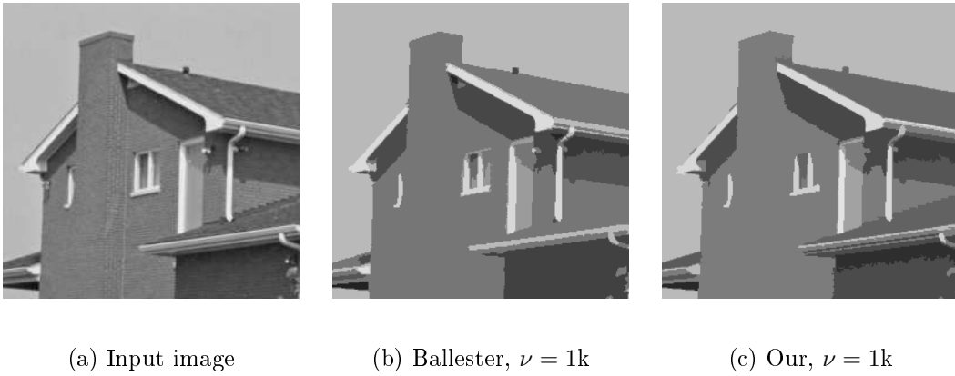
Figure 5.5: Comparison of our approach with the one of Ballester et al.. (a): E = 1.2433e + 08 ; (b): E = 1.28113e + 07 , PSNR = 27.3; (c): E = 1.15285e + 07 , PSNR = 28.7.
