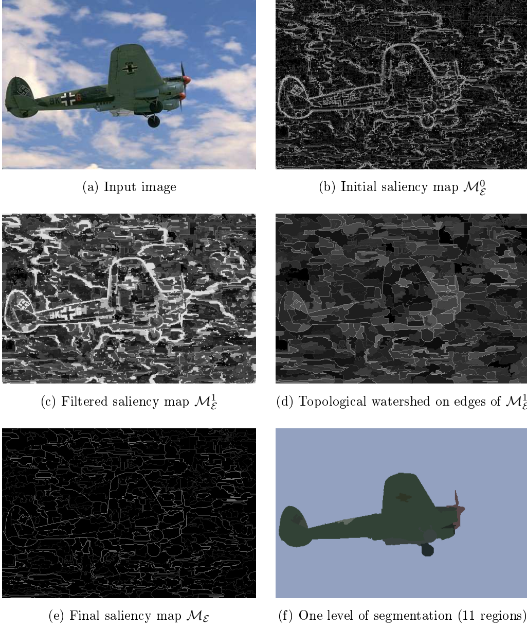
Figure 8.3: An example showing the scheme of the saliency map computation (a-e). (f): One level of segmentation by thresholding the final saliency map in (e).
