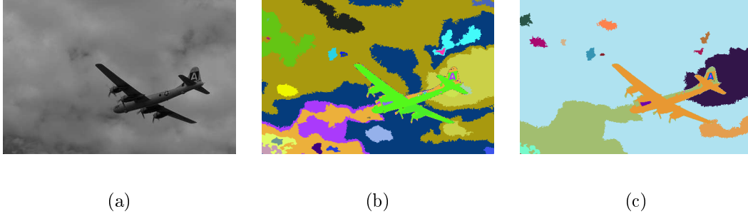
Figure 5.2: Illustration of causality principle violation. (a): input image; (b): randomly colorized simplified image with \nu = 100 ; (c): randomly colorized simplified image with \nu = 500 .
