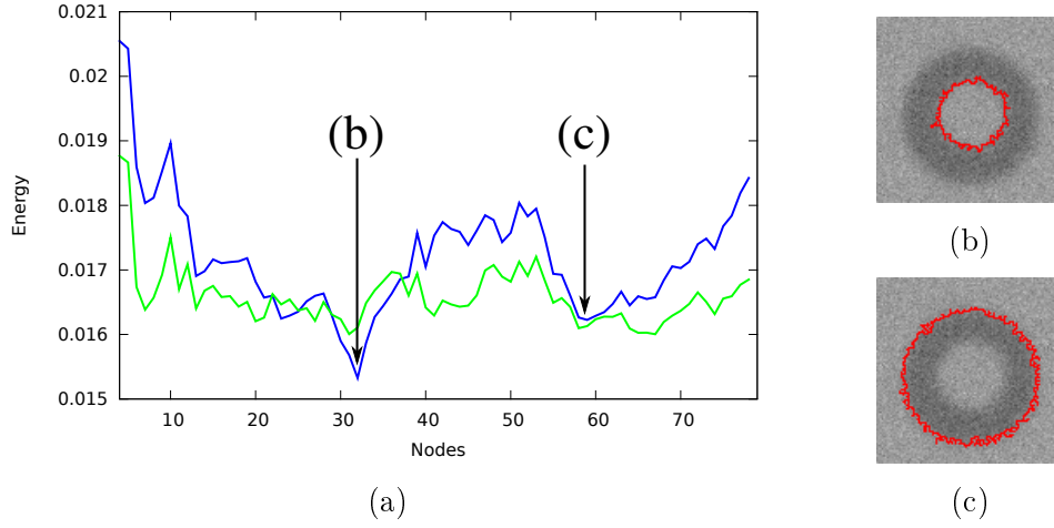
Figure 3.9: (a): Evolution of two attribute functions \mathcal{A}_o along a branch starting from a leaf (left side of Axis X) to the root (right side of Axis X). These two attribute functions \mathcal{A}_o are both based on the meaningfulness of the region boundaries: snake energy [Kass 1988] is depicted in green, and context-based energy estimator [Xu 2012] (see also Chapter 7) is in blue. (b) and (c): the boundaries of two regions corresponding to significant energy minima in the shape space given by the topographic map.
