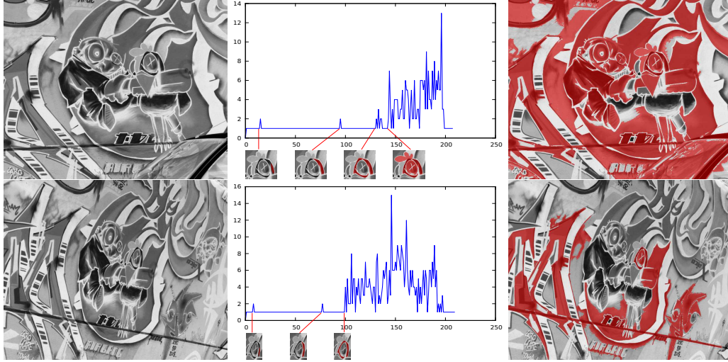
Figure 4.3: An example of TBMR extraction. Left: Front view (top) and 30° view (down) of “Graffiti” scene [Mikolajczyk 2005]. Middle: Evolution of number of children starting from a leaf to the root and some extracted TBMRs along the branch; Right: first TBMR containing the TBMRs illustrated in middle column (though they are actually too large).
