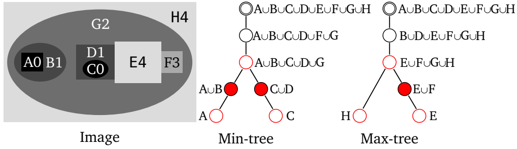
Figure 4.2: A synthetic image and the corresponding Min-tree (middle) and Max-tree (right) representation. The critical nodes are represented by red circles: (1) nodes having more than one child, and (2) leaf-nodes. The filled nodes are the TBMRs.
