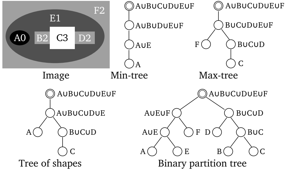
Figure 2.4: Tree-based image representations. The root is at the top represented by double circle. The numbers in the original image denote the pixel values.
