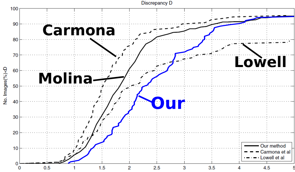
Figure 6.8: Accumulated discrepancy results for our detection method versus Carmona et al, Molina et al. and Lowell et al.
