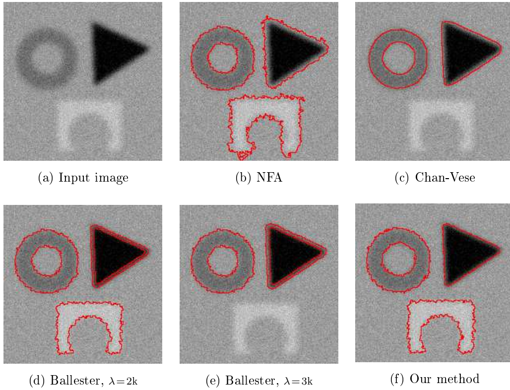
Figure 7.4: Comparison with three other methods.
