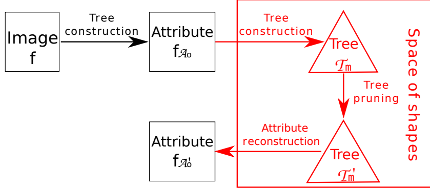
Figure 3.10: Tree pruning based connected filtering applied in the shape space. The first tree-based image representation along with the attribute function \mathcal{A}_o is seen as an image f_{\mathcal{A}_o} defined subordinated to the shape space. The second tree representation build from the image of attribute f_{\mathcal{A}_o} is a Min-tree \mathcal{T}_m .
