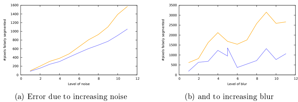
Figure 7.5: Evolution of number of falsely segmented pixels (ordinate) w.r.t. increasing noise and blur (abscissa) for the synthetic image in the Figure 7.4(a); NFA error evolution is depicted in orange and our method error in blue.
