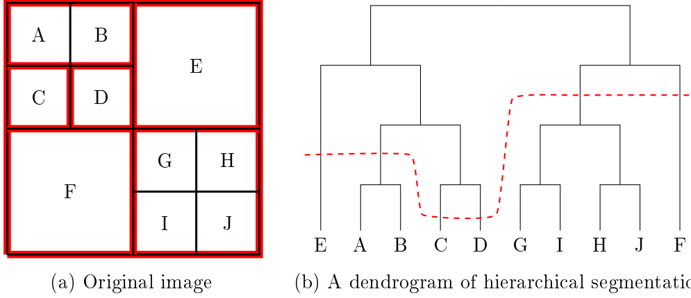
Figure 2.8: A synthetic image (a), and its associated dendrogram (b) representing a hierarchy of image segmentation. Note that there are possible partitions that are not spanned by the dendrogram. The red dashed curve in (b) is a cut of the dendrogram ( i.e. , hierarchy), the partition given by this cut is illustrated with red boundaries in the original image (a).
