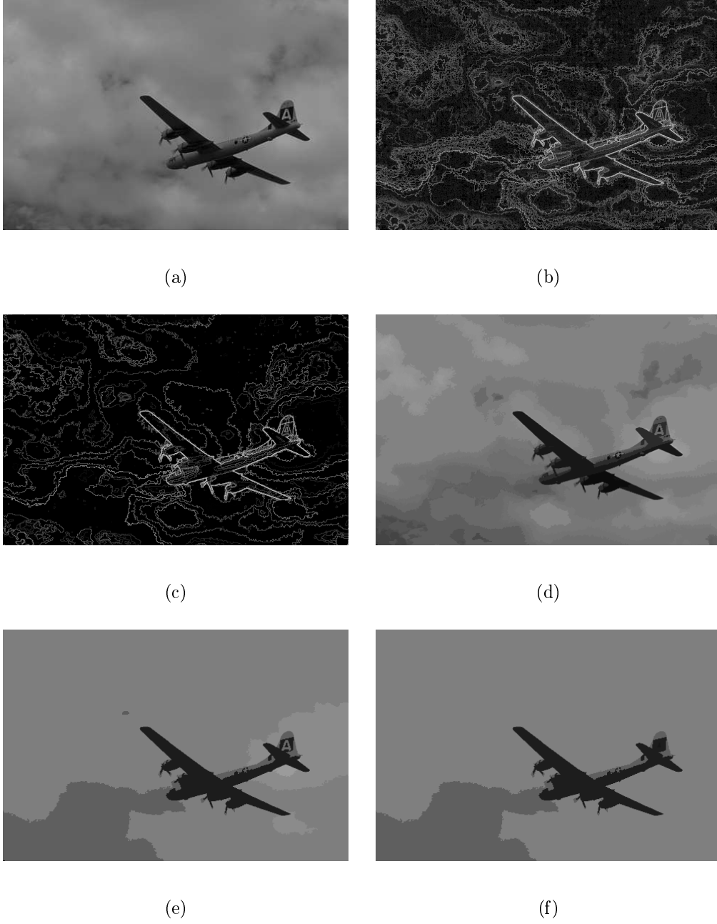
Figure 5.3: Illustration of saliency map representing the hierarchical salient level lines selection using shape meaningfulness increasing order. (a): input image; (b): attribute map defined on boundaries \mathcal{M}_{\mathcal{A}_{\nu}}^{\circ} ; (c): saliency map \mathcal{M}_{\mathcal{E}} representing the hierarchical salient level lines selection. (d-f): a simplified image reconstructed from the level lines obtained by thresholding the saliency map \mathcal{M}_{\mathcal{E}} with respectively small, median, and great threshold value.
