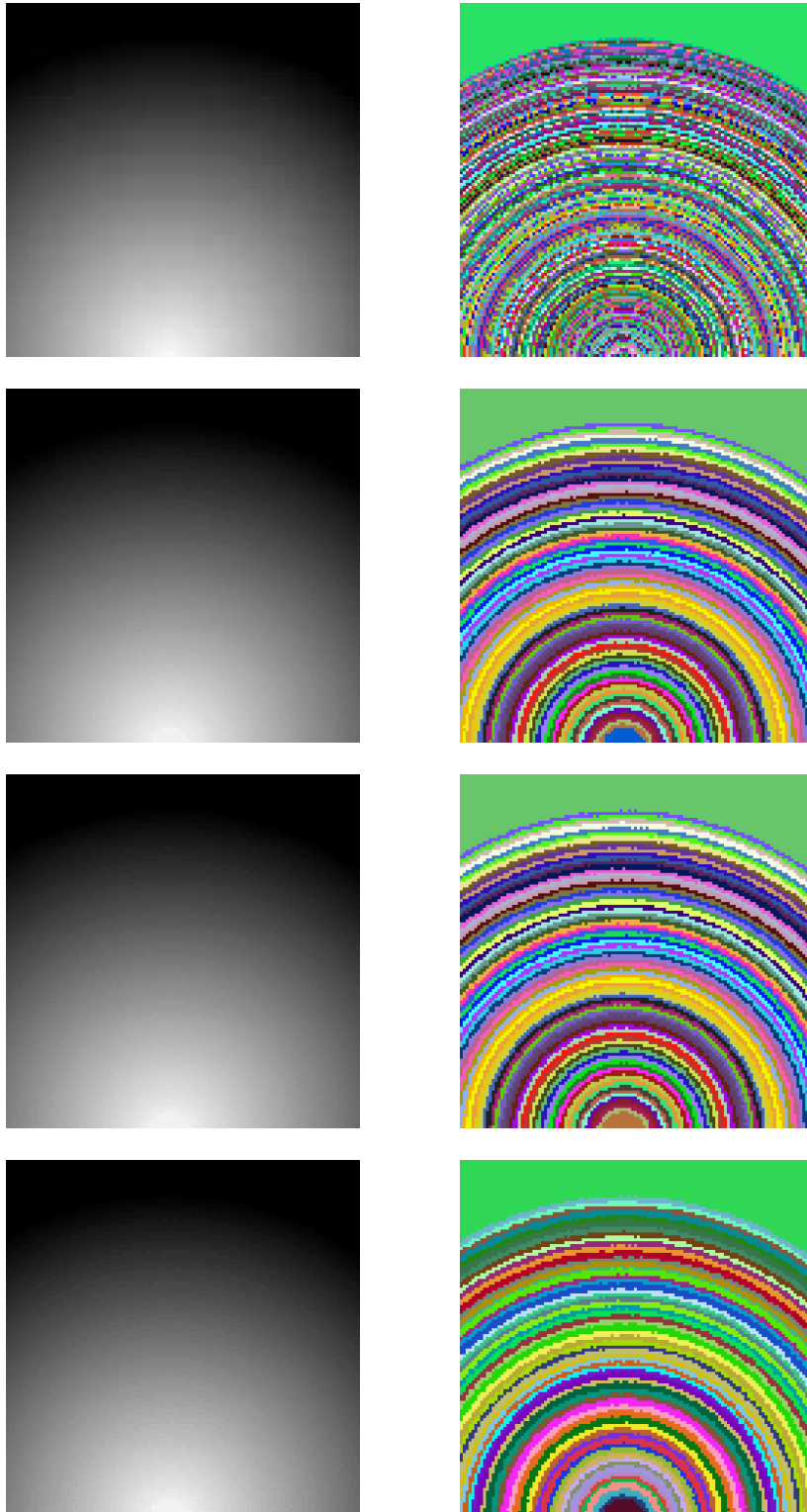
Figure 9.1: Illustration of the disjoint level lines selection with different orders. From top to down: original image, bottom-up, top-down, average of gradient's magnitude decreasing. Left: grayscale image; Right: corresponding randomly colorized image.
