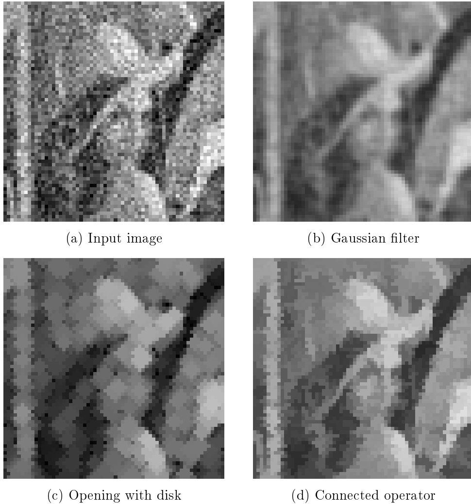
Figure 2.2: A connected operator example compared with a linear filter, and a classical morphological opening with structuring element. The Gaussian filter in (b) blurs image, and the opening using a disk as structuring element in (c) creates new contours. The grain filter [Caselles 2002] does not create any new contour, neither shifts the existing contours.
