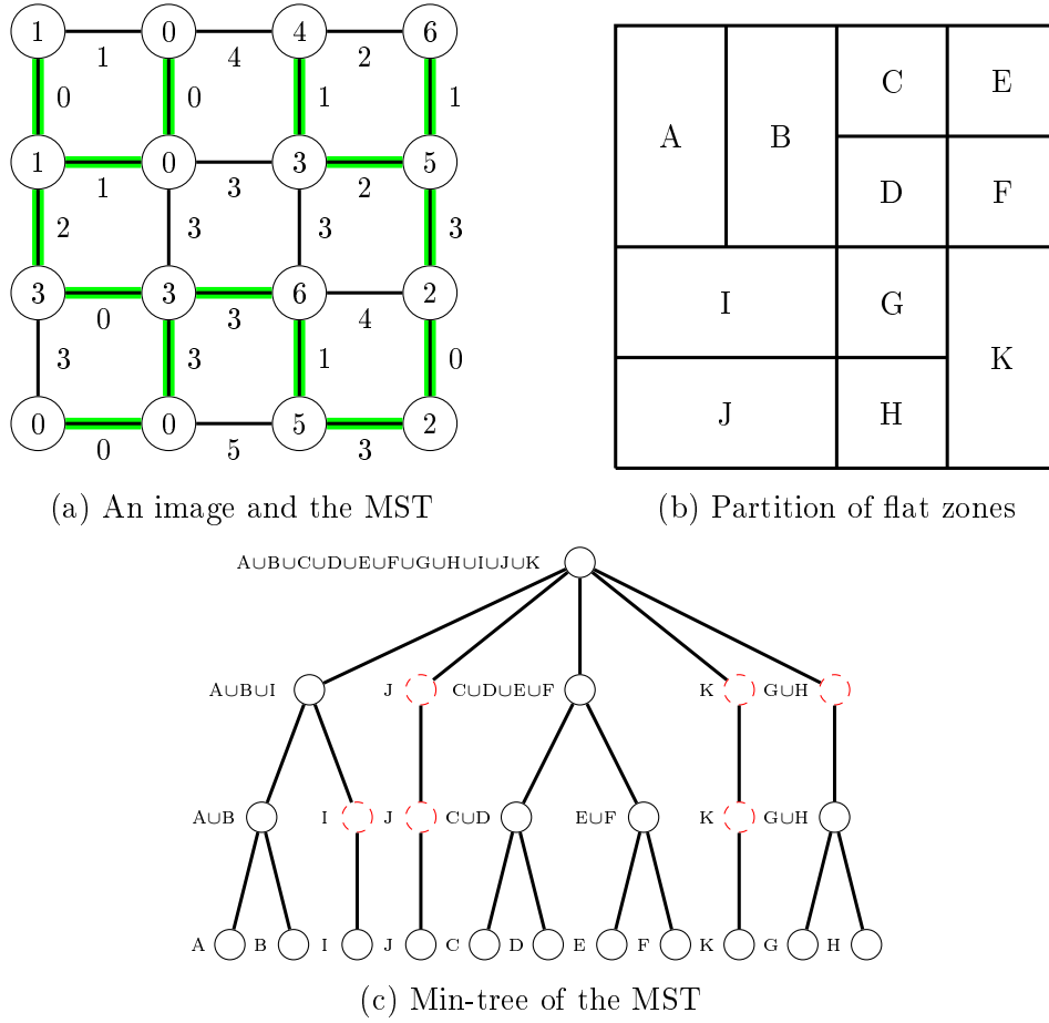
Figure 2.7: An example of the Minimum Spanning Tree (MST). The edges in the MST of image (a) are highlighted in green. The Min-tree of the MST represents a set of partition from fine to coarse, which is equivalent to the \alpha -tree.
