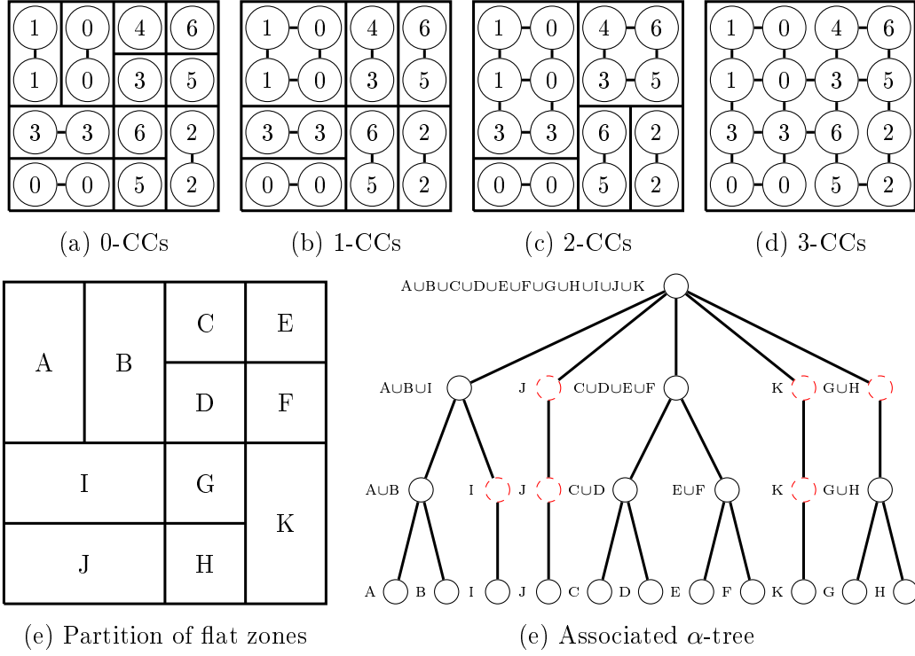
Figure 2.5: A 4×4 image and its partitions into \alpha -connected components for \alpha range from 0 to 3. (a) 0-CCs, (b) 1-CCs, (c) 2-CCs, (d) 3-CCs. Note the fine to coarse partition hierarchies. (e) The associated \alpha -tree that encodes the fine to coarse partition hierarchies. The red dashed circles represent redundant nodes of the tree-based image representation.
