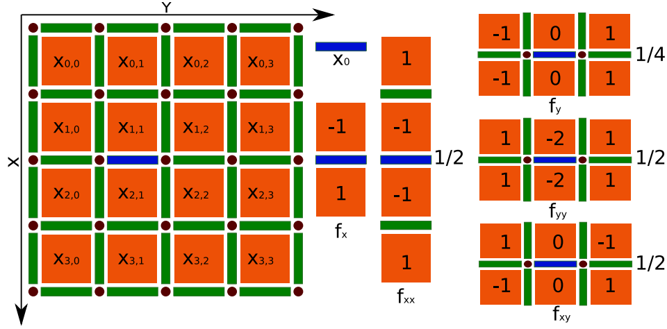
Figure 7.1: Differential operators for the horizontal blue pixel edge. The mask for those differentials in Eq (7.9) is depicted on the right side.
