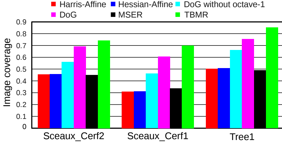
Figure 4.7: Image coverage evaluation by dilating a keypoint with a 2D window having size 31 \times 31 ; Vertical axis represents the average rate of area covered by the dilated region for multi-view images presented in Fig. 4.5, Fig. 4.17, and Fig. 4.18.
