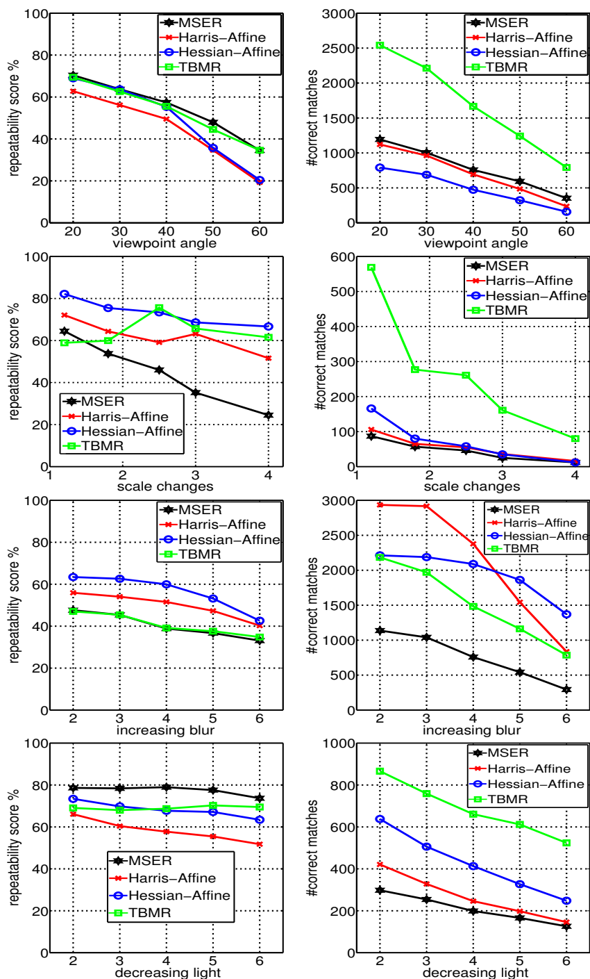
Figure 4.8: Repeatability score (left) and number of correspondences (right) for the sequences Wall , Bark , Trees , Leuven (top to down).
