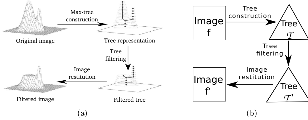
Figure 2.11: An example (a) and a schematic overview (b) of tree-based connected operators implementation [Salembier 1998, Salembier 2000]. In (a), the tree filtering strategy is a tree pruning process, and for those pixels contained in the pruned nodes, they take the value of the lowest preserved ancestor in the image reconstruction step.
