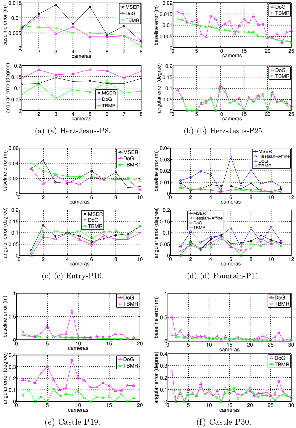
Figure 4.15: Evaluation of camera calibration based on baseline error and angular error applied on the dataset in [Strecha 2008].
