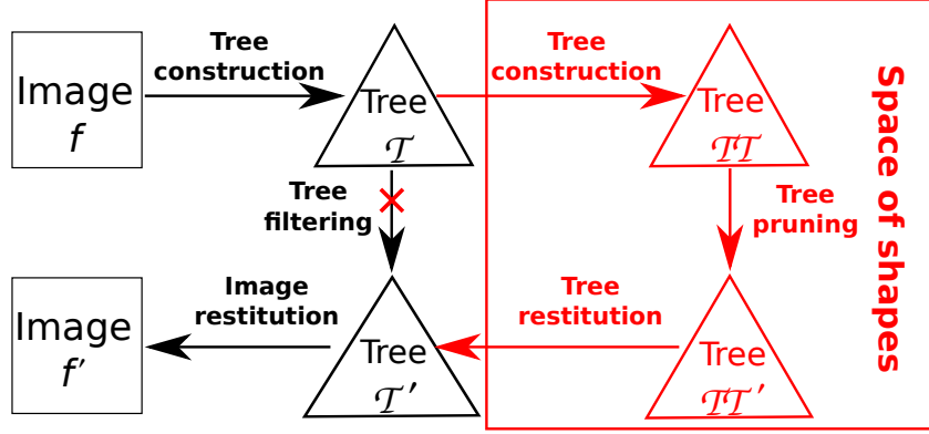
Figure 3.2: Classical connected operators (black path) and our proposed shape-based morphology scheme (black+red path).
