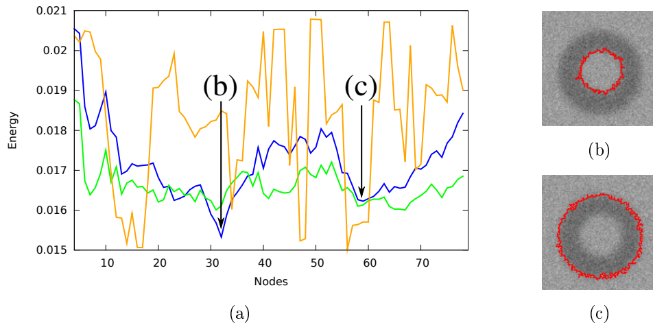
Figure 7.3: Energy estimator on a set of curves of an image, ordered by inclusion; classical snake energy is depicted in green, our proposed energy is in blue, and NFA is in orange. (b) and (c): the curves corresponding to significant energy minima.
