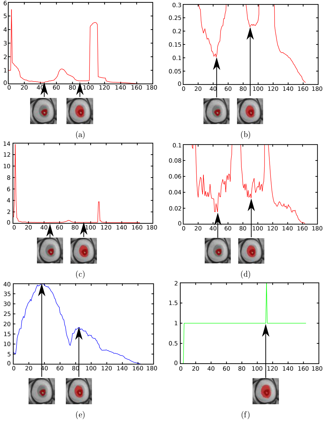
Figure 3.7: Evolution of stability function of Eq (3.2) and average of gradient's magnitude en Eq (3.8) of a branch starting from a leaf node (left side of Axis X) to the root node (right side of Axis X). Axis Y represents the value of corresponding attribute function. The images on the bottom of each figure represents the corresponding regions represented by the nodes at the corresponding locations in the shape space. (a-b) Normal and zoomed stability function with \Delta = 10 ; (c-d) Normal and zoomed stability function with \Delta = 2 ; (e) Average of gradient's magnitude along the boundaries. (f) Number of children.
