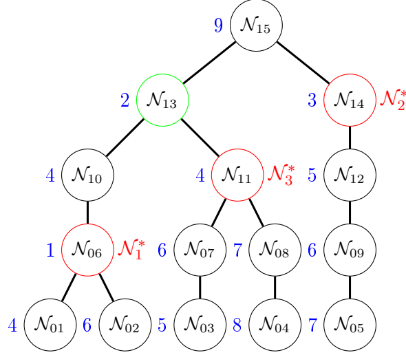
Figure 3.8: Object spotting by repeating the process of selecting the “most likely” node \mathcal{N}_i^* and disabling the ancestors and descendants of node \mathcal{N}_i^* . Blue values are corresponding attribute value \mathcal{A}_o . The three nodes represented by red circles are the detected objects, where \mathcal{N}_1^* is firstly spotted, then \mathcal{N}_2^* and \mathcal{N}_3^* . Note that the green node \mathcal{N}_{13} is more meaningful than \mathcal{N}_{11} , but it is not spotted.
