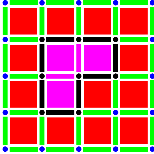
Figure 3.12: Materialization of the points in a 2D image with 0-faces (blue disks), 1-faces (green strips), and 2-faces (red squares). The original points of the image is the 2-faces, the boundaries are materialized with 0-faces and 1-faces. The contour of the purple region is composed of black 1-faces and 0-faces.
