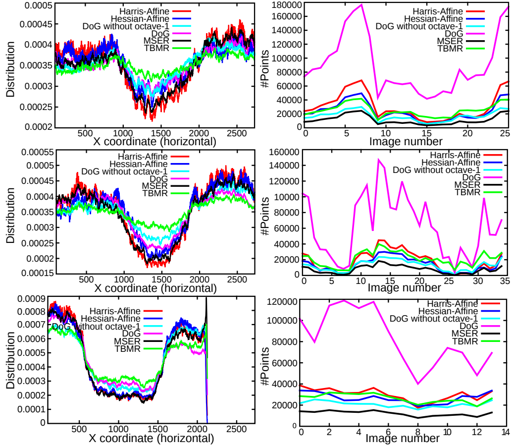
Figure 4.6: Horizontal distribution of the keypoints (left) and number of extracted keypoints (right), for the multi-view images taken around the objects of scene presented in respectively Fig. 4.5, Fig. 4.17, and Fig. 4.18 (top to bottom).
