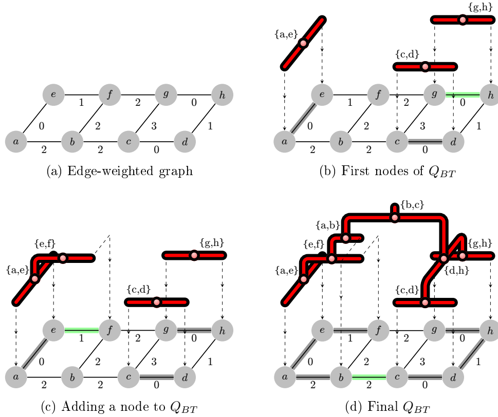
Figure 8.1: A simple process for obtaining Q_{BT} [Najman 2013], a binary tree providing a strict total order relation on the edges of the MST.
