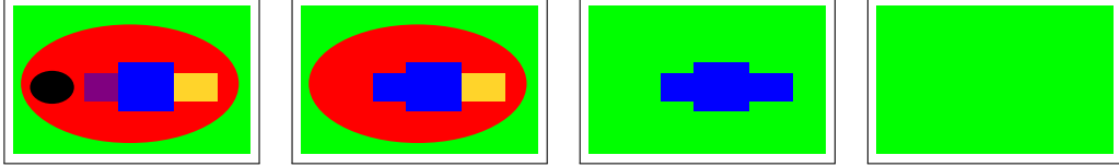
(a) Several levels of a thresholding decomposition based tree (e.g., Min-tree).
