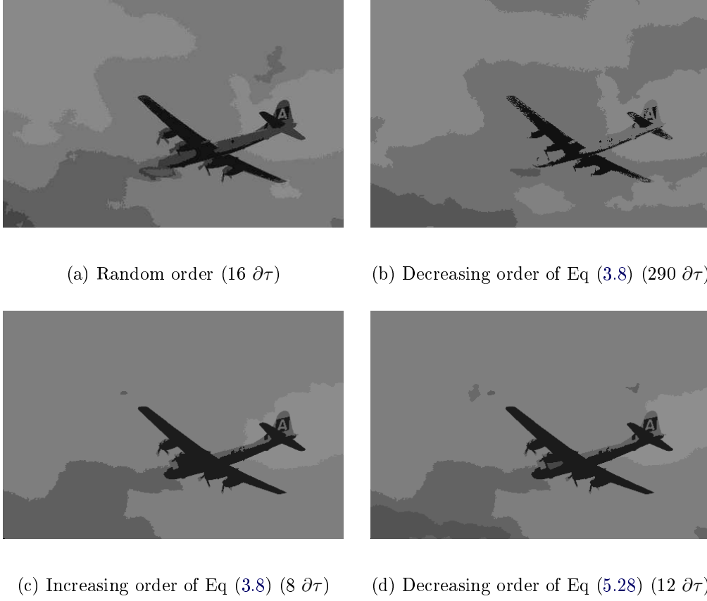
Figure 5.4: Comparison of the proposed greedy algorithm using different orders of the level lines. The parameter \nu is set to \nu = 1000 .
