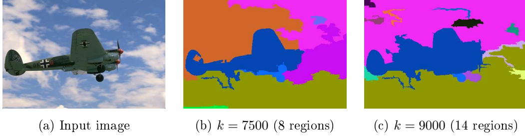
Figure 8.2: An example illustrating the violation of the causality principle by [Felzenszwalb 2004]: the number of regions (in parentheses) increases from 8 to 14, instead of decreasing when the parameter k increases.
