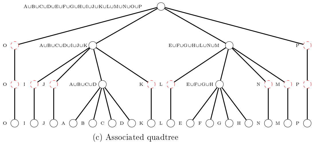
Figure 2.6: An example of quadtree. The homogeneous criterion \mathcal{C} is that the global range \omega \leq 3 .
