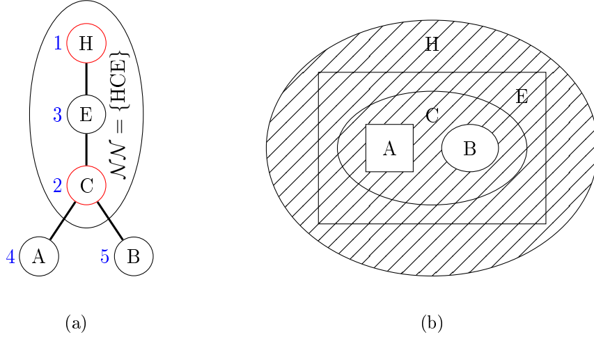
Figure 3.4: Illustration of second attribute \mathcal{AA} being the total variation inside the region given by the union of element “region” of shapes contained in a node \mathcal{NN} . (a) A branch of the tree in Figure 3.3, the nodes inside the ellipse form the node \mathcal{NN} = \{HCE\} in the second tree \mathcal{TT} . (b) The underlying region of image represented by the branch of tree \mathcal{T} in (a), the total variation inside the region covered with oblique lines correspond to \mathcal{AA}(\mathcal{NN}) .
