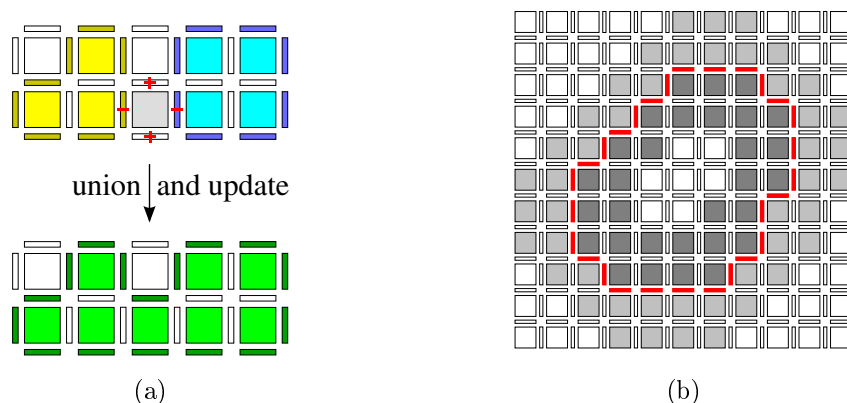
Figure 7.2: (a): Updating contour information when a union between two components (yellow and blue) occurs thanks to a pixel (gray). (b): Regional context of a level line (red) is the inner (dark gray) and outer (light gray) regions.
