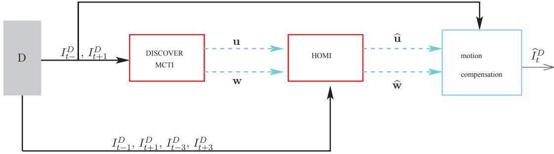
Figure 5.10: ZD-ZH method: the frames I_{t-1}^D, I_{t+1}^D, I_{t-3}^D, I_{t+3}^D are used for the HOMI algorithm and the MVFs \hat{\mathbf{u}} and \hat{\mathbf{w}} are produced. These two MVFs along with I_{t-1}^D and I_{t+1}^D are used for the construction of \hat{I}_t^D .
