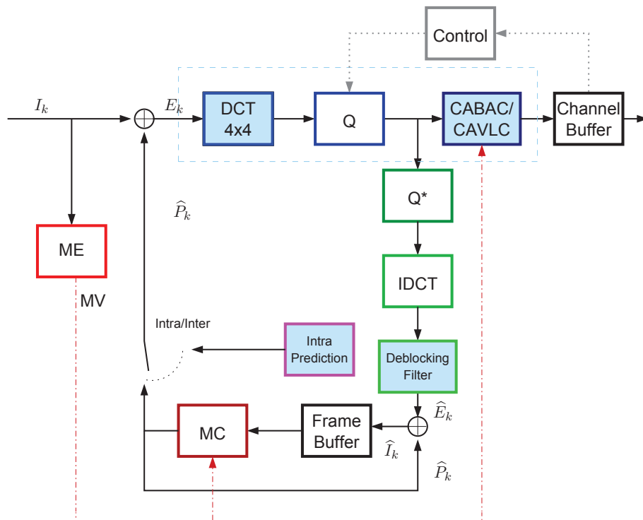
Figure 1.8: H.264/AVC Codec.
