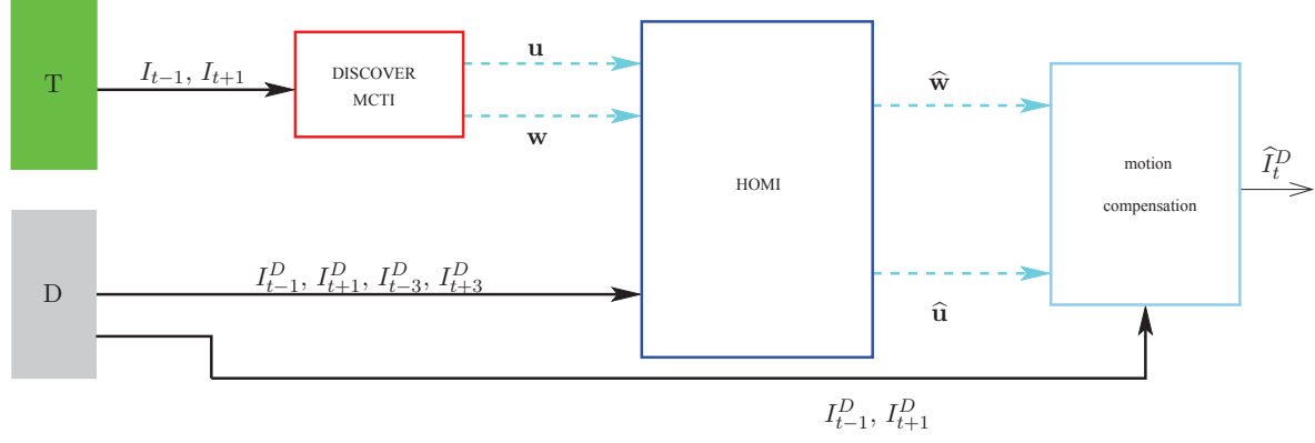
Figure 5.13: TD-ZH method: the frames I_{t-1}, I_{t+1} are used for the DISCOVER MCTI algorithm. The vectors \mathbf{u} and \mathbf{w} are obtained. These vectors are refined by HOMI algorithm implemented on I_{t-1}^D, I_{t+1}^D, I_{t-3}^D, I_{t+3}^D . The produced MVFs \hat{\mathbf{u}} and \hat{\mathbf{w}} are applied to I_{t-1}^D and I_{t+1}^D for producing the SI \hat{I}_t^D
