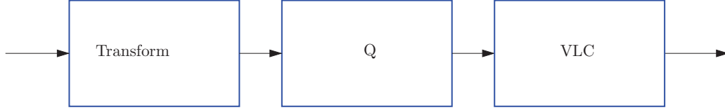
Figure 1.1: Transform coding.
