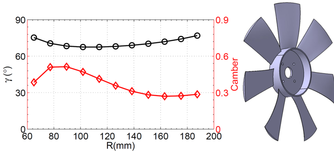
Figure 2.4: Radial profiles of the stagger angle ( \circ ) and of the aerodynamic camber ( \diamond , see Ref. [41] for a definition) for the Rear Rotor of JW1.
