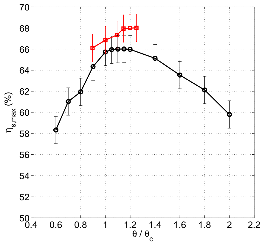
Figure 3.30: Maximum static efficiency vs. \theta . Stage JW1, at N_{FR} = 1400 rpm ( \circ ), N_{FR} = 2300 rpm ( \square ), S = 10 mm.
