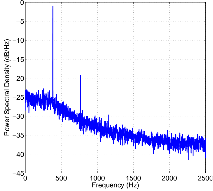
Figure 3.4: Power Spectrum Density of the fluctuations in tangential velocity V_\theta at R = 125 mm (49% of blade height) near the inlet of JW1 (Position Z_p = -46 mm), at design point Q_v = 1 \text{ m}^3 \cdot \text{s}^{-1} , \theta = \theta_C
