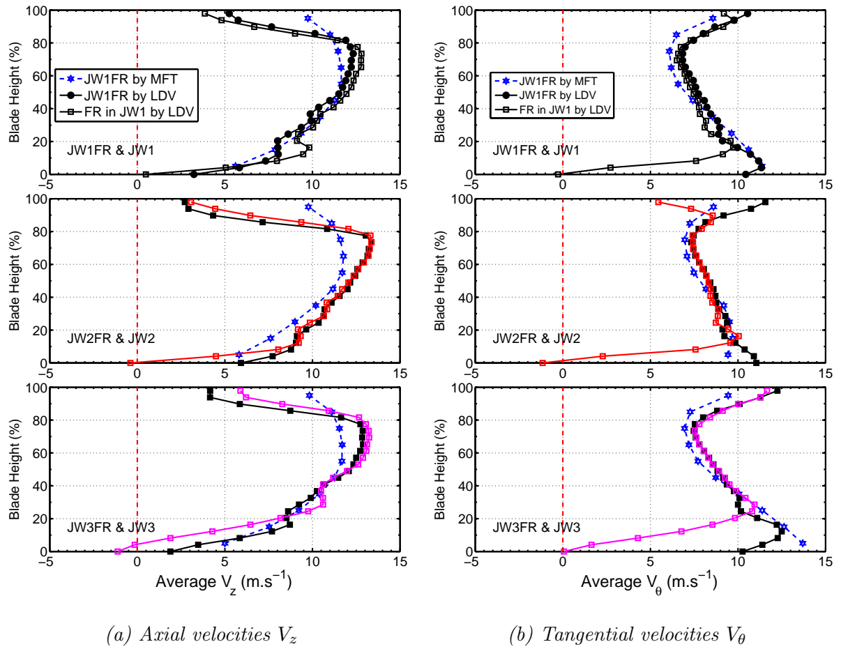
Figure C.16: Averaged axial V_z and tangential V_\theta velocities near the outlet of the FR (Position Z_p = 5\text{mm} ) at design point Q_v = 1\text{m}^3.\text{s}^{-1} , \theta = \theta_C , in: FR alone analyzed by MFT( \star ); FR alone measured by LDV(closed symbols); in CRS measured by LDV(open symbols)
