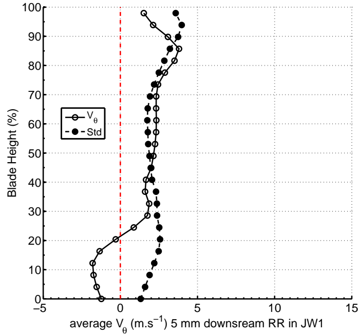
Figure 3.7: Averaged tangential velocity V_\theta ( \circ ) by LDV and its STD ( \bullet ) at the outlet of stage JW1 (Position Z_p = 50\text{mm} ) at design point Q_v = 1\text{m}^3.\text{s}^{-1} , \theta = \theta_C
