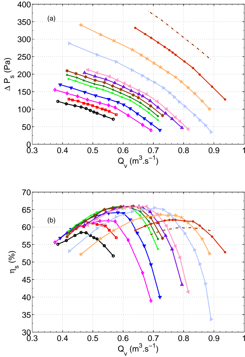
Figure 3.29: Global performance of Stage JW1, at N_{FR} = 1400 \text{ rpm} \theta/\theta_C = 0.6(\circ) , 0.7(\square) , 0.8(\diamond) , 0.9(\nabla) , 1(\times) , 1.05(+) , 1.1(\star) , 1.15(\triangle) , 1.2(\triangleleft) , 1.4(\triangleright) , 1.6(\star) , 1.8(\star) and 2(\cdot) , S = 10 \text{ mm} .
