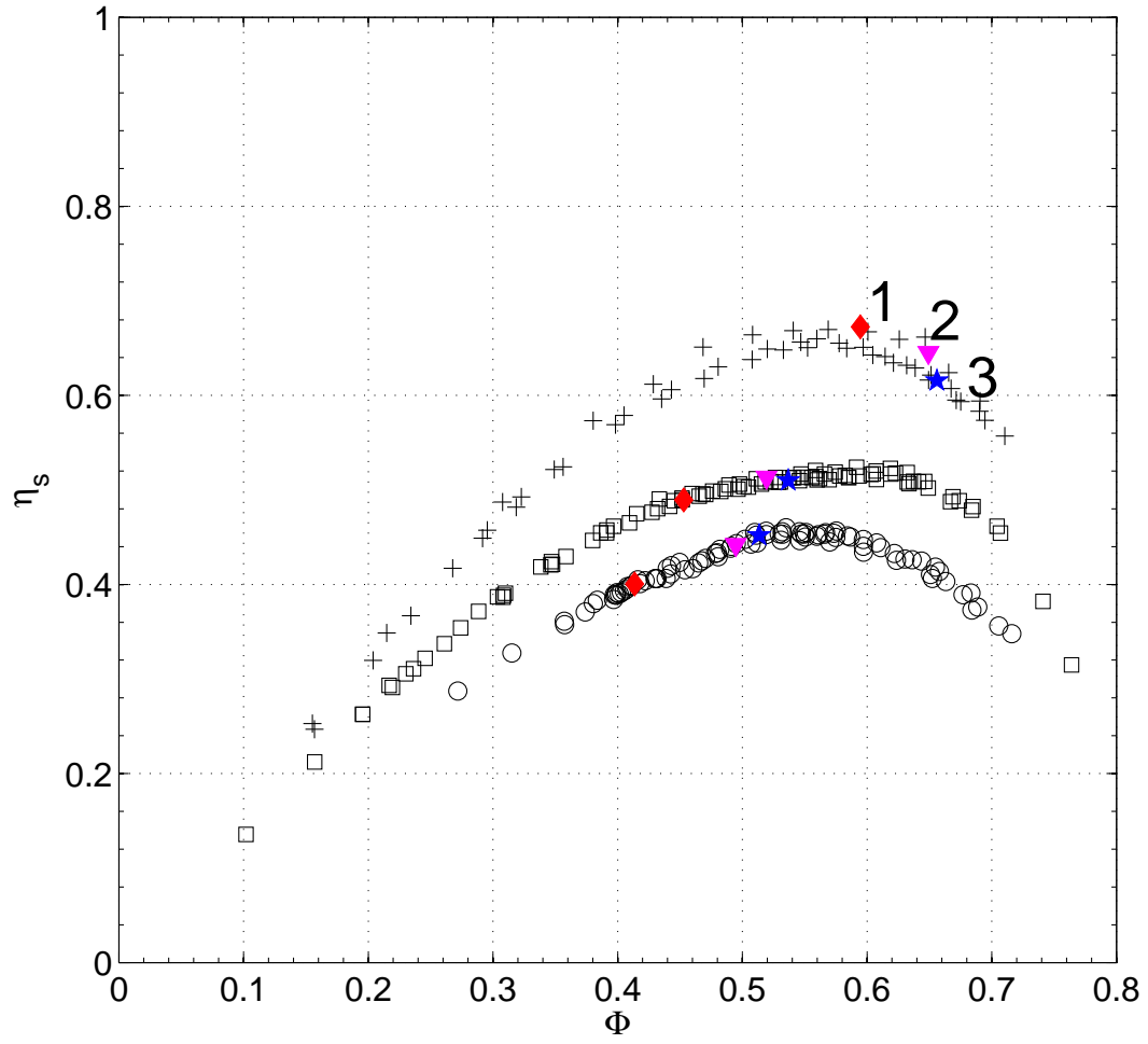
Figure B.1: Static efficiency \eta_s vs. flow coefficient \phi , for the three systems: R1 ( \circ ), RSS at s = 15 mm ( \square ) and CRS at s = 10 mm and \theta = 1 ( + ). Crosspoint 1( \blacklozenge ), Crosspoint 2( \blacktriangledown ), Crosspoint 3( \star )
