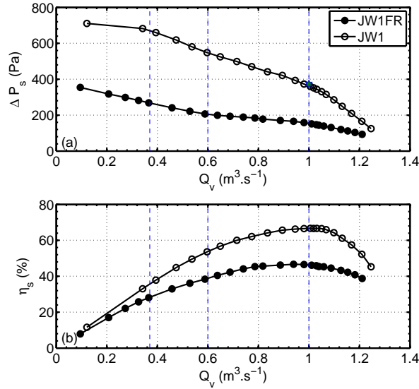
Figure C.3: Overall performance of the JW1FR (●), JW1 (○) and the design point (★) (a): Static pressure rise \Delta P_s vs. volumetric flow rate Q_v ( \Delta P_s is corrected by \rho_{ref} ). (b): Static efficiency \eta_s vs. volumetric flow rate Q_v , at S = 10 mm.
