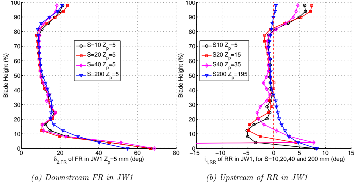
Figure 3.21: Flow angles between FR and RR in JW1 at various S at design point Q_v = 1 \text{ m}^3 \cdot \text{s}^{-1} , \theta = \theta_C . (a) downstream of FR Z_p = 5 \text{ mm} , S = 10, 20, 40, 200 \text{ mm} ; (b) upstream of RR at Z_p = 5 ( S = 10 ), Z_p = 15 ( S = 20 ), Z_p = 35 ( S = 40 ) and Z_p = 195 ( S = 200 ) \text{mm}
