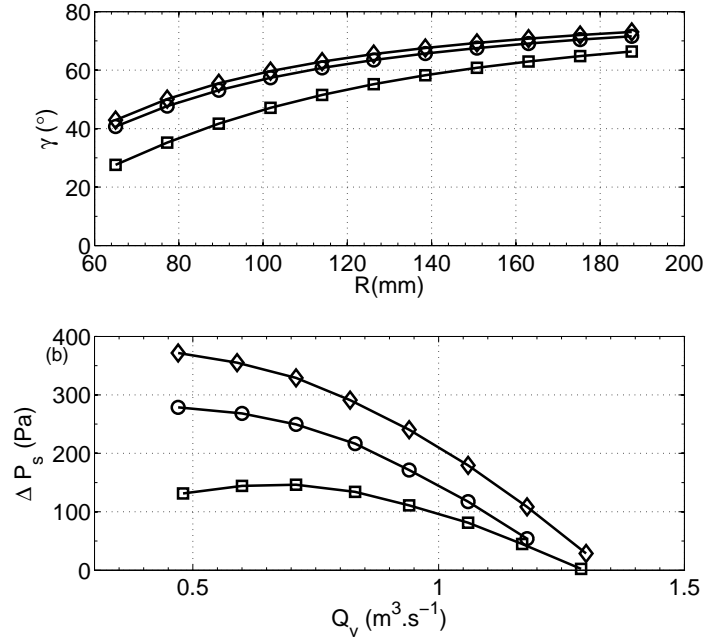
Figure 2.3: Conception by MFT [39], Front Rotor of JW1 ( \circ ); JW2 ( \square ) and JW3( \diamond ). (a): radial profile of the stagger angle and (b): static pressure rise calculated by a semi-empirical model [39].
