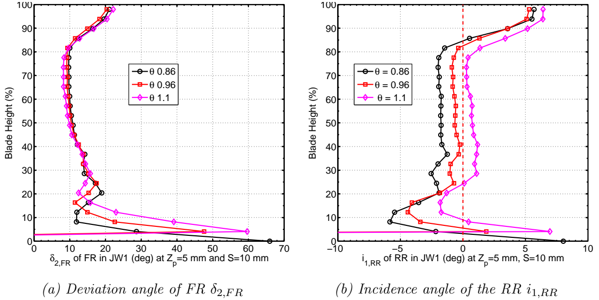
Figure 3.26: Calculated flow angles downstream FR (between FR and RR) in JW1 at Z_p = 5 mm, for \theta = 0.86(0.9\theta_C) , 0.96(\theta_C) , 1.1(1.15\theta_C) , at design point Q_v = 1\text{m}^3.\text{s}^{-1} , S = 10 mm. (a) deviation angle of FR; (b) incidence angle of RR
