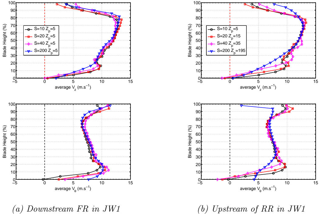
Figure C.11: Circumferential averaged velocity fields between FR and RR in JW1 at various S at design point Q_v = 1 \text{ m}^3 \cdot \text{s}^{-1} , \theta = \theta_C . (a) downstream of FR Z_p = 5 mm, S = 10, 20, 40, 200 mm; (b) upstream of RR at Z_p = 5 ( S = 10 ), Z_p = 15 ( S = 20 ), Z_p = 35 ( S = 40 ) and Z_p = 195 ( S = 200 ) mm
