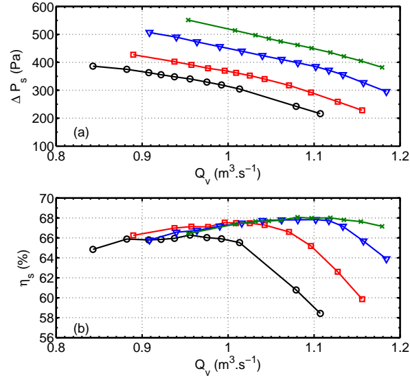
Figure C.12: Overall performance of stage JW1 at Q_v = 1 \text{ m}^3 \cdot \text{s}^{-1} , S = 10 \text{ mm} , N_{FR} = 2300 \text{ rpm} , \theta = [0.86 \text{ (} 0.9\theta_C \text{ } \circ), 0.96 \text{ (} 1.0\theta_C \text{ } \square), 1.1 \text{ (} 1.15\theta_C \text{ } \nabla), 1.2 \text{ (} 1.25\theta_C \text{ } \times)] , \theta_C = 0.96 .
