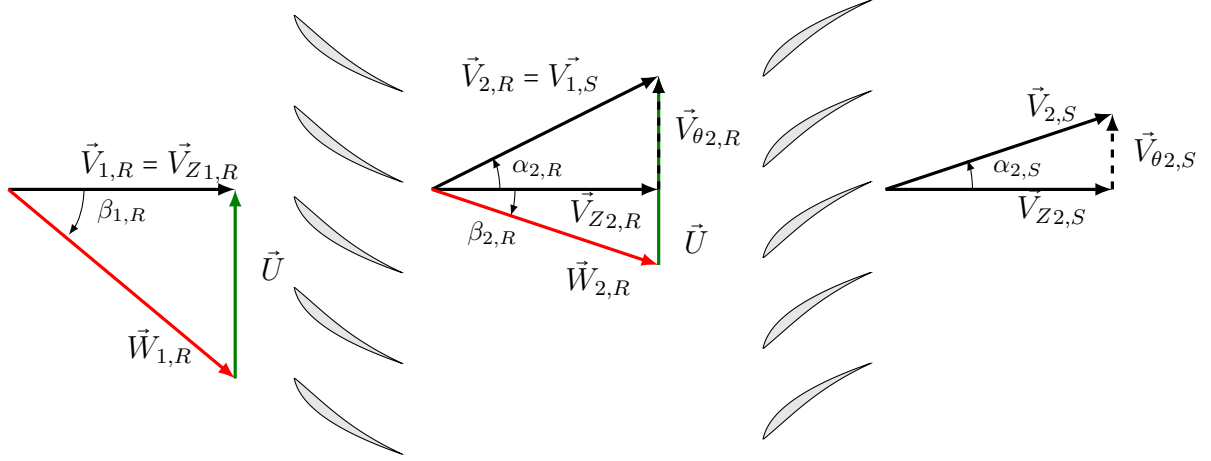
Figure 1.1: Velocity triangles in a compressor/fan: Rotor-Static Stage [5].
