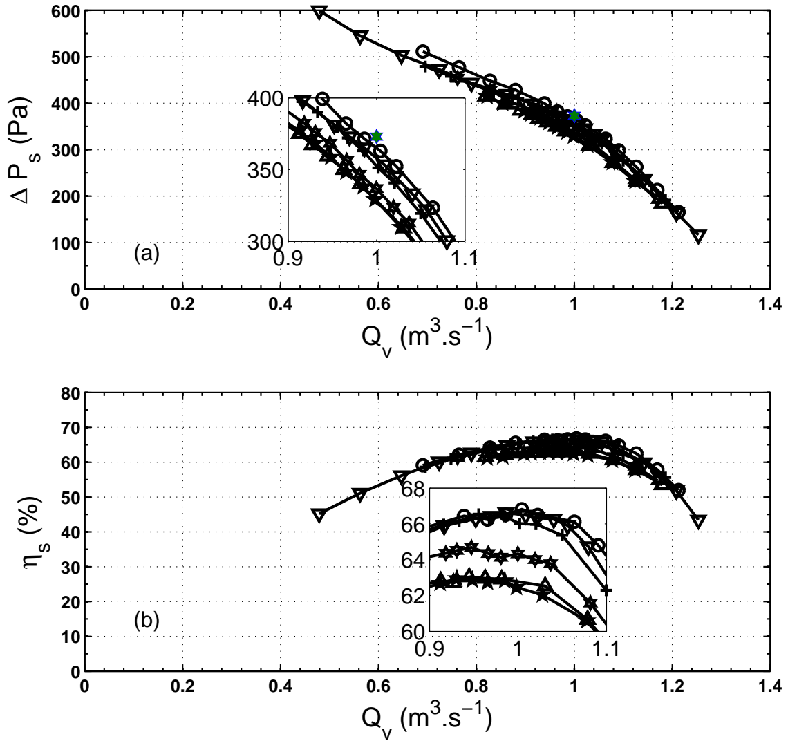
Figure 3.17: Performance S = 10 - 300 \text{ mm} : s = 10(\circ), 50(\nabla), 100(+), 200 (\star), 250(\triangle), 300 \text{ mm}(\star) ; the design point ( \star ), \Delta P_s rescaled by \rho_{ref} .
