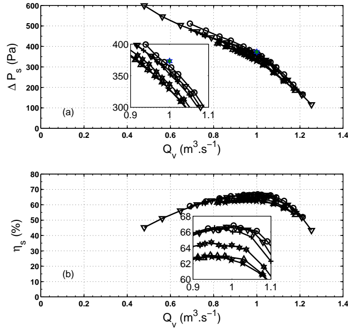
Figure C.10: Performance S = 10 - 300 \text{ mm} : s = 10(\circ), 50(\nabla), 100(+), 200(\star), 250(\triangle), 300 \text{ mm}(\star) ; the design point ( \star ), \Delta P_s rescaled by \rho_{ref} .
