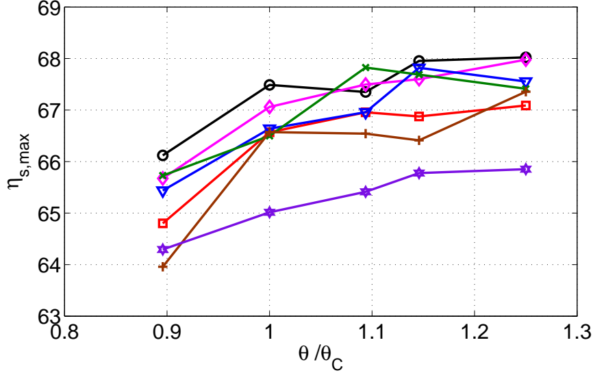
Figure 3.31: Maximum Static efficiency of the stage JW1 at N_{FR} = 2300 rpm, vs. \theta/\theta_C for S = 10 mm ( \circ ), S = 20 mm ( \square ), S = 40 mm ( \diamond ), S = 50 mm ( \nabla ), S = 60 mm ( \times ), S = 100 mm ( + ) and S = 200 mm ( \star ).
