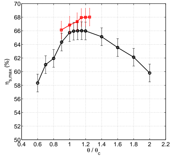
Figure C.14: Maximum static efficiency vs. \theta . Stage JW1, at N_{FR} = 1400 rpm (○), N_{FR} = 2300 rpm (◻), S = 10 mm.
