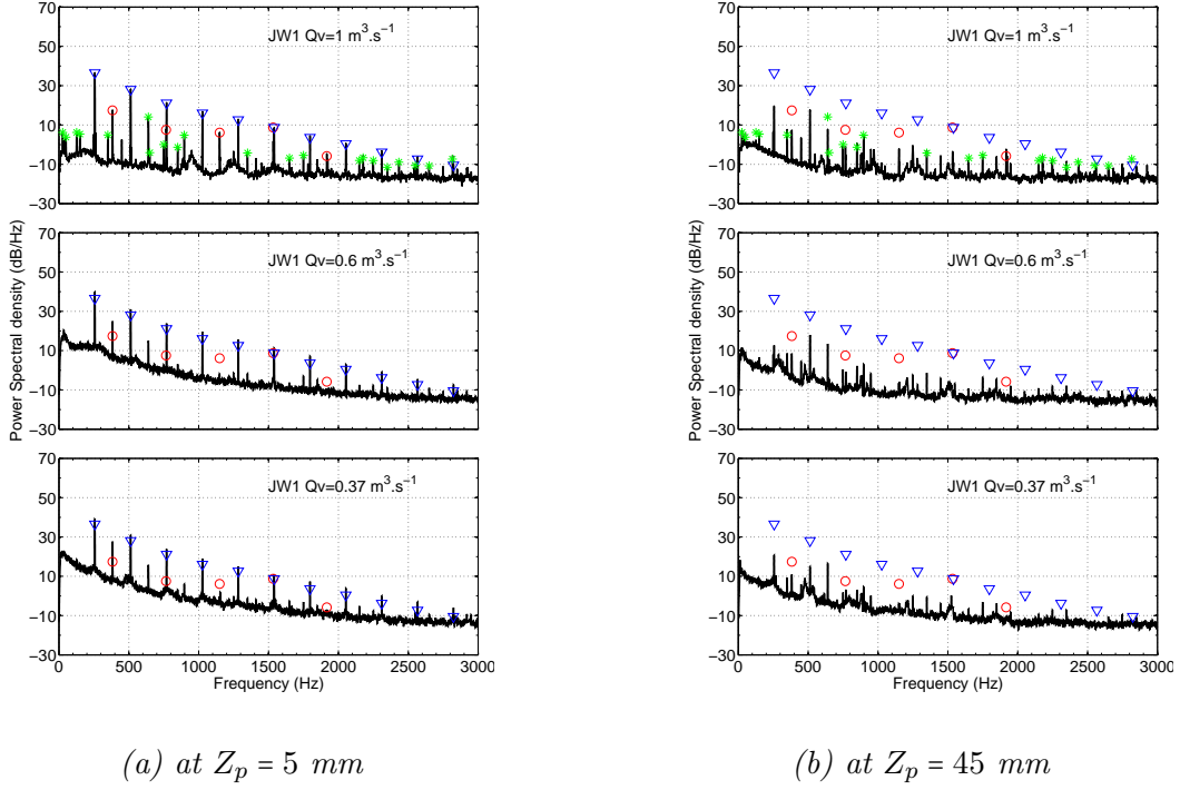
Figure C.9: PSD of the wall pressure fluctuations measured at Z_p = 5 and 45 \text{ mm} , for JW1 at N = 2300 - 2200 \text{ rpm} and S = 10 \text{ mm} , Q_v = 1, 0.6 and 0.37 \text{ m}^3.\text{s}^{-1} . (○): m f_{bpf,FR} ; (▽): n f_{bpf,RR} ; and (*): m f_{bpf,FR} + n f_{bpf,RR} with m \neq 0 and n \neq 0 .
