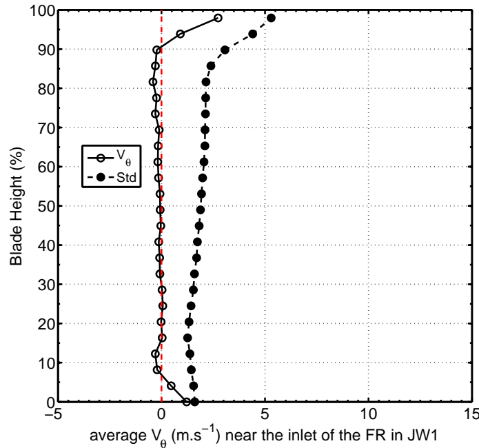
Figure 3.3: Averaged tangential velocity V_\theta ( \circ ) by LDV and the their Standard Deviation ( \bullet ) at the inlet of JW1 (Position Z_p = -46 mm) at design point Q_v = 1 m 3 .s -1 , \theta = \theta_C
