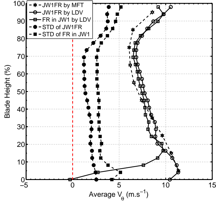
Figure 3.6: Averaged axial velocity V_\theta near the outlet of the Front Rotor (Position Z_p = 5\text{mm} ) at the design point Q_v = 1\text{m}^3.\text{s}^{-1} , \theta = \theta_C , In: JW1FR analyzed by MFT( \star ); JW1FR measured by LDV( \circ ) and their STD( \bullet ); JW1 measured by LDV( \square ) and their STD( \blacksquare )
