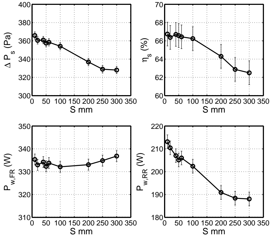
Figure 3.19: Performance of JW1 ( \circ ) at S = 10, 20, 40, 50, 60, 100, 200, 250, 300 mm at design point Q_v = 1 \text{ m}^3.\text{s}^{-1} , \theta = \theta_C , \Delta P_s , \mathcal{P}_{w,FR} and \mathcal{P}_{w,RR} are rescaled by \rho_{MFT}
