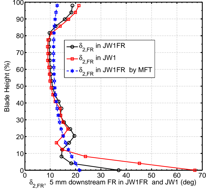
Figure 3.11: Deviation angle \delta_{2,FR} at the outlet of the Front Rotor (Position Z_p = 5\text{mm} ) at design point Q_v = 1\text{m}^3.\text{s}^{-1} , \theta = \theta_C , in : Isolated JW1FR analyzed by MFT( \star ); Isolated JW1FR measured by LDV ( \circ ); JW1 measured by LDV ( \square )
