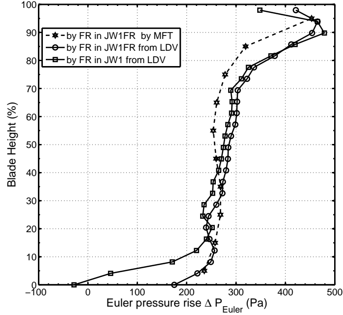
Figure 3.9: Radial profiles of the Euler pressure rise of the FR in JW1FR analyzed by MFT (☆); in JW1FR calculated from LDV measurements (○), and in JW1 calculated from LDV measurements (□), at design point Q_v = 1 \text{ m}^3 \cdot \text{s}^{-1} , \theta = \theta_C , S = 10 \text{ mm}
