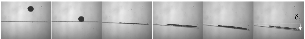
Figure V.7 – Galinstan drop of radius R = 1.25 mm and speed V = 4 m/s hitting the edge of a thin glass plate. Images are separated by 1 ms and only show 1/3 of the lamella. We denote \delta_0 as the maximum plate deflection after impact.
