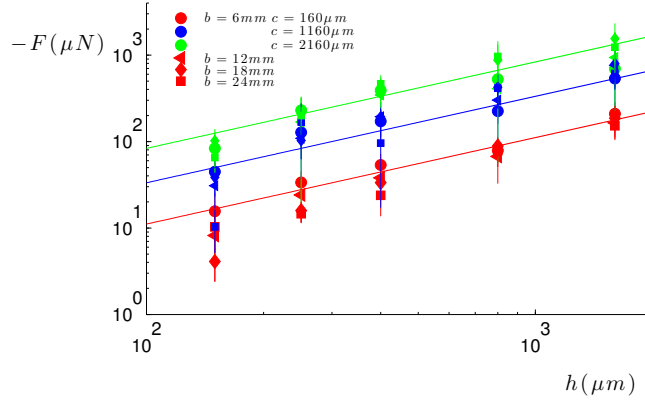
Figure III.17 – Force of propulsion as a function of wall height h . Each color represent a thickness c \in [160, 1160, 2160] \mu\text{m} . Each symbol represent a width b (circles for b = 6 mm, triangles for b = 12 mm, diamonds for b = 18 mm, squares for b = 24 mm). Length a is fixed to 30 mm and \alpha = 45^\circ . For a given plate thickness c (i.e. a given color), each cluster corresponds to a wall height h \in [150, 250, 400, 800, 1600] \mu\text{m} . Compared to previous viscous entrained experiments, the propulsion direction is opposed, hence the negative sign of F . Solid lines show best linear fit, as suggested by equation III.21. Each point is an average of at least 5 measurements.
