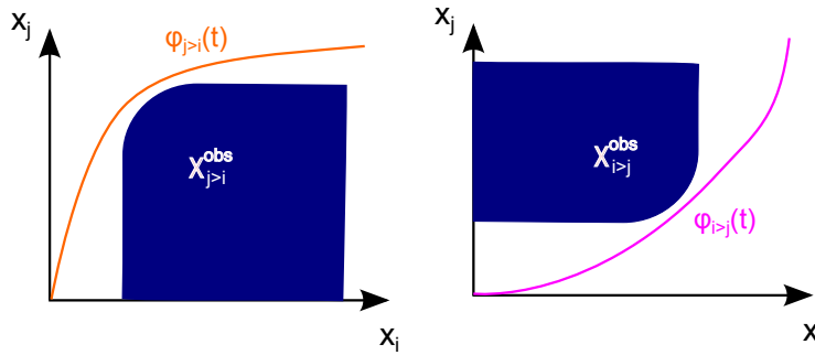
Figure 2.7: Projection of the completed collision cylinders \chi_{i \succ j}^{\text{obs}} and \chi_{j \succ i}^{\text{obs}} .
