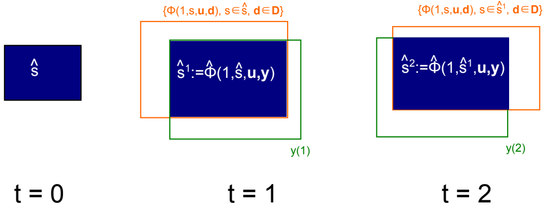
Figure 6.1: Evolution of the non-deterministic information state. For t \in (0, 1) , the "size" of the non-deterministic information state grows until a new observation is available at t = 1 . The intersection with y(1) at t = 1 enables to take into account the new observation and reduces the "size" of the updated non-deterministic information state \hat{s}^1 .
