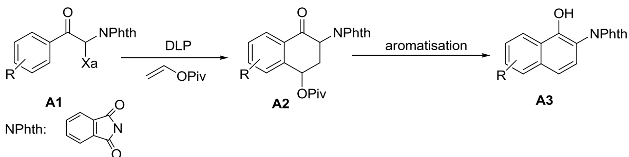
Scheme II-A3
