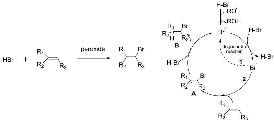
Scheme I-13
