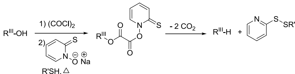
Scheme II-8
