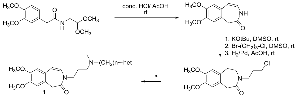
Scheme I-10
