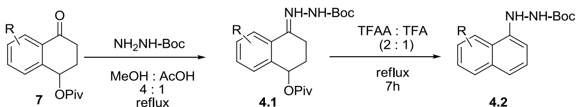
Scheme II-8
