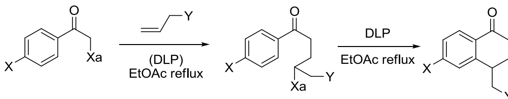
Scheme II-A1
