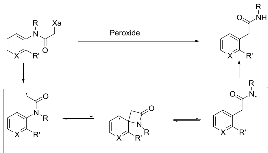
Scheme I-8
