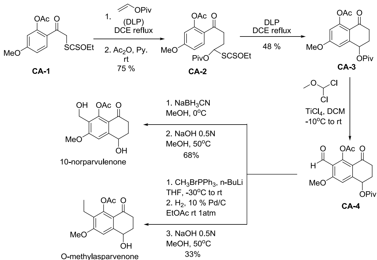
Scheme II-29
