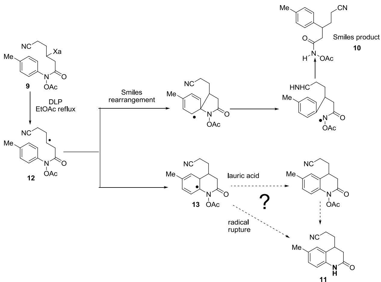
Scheme II-6
