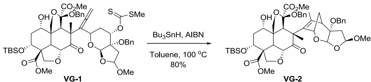
Scheme II-6
