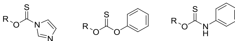
Scheme II-7
