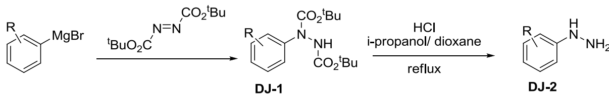
Scheme I-3
