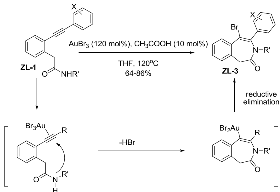
Scheme I-21
