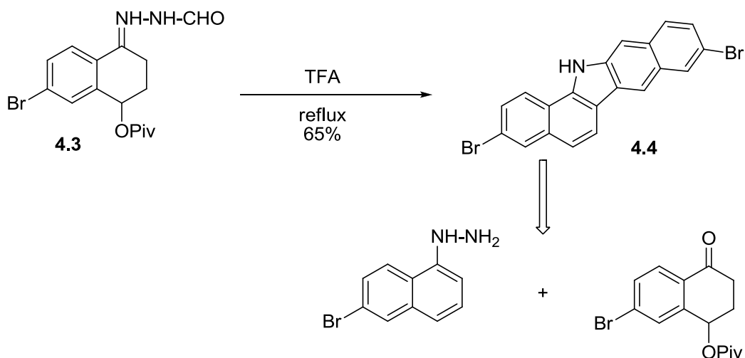
Scheme II-5
