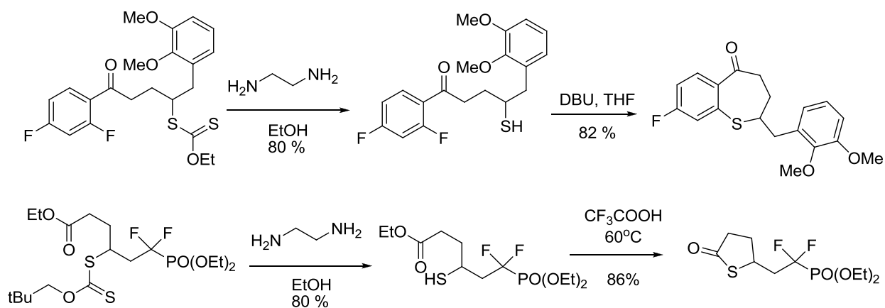
Scheme II-26
