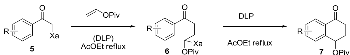
Scheme II-7
