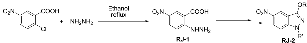
Scheme I-1
