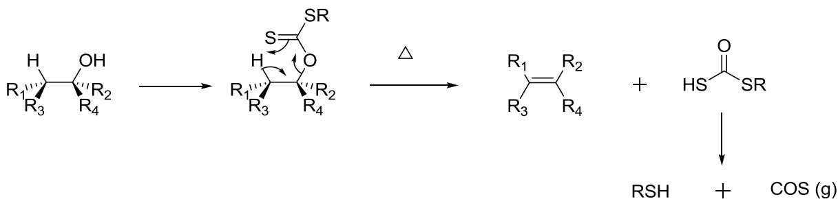
Scheme II-1
