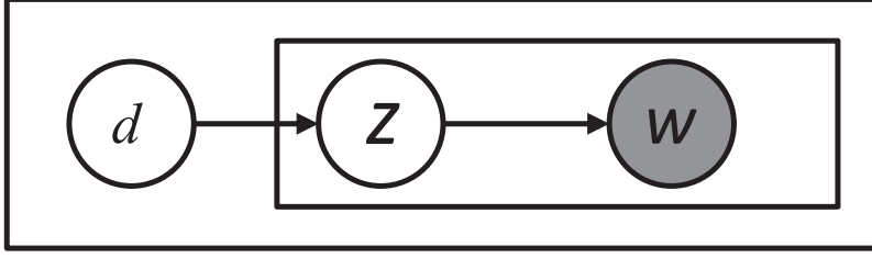
Figure 2.4: pLSA model
