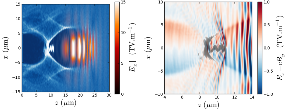
Figure 2.5: Snapshot of the CALDER 3D simulation, after 250 \mu\text{m} of acceleration. Left panel: Representation of the electron density (blue) and the electric field (orange, superimposed with partial transparency). Right panel: Representation of the fields in the vicinity of bunch. The shaded areas correspond to zones of high electron density (here mainly the electron bunch and the back of the sheath).
