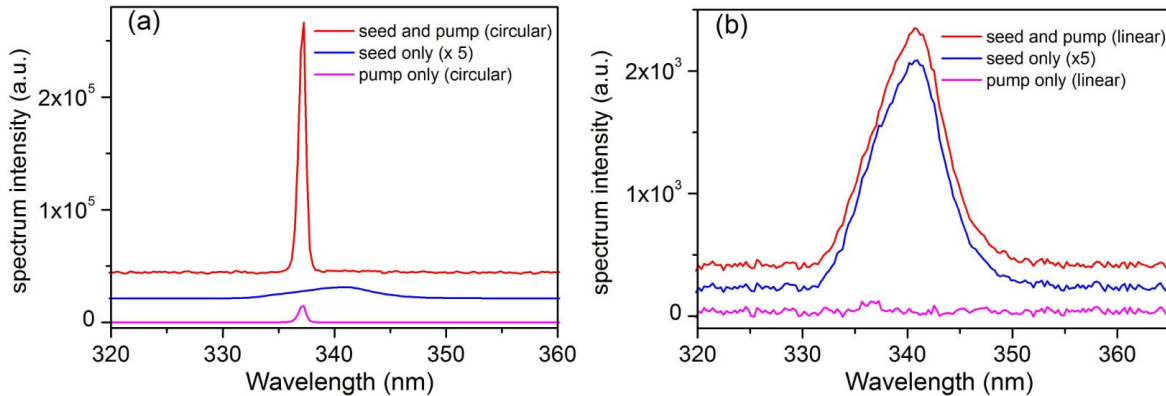
Figure 4.15: Spectra of the backward stimulated emission with circularly (a) and linearly (b) polarized pump pulsed at 800 nm. The spectra of the seed pulses and those of the backward emission from just the pump pulses are also presented for comparison.
