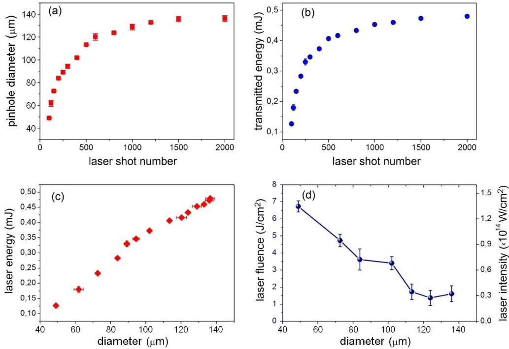
Figure 2.3: (a) and (b), diameter of the micrometric pinholes and the corresponding transmitted laser energy as a function of the laser shot number. (c), Transmitted laser energy as a function of the pinhole diameter. (d), Calculated laser fluence (left scale) and laser intensity (right scale) as a function of the pinhole diameter.
