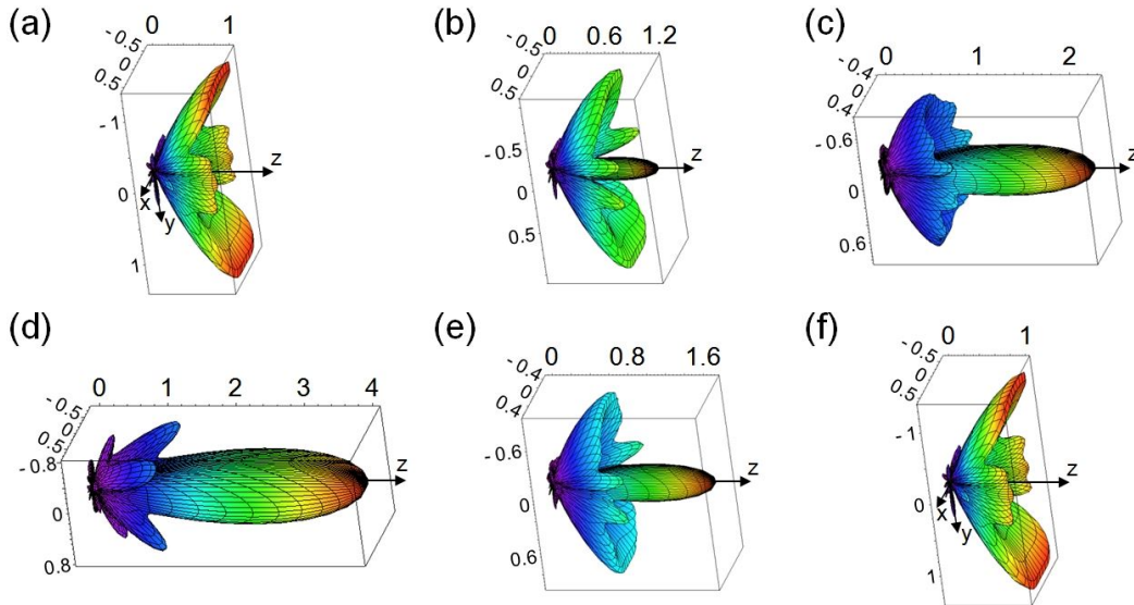
Figure 6.13: Evolution of the 3D emission diagram of the THz radiation from two 'V-oriented' filaments as a function of the temporal delay between the two laser pulses. The angle between the two filaments is 2\alpha = 56^\circ . Values of the temporal delay \tau_p : (a) 0 ps; (b) 2 ps; (c) 3 ps; (d) 5.5 ps; (e) 8.5 ps; (f) 11 ps.
