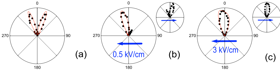
Figure 7.2: Angular dependence of the THz emission from a laser filament in the presence of increasing transverse electric field E_{ext} = 0 kV/cm (a), 0.5 kV/cm (b), and 3 kV/cm (c). The figure is taken from [Houard 08c].
