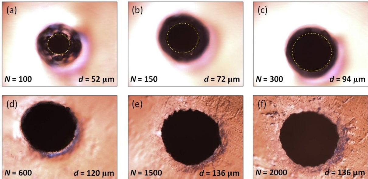
Figure 2.2: The micrometric pinholes created by the laser filament as a function of the number of laser shots. The 1.1 mJ femtosecond laser pulses are focused by a convex f = 1000 mm lens in air.
