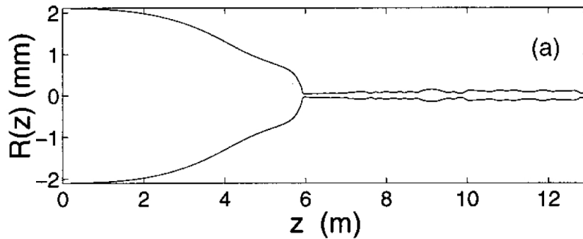
Figure 1.3: Evolution of the laser beam width along the propagation direction (result of computer simulation). The Figure is taken after [Couairon 02b]. The laser pulse is 5 mJ, 50 fs, 800 nm. The laser beam self-collapses on its axis due to the Kerr effect, subsequently the laser intensity becomes high enough to ionize the gas. Therefore, a long filament is formed due to the competition of the Kerr effect and plasma defocusing.
