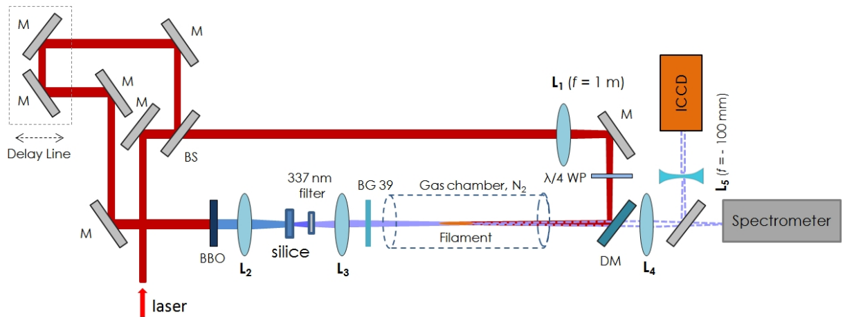
Figure 4.14: Scheme of the experimental setup.
