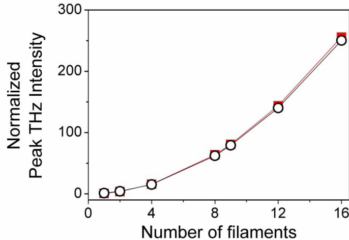
Figure 7.11: Dependence of the peak THz intensity on the number of filaments. Squares – theoretical upper limit (quadratic dependence), Circles – maximum value obtained in our calculations.
