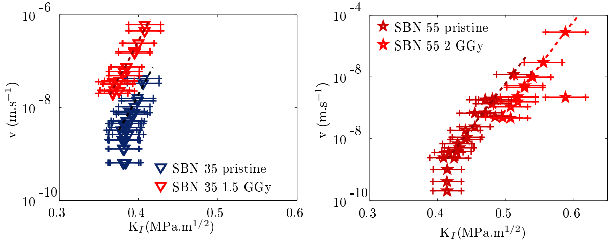
Figure 4.21: Evolution of failure behavior of: (left) SBN 35 pristine (dark blue) and irradiated (red) in stress corrosion regime; (right) SBN 55 pristine (dark red) and irradiated (red).
