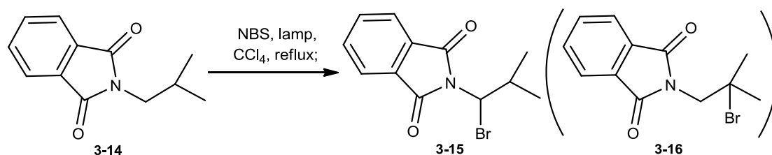
Scheme 3.12 Bromination of 3-14
