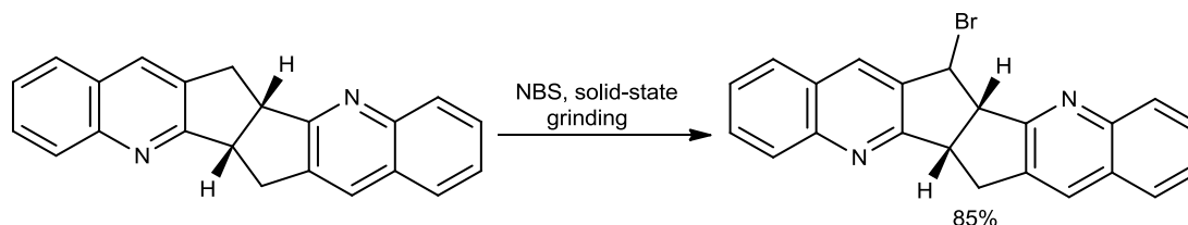
Scheme 3.6 Wohl-Ziegler reaction in the absence of solvent
