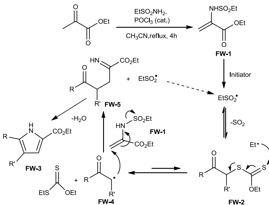
Scheme 5.15
