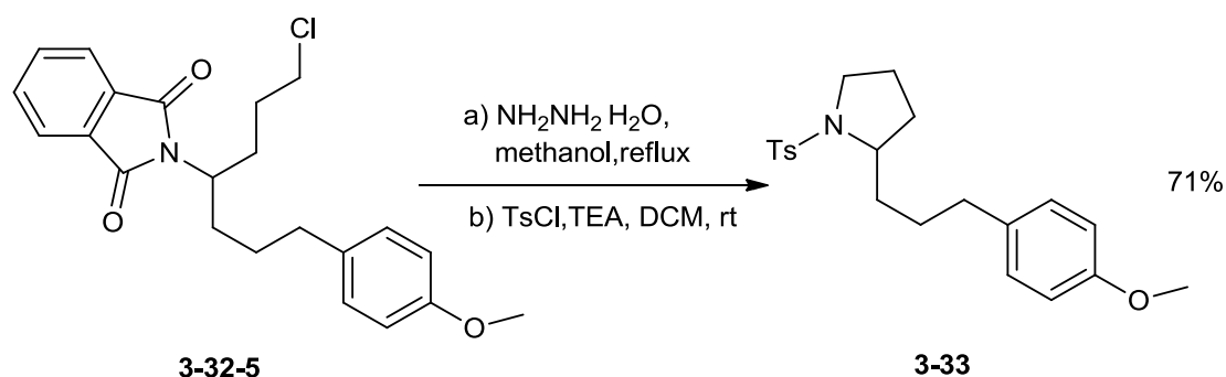
Scheme 3.31 Synthesis of pyrrolidines 3-33
