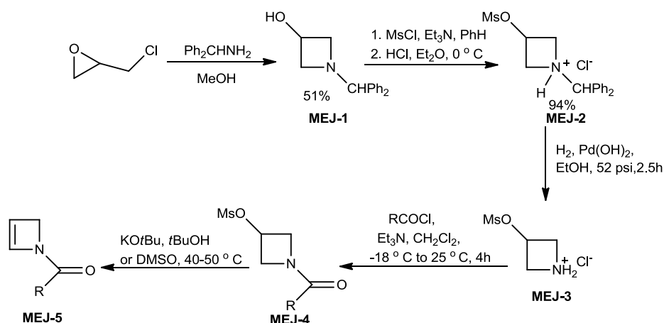
Scheme 5.22 Synthesis of 1-acyl-2-azetidines
