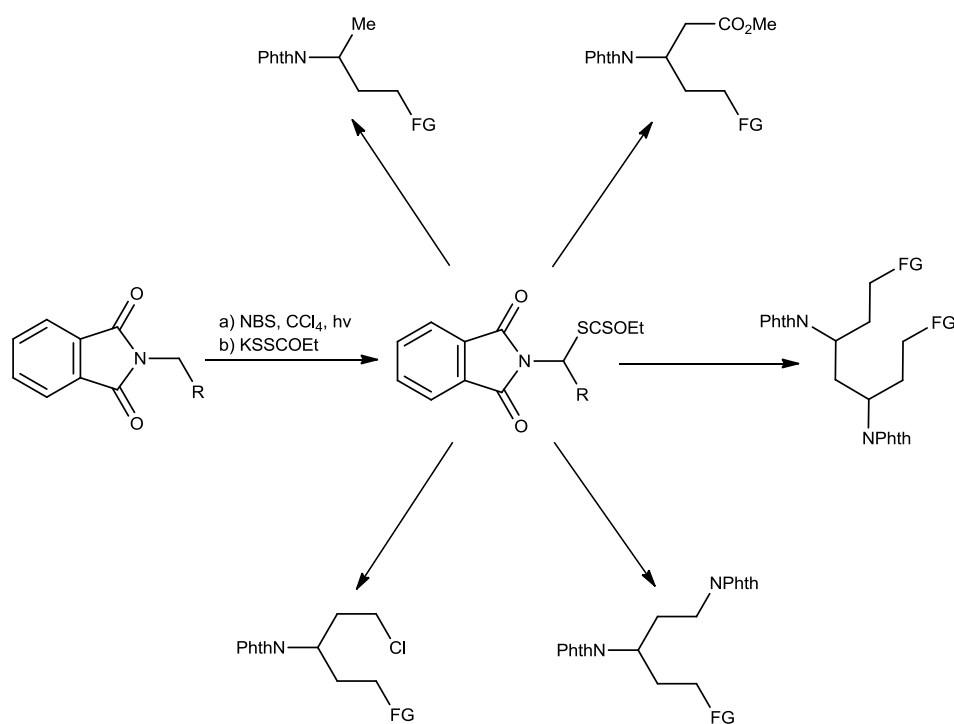
Scheme 3.51
