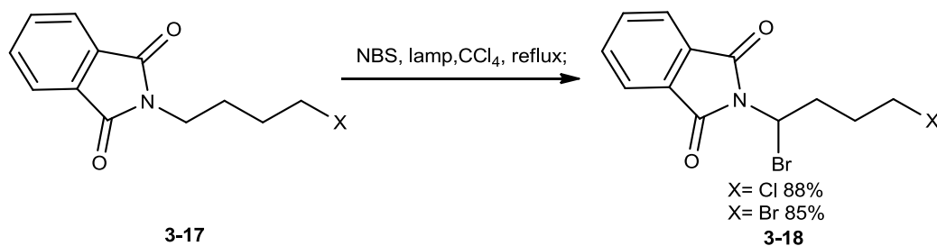
Scheme 3.13 Bromination of 3-17
