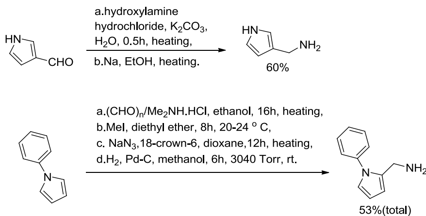
Scheme 5.12 Reductive amination
