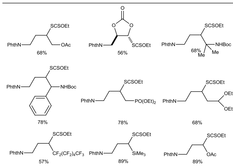
Scheme 2.35 Examples of phthalimidomethyl adducts
