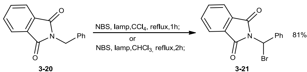
Scheme 3.15 Bromination of 3-20
