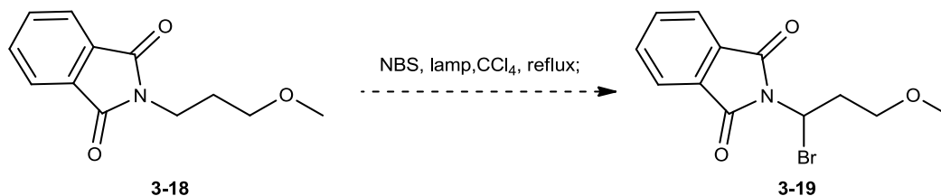
Scheme 3.14 Bromination of 3-18
