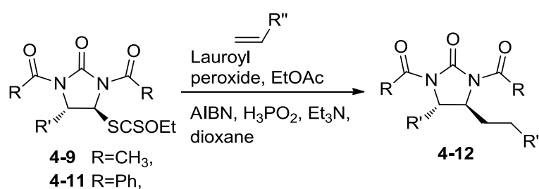
Scheme 4.18 Secondary radical addition
