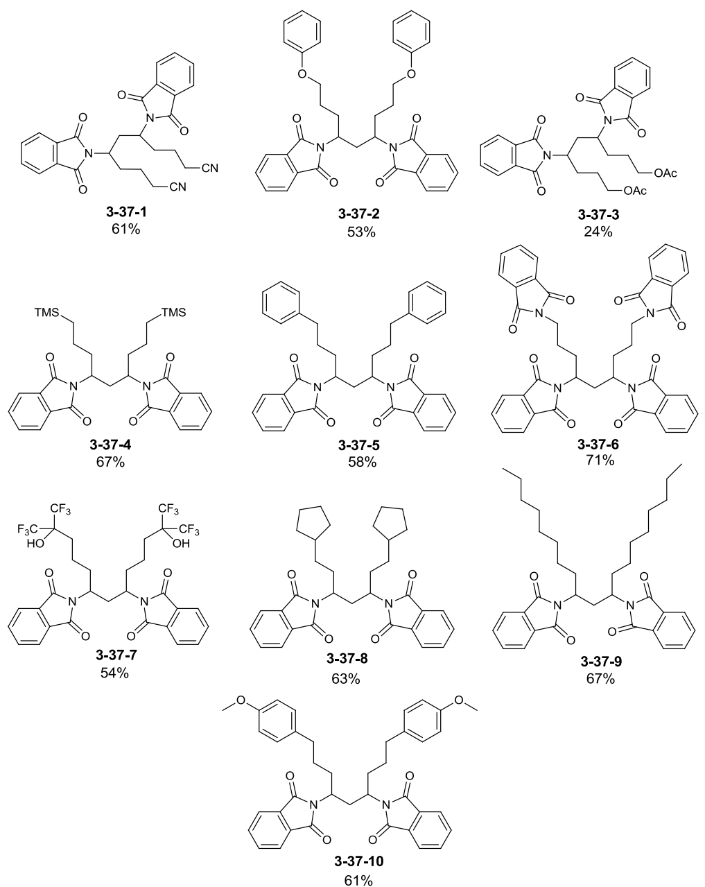
Scheme 3.39 Examples of 3-37
