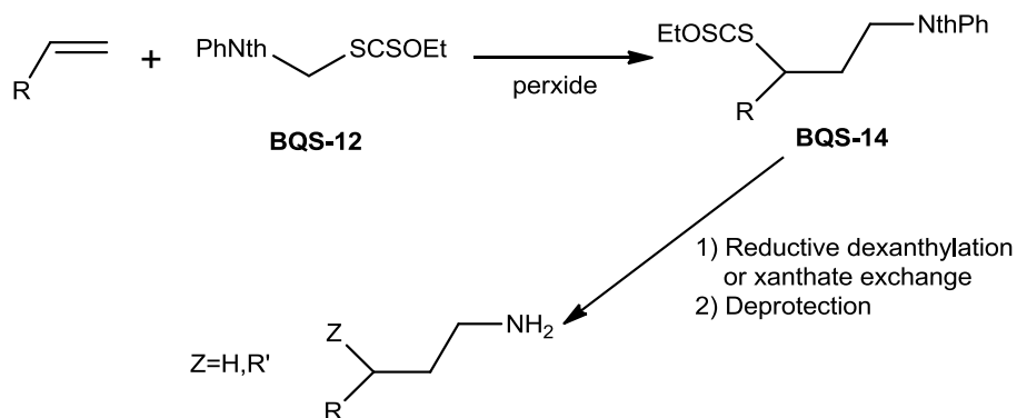
Scheme 2.34
