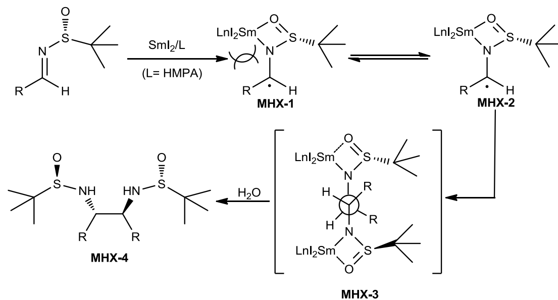
Scheme 4.5 Plausible mechanism
