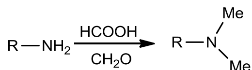
Scheme 2.15 Eschweiler-Clarke reaction
