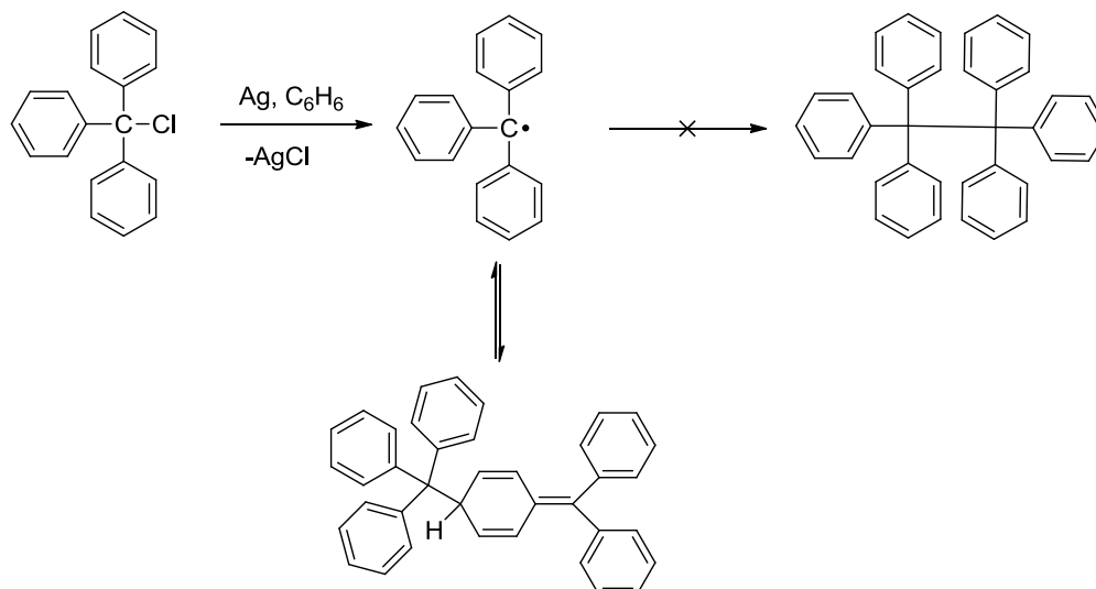
Scheme 1.2
