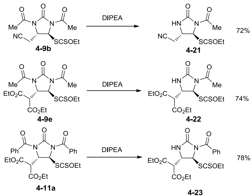
Scheme 4.23 Selective deprotection
