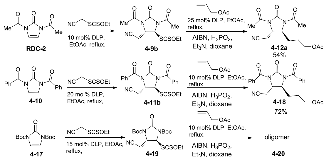
Scheme 4.22
