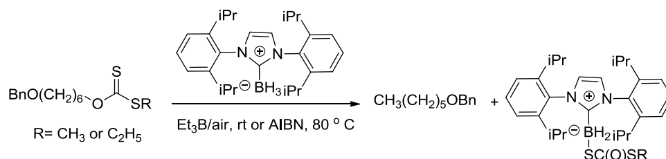
Scheme 1.21 Reductive elimination of xanthate group by using NHC-boranes
