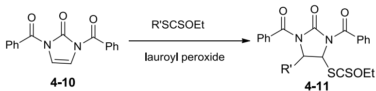
Scheme 4.17 Synthesis of 4-11
