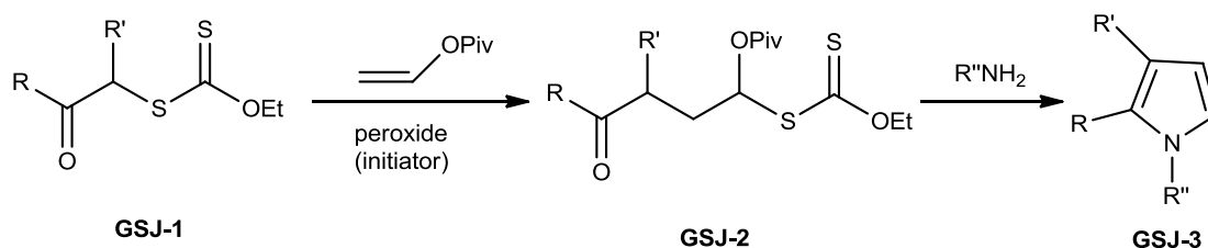
Scheme 5.17 Radical addition of \alpha -xanthyl ketones to vinyl pivalate
