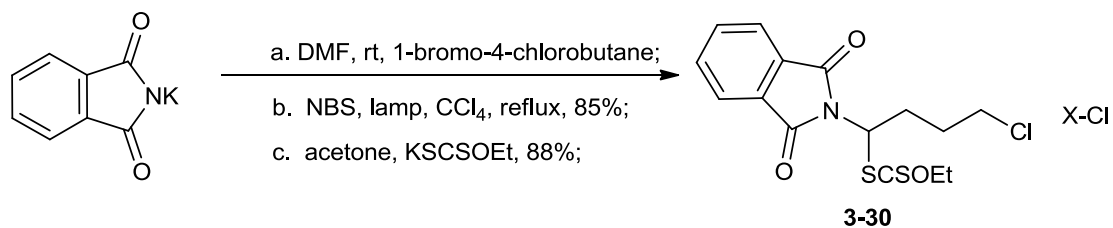
Scheme 3.28 Synthesis of xanthate 3-30
