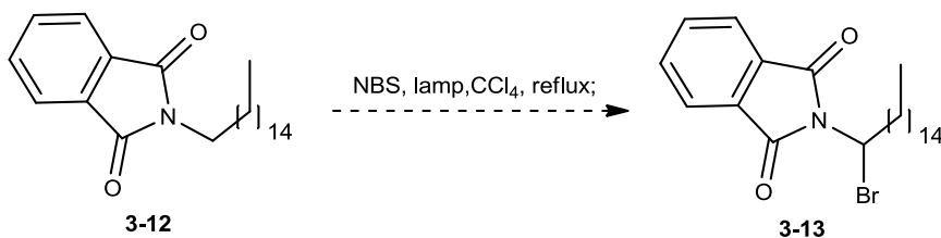
Scheme 3.11 Bromination of 3-12
