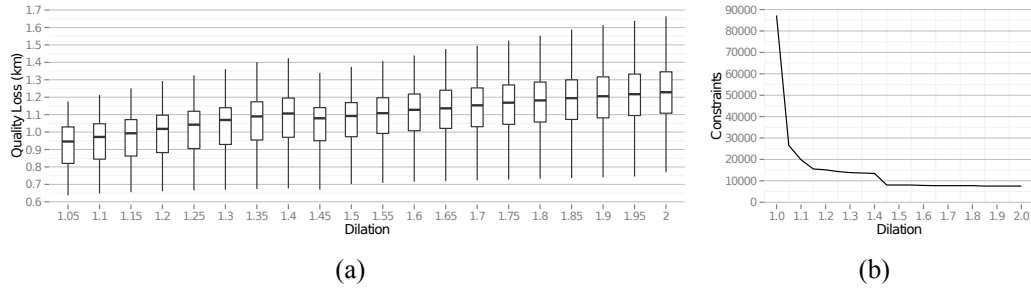
Figure 6.5: (a) Boxplot of the relation between QL and dilation for the mechanism OPTQL with privacy constraint \epsilon = 1.07 . The spanner is calculated with the greedy algorithm presented in Section 6.1.3. (b) Relation between the approximation ratio and the number of constraints in the linear program. This number is independent from the user and from the value of \epsilon .
