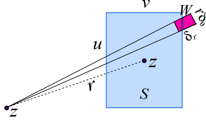
Figure 5.5: Bounding the probability of z in the discrete Laplacian.
