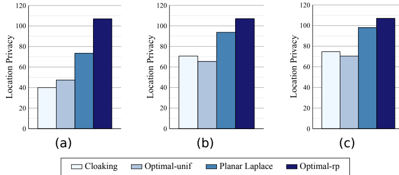
Figure 5.16: Location Privacy, in terms of \text{ADVERROR} , for \text{QL} = 107.03 m, for the four mentioned mechanisms, under priors (a) \pi_1 , (b) \pi_2 and (c) \pi_3 .
