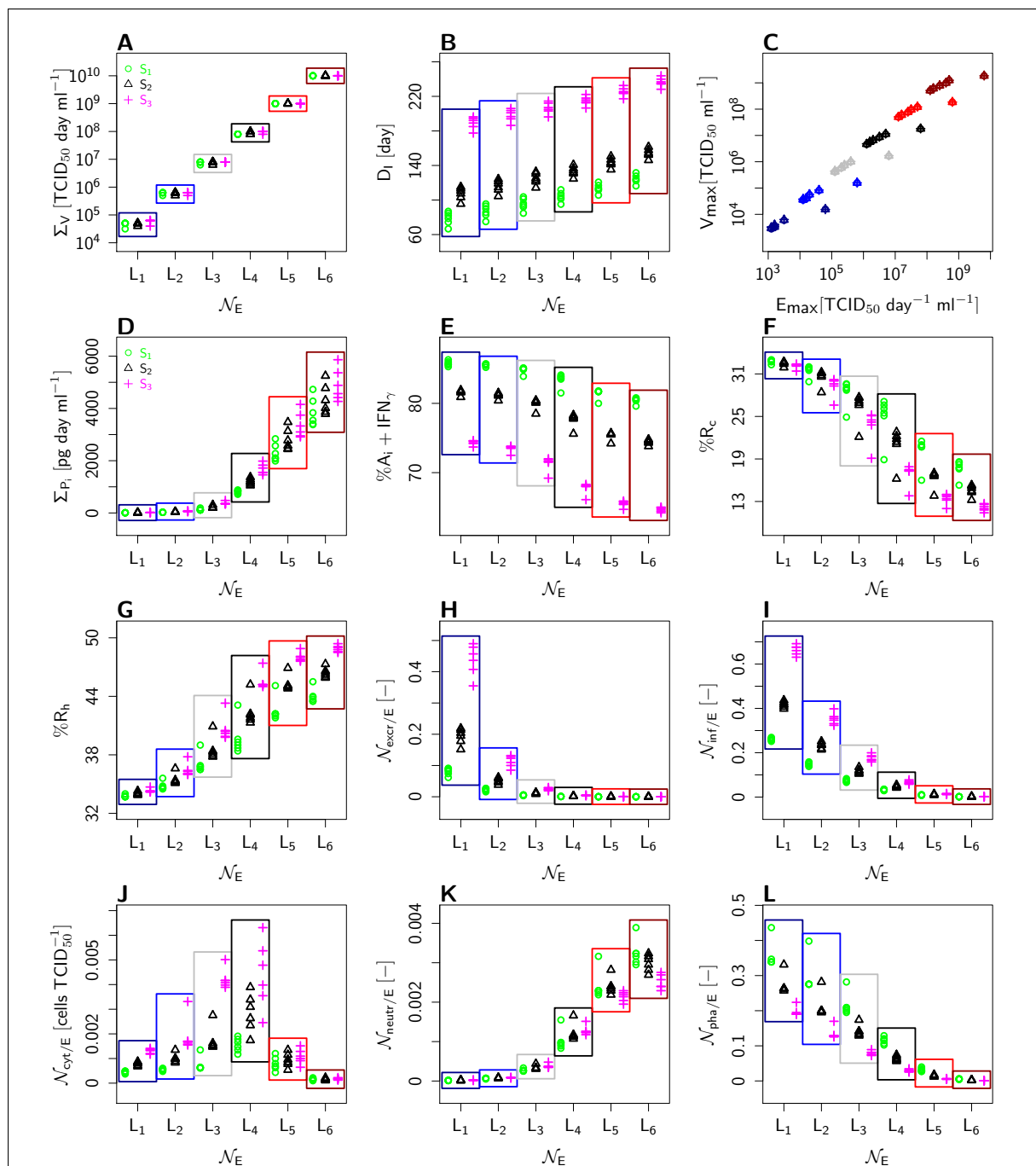
Figure III.10 Impact of scenario parameters on viral and immune characteristics for simple exposures (design D 1 ). A : total viral dose; B : infection duration D_I ; C : viral peak V_{max} ; D : total pro-inflammatory cytokines \Sigma_{P_i} ; E : percentage of antiviral cytokines \%(A_i + IFN_\gamma) ; F : percentage of cellular effectors \%R_c ; G : percentage of humoral effectors \%R_h ; H : normalised number of excreted viral particles \mathcal{N}_{excr/E} ; I : normalised number of viral particles having infected macrophages \mathcal{N}_{inf/E} ; J : normalised number of cytolysed infected macrophages \mathcal{N}_{cyt/E} ; K : normalised number of neutralised viral particles \mathcal{N}_{neutr/E} ; L : normalised number of phagocytosed viral particles \mathcal{N}_{pha/E} . All characteristics but the viral peak (all but C ) are plotted against the exposure intensity \mathcal{N}_E \in \{L_1, L_2, L_3, L_4, L_5, L_6\} , with the virulence level highlighted in colours : S_{vir} \in \{oS_1, \Delta S_2, +S_3\} ; replicates (same \mathcal{N}_E and S_{vir} ) and correspond to the various exposure durations. The viral peak ( C ) is plotted against the exposure peak E_{max} , with the exposure intensity highlighted in colours; replicates (same \mathcal{N}_E ) correspond to the different virulence levels and exposure durations. [-] = no unit.
