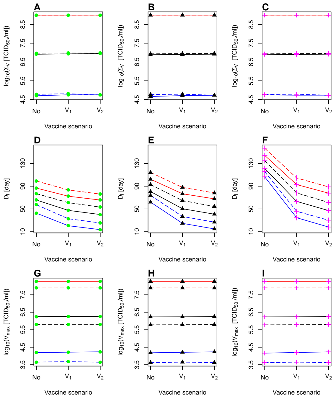
Figure IV.8 Viral characteristics for the virulence, exposure and vaccination scenarios. A–C total viral dose \Sigma_V ; D–F infection duration D_I ; G–I viral peak V_{\max} . 54 scenarios were simulated, crossing 3 exposure intensities \mathcal{N}_E \in \{L_1; L_3; L_5\} ; 2 exposure durations D_E : short 1-day exposure ( D_{E_s} , solid lines) and prolonged 20-day exposure ( D_{E_{p2}} , dashed lines); 3 virulence levels S_{\text{vir}} \in \{S_1, L_2, S_3\} ; and 3 vaccine scenarios: no vaccine, vaccine 1 V_1 and vaccine 2 V_2 .
