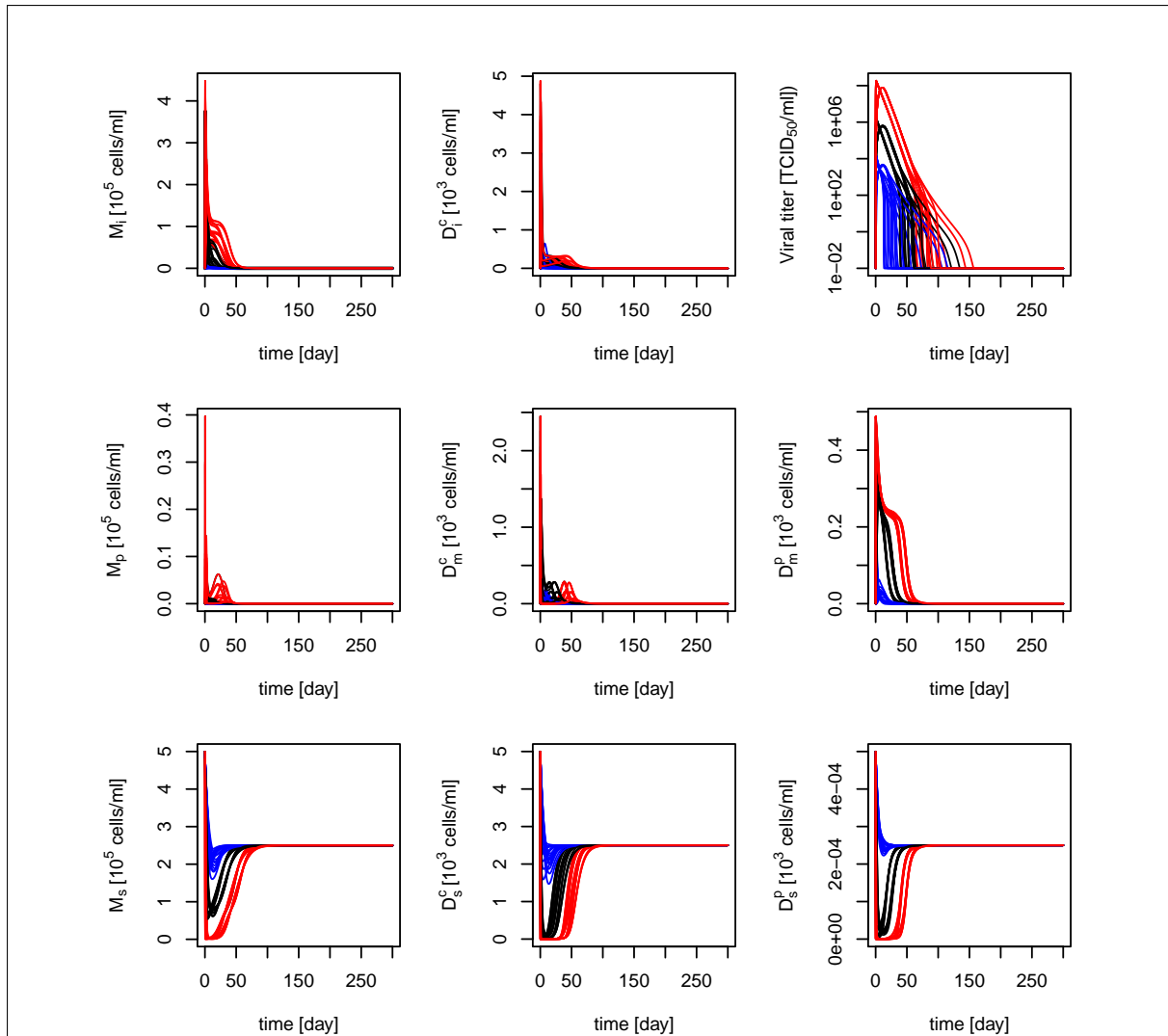
Figure C.4 PRRSv and antigen presenting cells dynamics for the 54 scenarios tested. C Viral titer ( V , semi-log graph). Antigen presenting cells : A infected macrophages ( M_i ), D phagocytosing macrophages ( M_p ) and G susceptible macrophages ( M_s ); B infected conventional dendritic cells ( D_i^c ), E mature conventional dendritic cells ( D_m^c ) and H susceptible conventional dendritic cells ( D_s^c ); F mature plasmacytoid dendritic cells ( D_m^p ) and I susceptible plasmacytoid dendritic cells ( D_s^p ). The 54 scenarios correspond to the 3 vaccination strategies ( V_s \in \{\text{No}, V_1, V_2\} ), crossed with 3 virulence levels ( S_{\text{vir}} \in \{S_1, S_2, S_3\} ), 2 exposure durations ( D_E \in \{D_{E_s} = 1 \text{ day}, D_{E_{p2}} = 20 \text{ day}\} ), and 3 exposure intensities ( \mathcal{N}_E ) highlighted in colours : L_1 = 10^{4.3} TCID 50 /ml, L_3 = 10^{6.3} TCID 50 /ml, L_5 = 10^{8.3} TCID 50 /ml.
