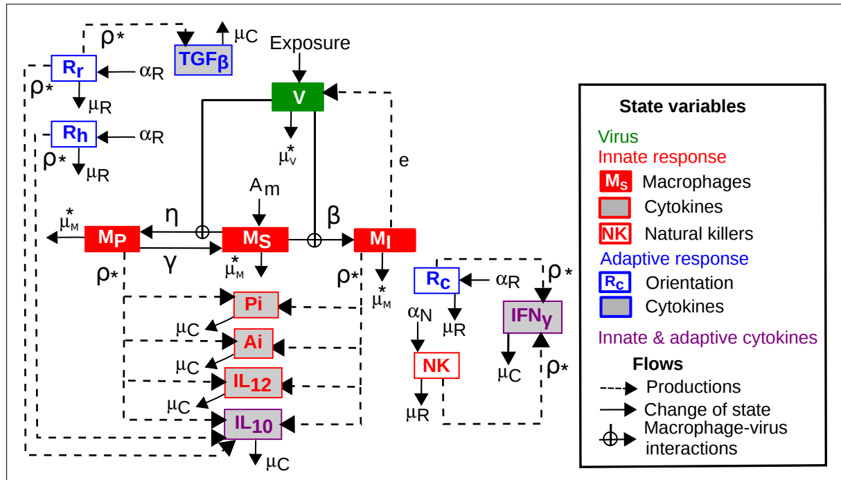
Figure I.2 Conceptual model : state variables and flows without regulations. The state variables consist of : the free viral particles ( V ); the susceptible ( M_s ), phagocytosing ( M_p ) and infected ( M_i ) macrophages; the natural killers ( NK ); the cellular ( R_c ), humoral ( R_h ) and regulatory ( R_r ) adaptive effectors; the pro-inflammatory cytokines ( P_i ), the innate antiviral cytokines ( A_i ) and the immuno-regulatory cytokines ( IL_{12} , IFN_\gamma , IL_{10} & TGF\beta ). The flows represented are : the viral exposure E(t) ; the recruitment of susceptible macrophages ( A_m ); the activation of natural killers ( \alpha_N ) and cells of the adaptive response ( \alpha_R ); the decay of the free viral particles ( \mu_V ), the macrophages ( \mu_M^* ), the natural killers ( \mu_N ), the adaptive cells ( \mu_R ) and the cytokines ( \mu_C ); the macrophage state changes, i.e. phagocytosis ( \eta and \gamma ) and the infection ( \beta ); the excretion of free viral particles by infected macrophages ( e ) and the cytokine syntheses by activated immune cells ( \rho^* ). For the sake of readability, the cytokine and cell regulations and not drawn and some parameter notations (marked with *) are simplified.
