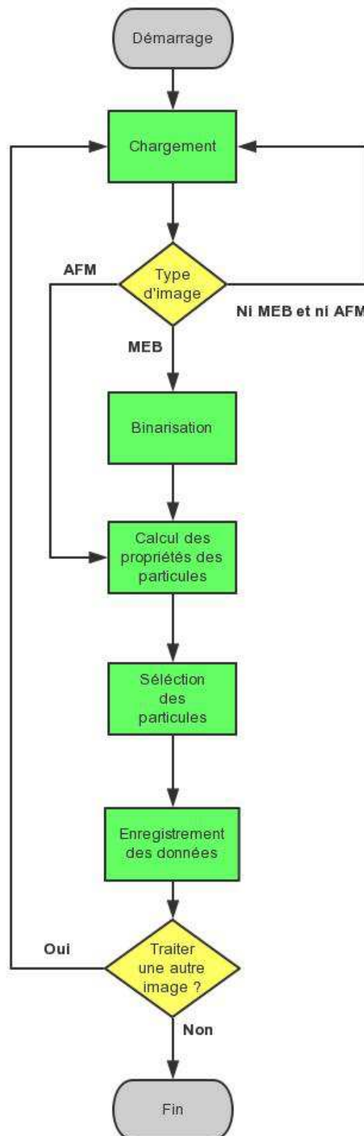
Figure 5-17 : Processus principal du programme Nanoselect.
