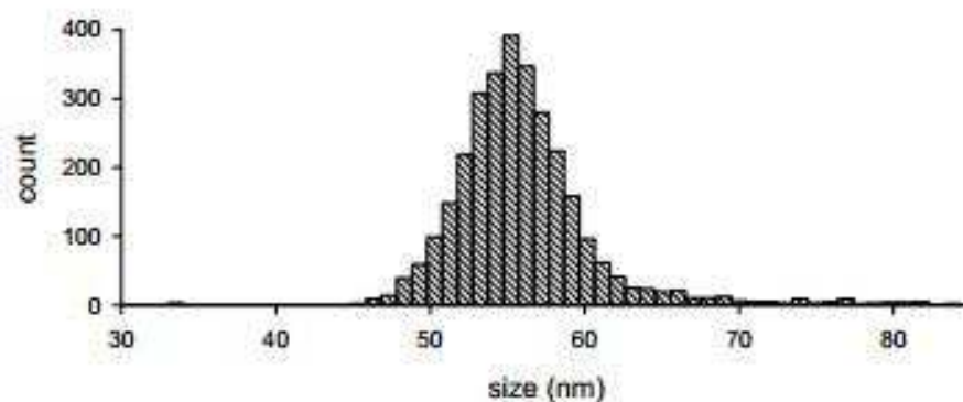
Figure 6. Particle size histogram generated by TEM analysis.
