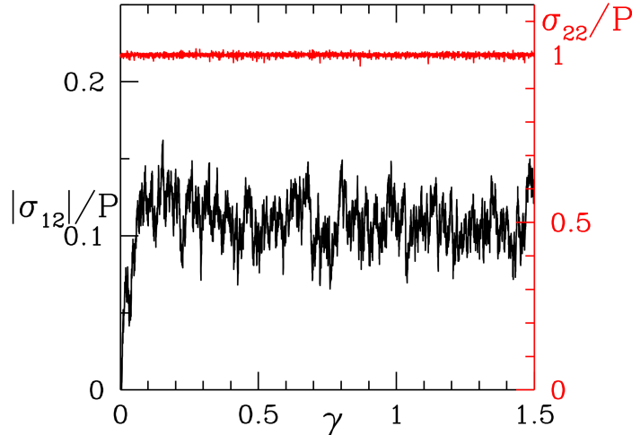
Figure 1.18: \sigma_{12} (left axis, in black) and \sigma_{22} (right axis, in red) as functions of shear strain \gamma . Results of [104], 3D simulations of rigid frictionless grains, under a constant normal stress P , with I = 3 \times 10^{-5} .
