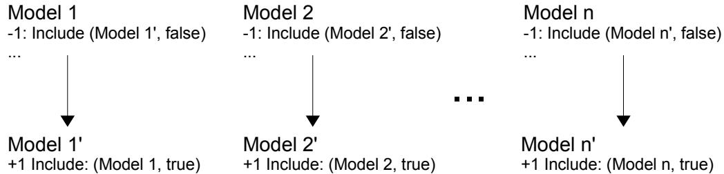
Figure 7.5. Module substitution in general: Modules are substituted by providing alternative module implementations in additional models. Replacing includes in the original models towards the additional models enable the substitution.
