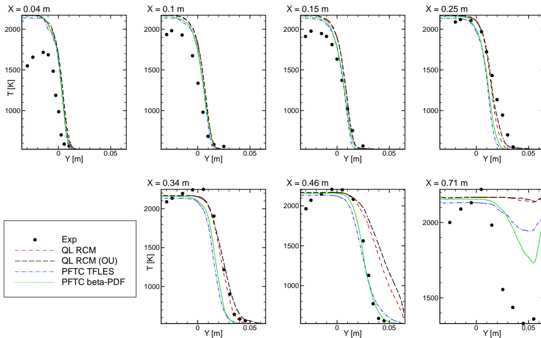
Figure 6.42: Vertical profiles of mean temperature \langle \tilde{T} \rangle in reactive backward-facing step flow; LES
