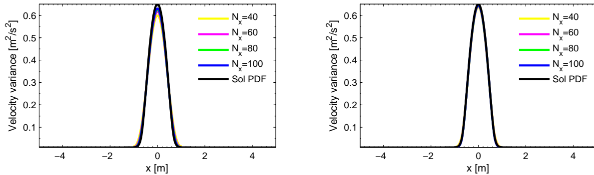
Figure A.44: Scheme non-dissipativity test: spatial profile of velocity variance at time t = 0.2 s. Left: stochastic GForce method, right: stochastic Godunov method. N_r = 10^7 .
