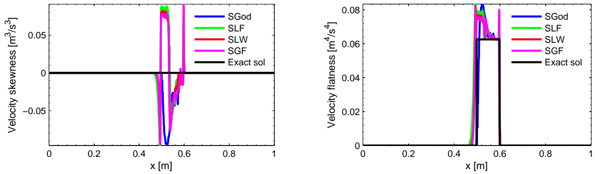
Figure 3.11: Backward step: spatial profiles of Favre skewness (left) and flatness (right) of velocity at time t = 0.1 s with mean correction of density (3.118). N_r = 10^4 , N_x = 10^3 .
