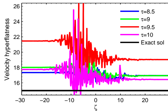
Figure 3.60: Statistically homogeneous velocity fluctuations test: spatial profiles of velocity hyperflatness at \tau \geq 8.5 calculated by kinetic scheme after normalization (3.168). N_r = 4800 , N_x = 3 \times 10^4 on D = [-150; 150] .
