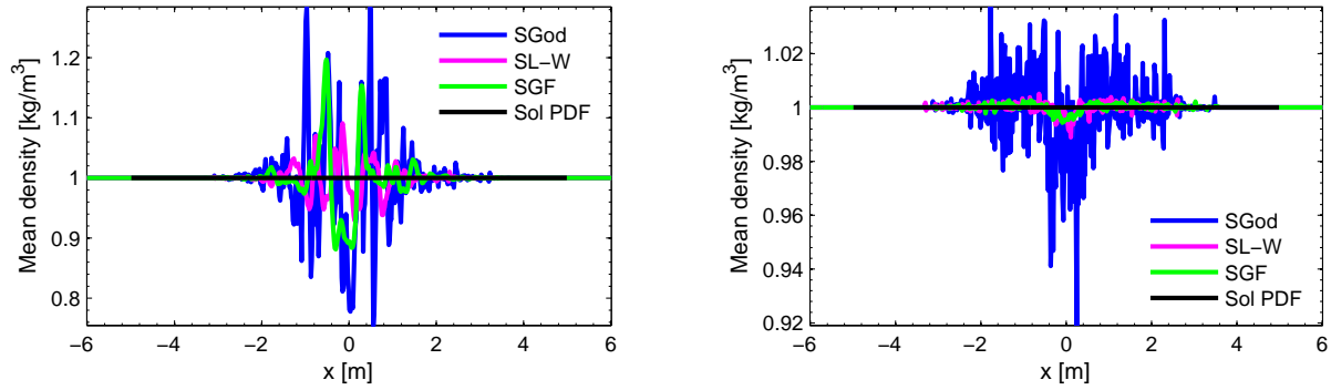
Figure 3.80: Model PDF eq. with non-zero RHS: spatial profile of mean density at time 3s; left: without mean velocity correction, right: with mean velocity correction. N_r = 2000 , N_x = 612 .
