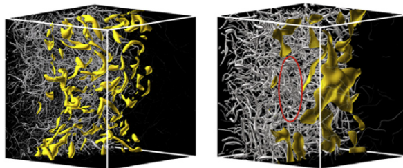
Figure 2.10: Results from recent DNS of combustion at moderate Re_t and Da numbers from [TanahashiSato2008]. Figures show iso-surfaces of the heat-release (yellow) and vorticity (gray) from a planar flame in homogeneous isotropic turbulence at Re_t \approx 515 and 141, Da \approx 21 and 5, and Ka \approx 1.3 and 2.8, respectively.
