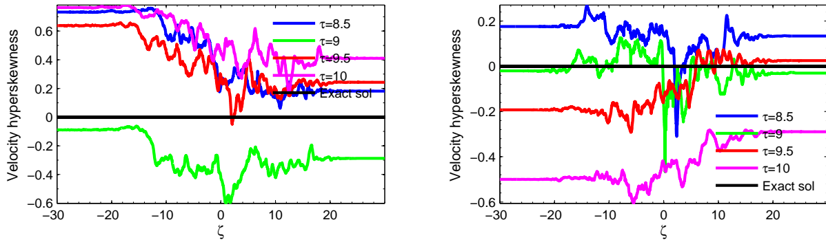
Figure 3.55: Statistically homogeneous velocity fluctuations test: spatial profiles of velocity hyperskewness at \tau \geq 8.5 . Left: stochastic Lax-Wendroff method; right: stochastic GForce method. N_r = 4800 , N_x = 3 \times 10^4 on D = [-150; 150] .
