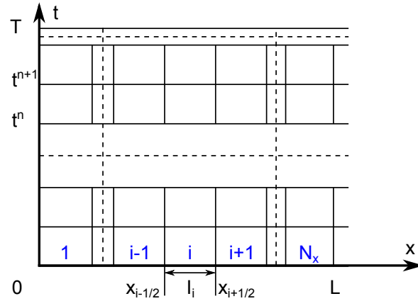
Figure A.1: Discretization of [0, L] interval into N_x finite volumes
