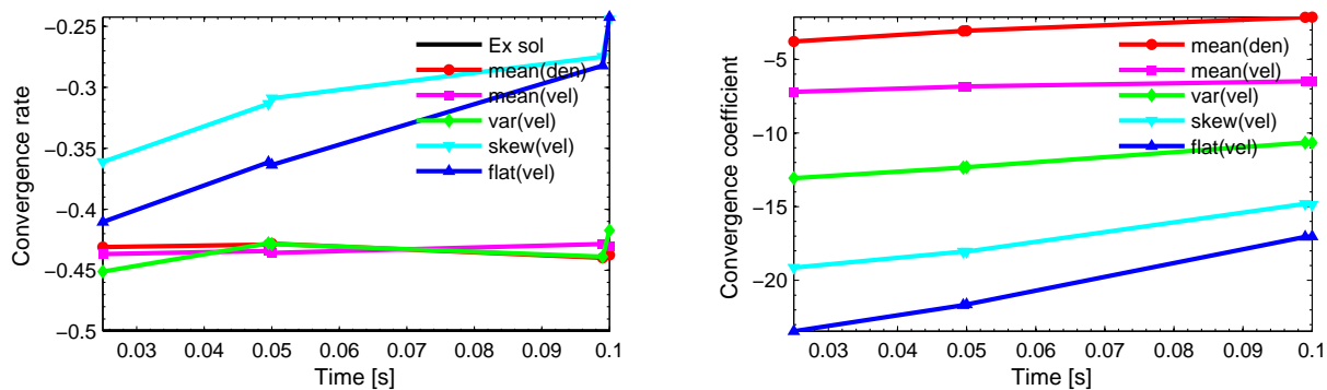
Figure A.37: Hat: time evolution of the statistical convergence rates (left) and coefficients (right) for moments of density and velocity; stochastic GForce method. N_x = 10^4 .
