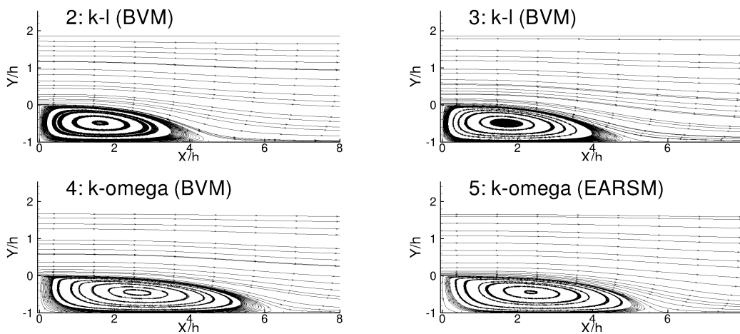
Figure 6.8: Recirculation regions in nonreactive backward-facing step flow; 2: k - l (BVM) model with homogeneous inlet profiles, 3: k - l (BVM) model with nonhomogeneous inlet profiles, 4: k - \omega (BVM) model with homogeneous inlet profiles, 5: k - \omega (EARSM) model with homogeneous inlet profiles
