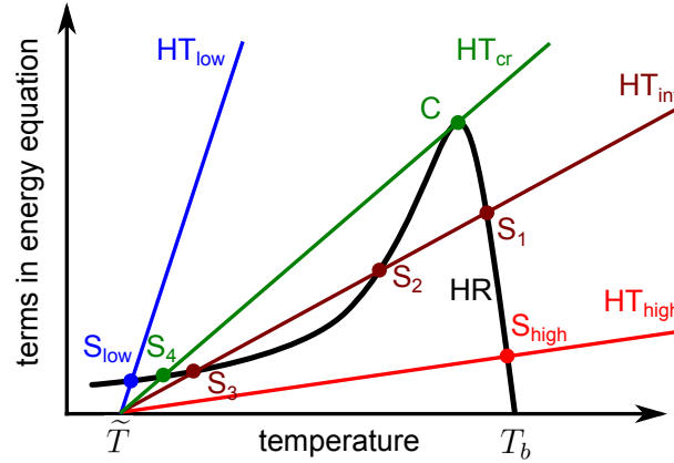
Figure 2.11: The dependence of the rates of heat release HR and of heat losses HT_{low} , HT_{cr} , HT_{int} and HT_{high} on the temperature for various heat transfer conditions
