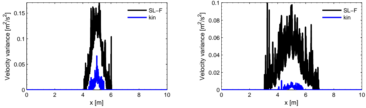
Figure 3.28: Scheme non-dissipativity test: spatial profile of velocity variance at 4t_c (left) and at 10t_c (right). N_r = 10^4 , N_x = 10^4 .
