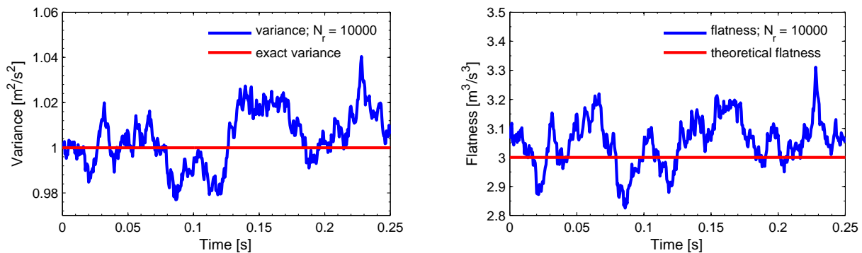
Figure A.67: Comparison of variance (left), flatness (right) with their theoretical values
