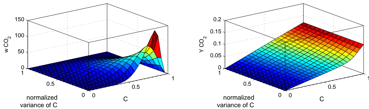
Figure 4.2: Production rate (left) and mass fraction (right) of CO_2 ; obtained from PFTC \beta -PDF table of the premixed flame CH_4/O_2 , \tilde{Z} = 0.0455 , \widetilde{Z''^2} = 0 , N_c = 25 , N_{VarC} = 15
