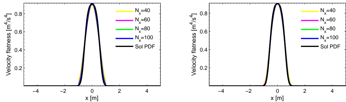
Figure A.47: Scheme non-dissipativity test: spatial profile of velocity flatness at time t = 0.2 s. Left: stochastic Lax-Friedrichs method, right: stochastic Lax-Wendroff method. N_r = 10^7 .
