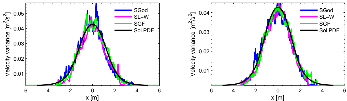
Figure 3.82: Model PDF eq. with non-zero RHS: spatial profile of Favre velocity variance at time 3s; left: without mean velocity correction, right: with mean velocity correction. N_r = 2000 , N_x = 612 .
