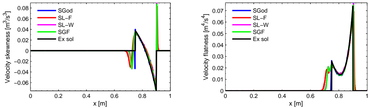
Figure A.32: Triangle: spatial profiles of velocity skewness (left) and flatness (right) at time t = 0.4 s. N_r = 10^4 , N_x = 5 \times 10^3 .
