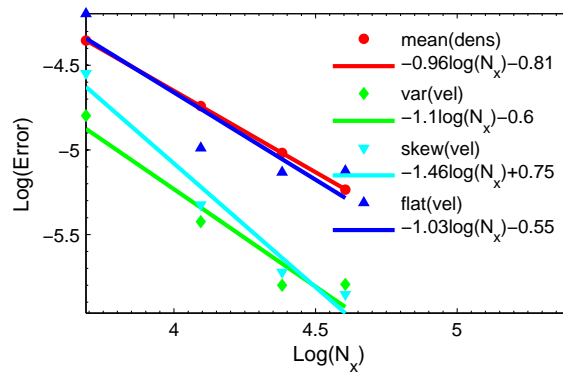
Figure 3.86: Model PDF eq. with non-zero RHS: spatial convergence of stochastic Godunov method. N_r = 10^6 .
