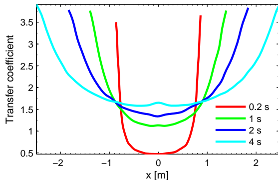
Figure 3.77: Model PDF eq. with non-zero RHS: transfer coefficient calculated with PDF
