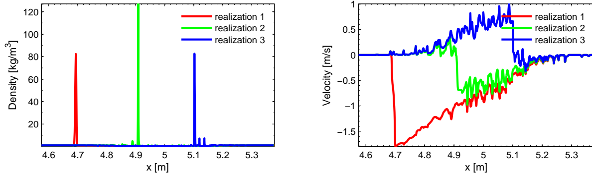
Figure 3.29: Scheme non-dissipativity test: examples of stochastic density (left) and velocity (right) fields at 2t_c calculated with kinetic scheme. N_r = 10^4 , N_x = 10^4 .
