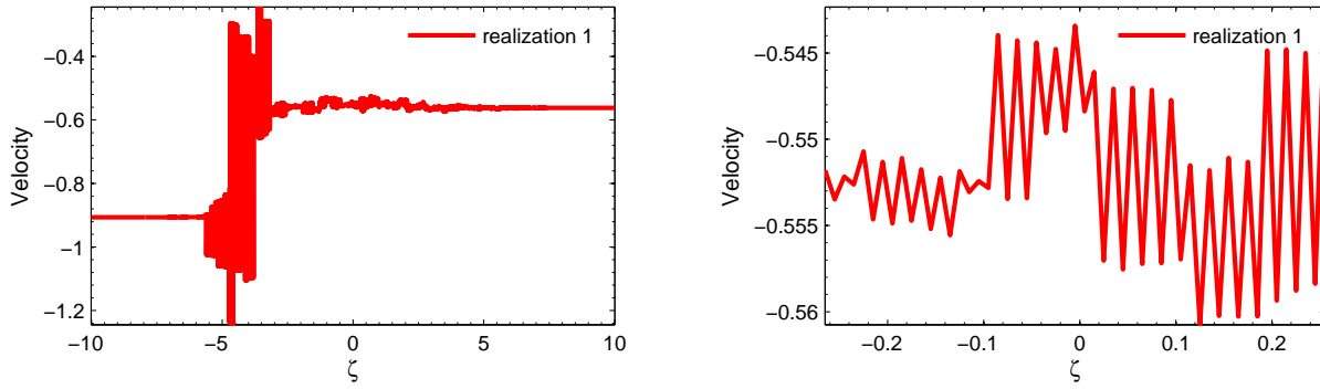
Figure 3.70: Statistically homogeneous velocity fluctuations test: spatial profile of one realization of velocity (left) and its zoom (right) at \tau = 2 ; stochastic Lax-Friedrichs method. N_r = 4800 , N_x = 3 \times 10^4 on D = [-150; 150] .
