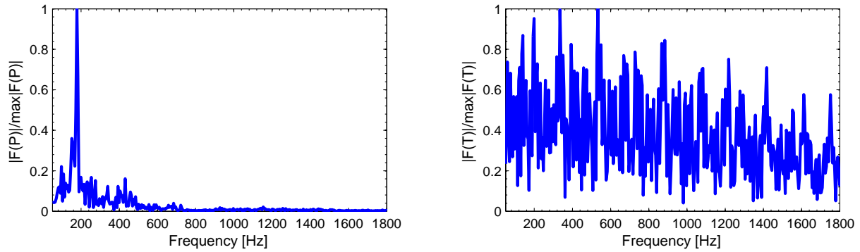
Figure 6.54: Spectra of pressure (left) and temperature (right) at point C in reactive backward-facing step flow; LES/PFTC \beta -PDF
