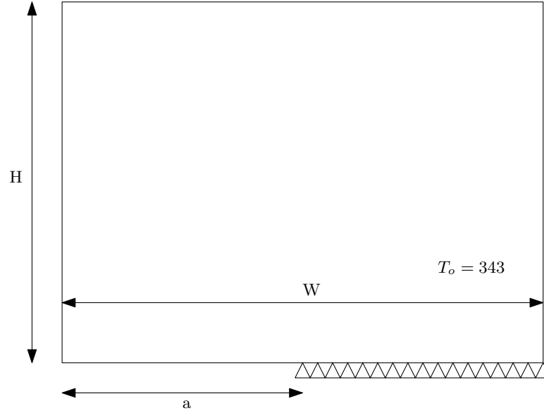
Figure 5.5. The geometry of the problem and the boundary conditions (W = 100 \text{ mm}, H = 100 \text{ mm}, a = 50 \text{ mm}) .
