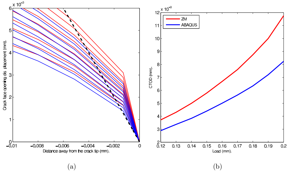
Figure 3.18. (a) Crack face opening profiles for increasing u . Half of the CTOD is measured from the intercept of 45^\circ line (dashed line starting from the crack tip) and the crack profile (b) CTOD values
