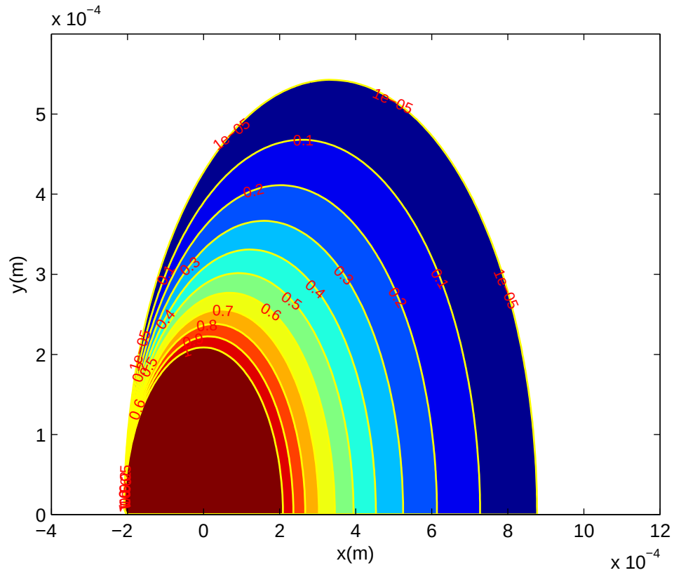
Figure 5.4. Martensite transformation region, thermomechanical coupling is not included, T_0 = 343 \text{ K}
