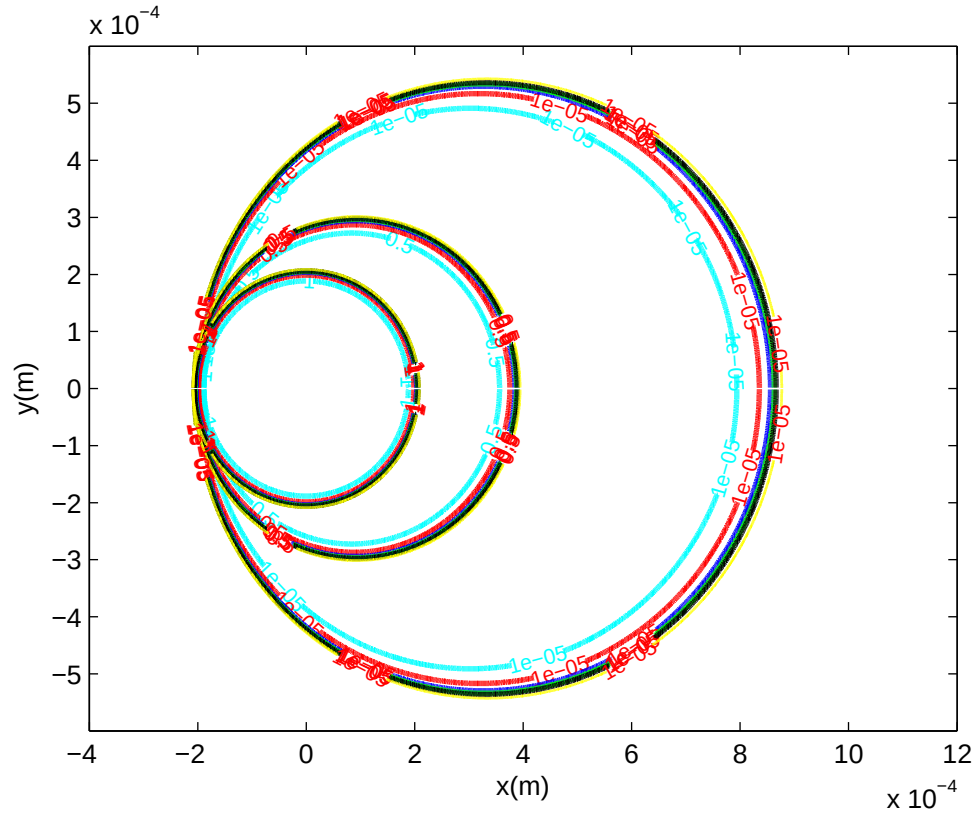
Figure 5.7. \zeta contours. \zeta = 1 is the inner circle, \zeta = 0.5 is the middle circle, \zeta = 1 \times 10^{-5} represents the outer circle. Colours: cyan: \dot{k}^\infty = 2.56 \times 10^{-5} (1/s) , red: \dot{k}^\infty = 1.280 \times 10^{-5} (1/s), blue: \dot{k}^\infty = 0.64 \times 10^{-5} (1/s), green: \dot{k}^\infty = 0.43 \times 10^{-5} (1/s), black: \dot{k}^\infty = 0.32 \times 10^{-5} (1/s) and yellow curve is when the latent heat generation is neglected
