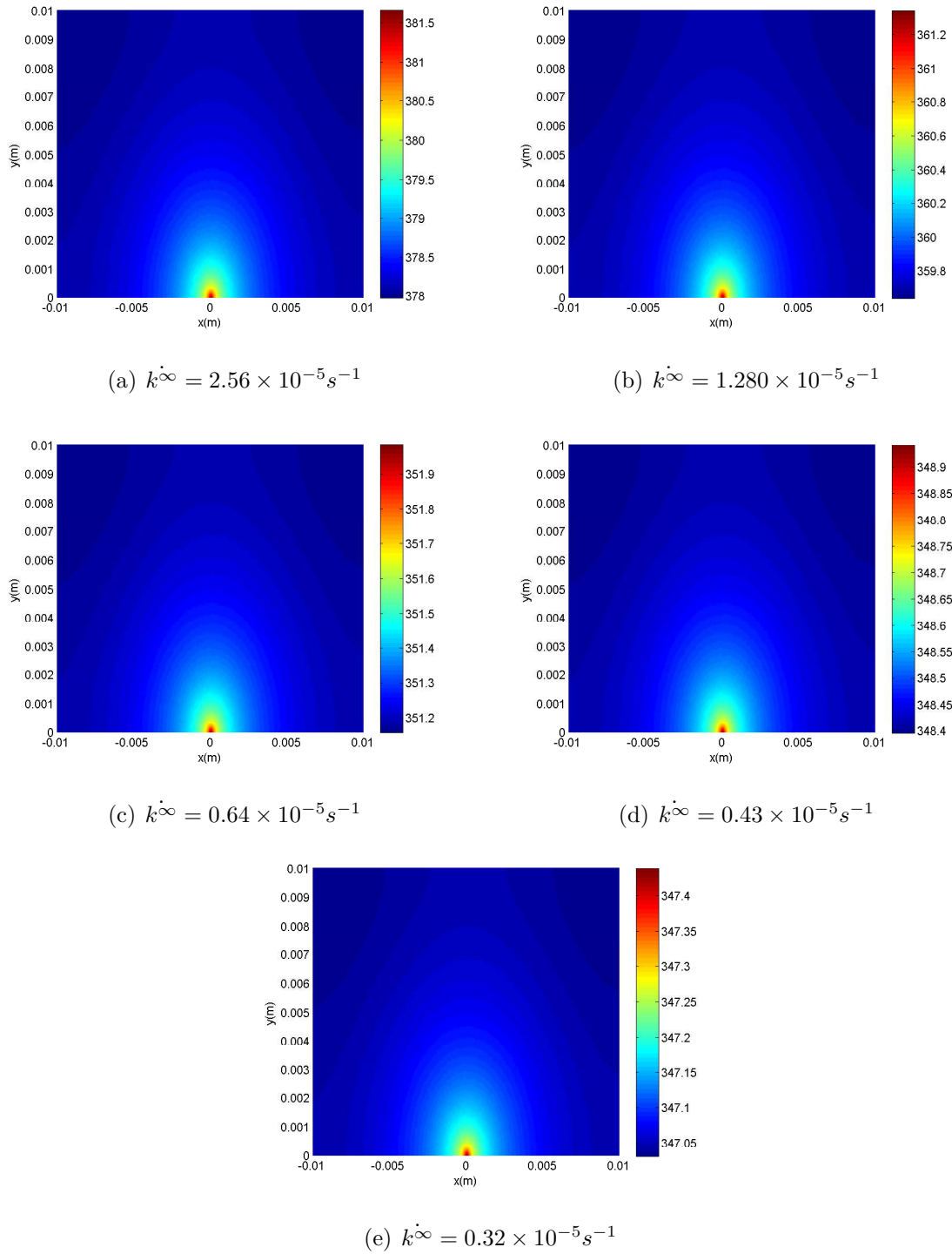
Figure 5.8. Temperature increase due to thermomechanical coupling.
