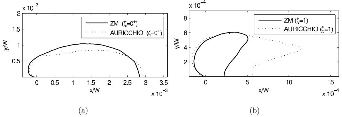
Figure 3.4. (a) Phase transformation regions, \zeta = 0^+ , (b) Full martensite region, \zeta = 1 , ( a/W = 0.40 ).
