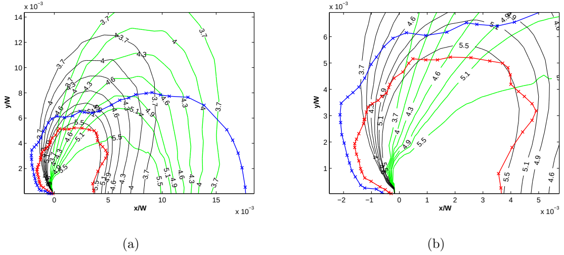
Figure 2.3. (a) Contour plot of normalized opening stress, \frac{\sigma_{yy}}{\sigma_0} ( \sigma_0 being far field applied stress), from the full field finite element solution (green lines) and from the asymptotic field (black lines). Red line represents martensite region \zeta = 1 and the region between red and blue lines is the transformation region 0 < \zeta < 1 . In both cases crack tip is located at the origin and only half-plate is shown. (b) close up view of the stress contours, \frac{\sigma_{yy}}{\sigma_0} , near the crack tip.
