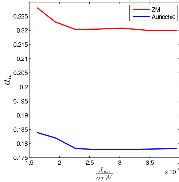
Figure 3.19. d_n values.
