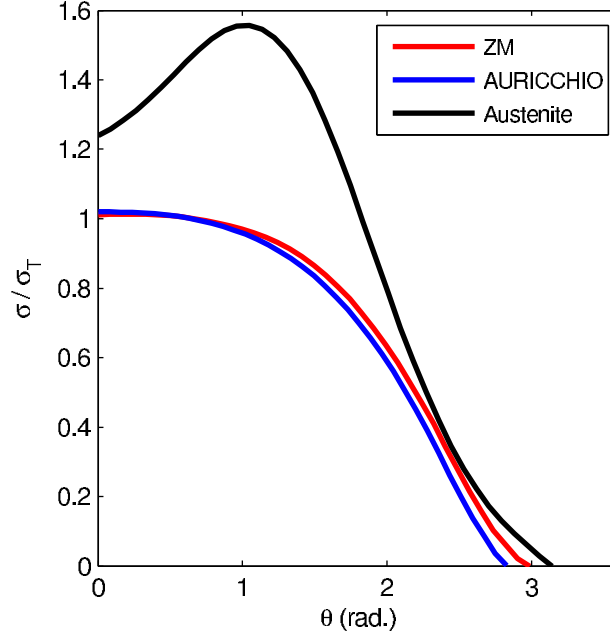
Figure 3.8. Angular variation of the \frac{\sigma_{yy}}{\sigma_T} where \sigma_T is the average transformation stress along a radial path ( r = 0.18mm ). The crack tip is located at the origin. ( a/W = 0.40 and u = 0.1 mm ).
