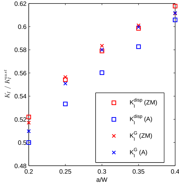
Figure 3.15. Comparison of stress intensity factors normalized by K_I^{aus} , which is the SIF calculated for a linear elastic material with material properties identical to NiTi in the austenitic phase. (ZM: Zaki-Moumni model A: Auricchio's Model).
