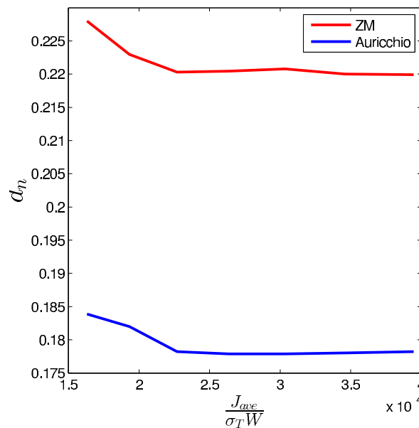
Figure 3.19. d_n values.
