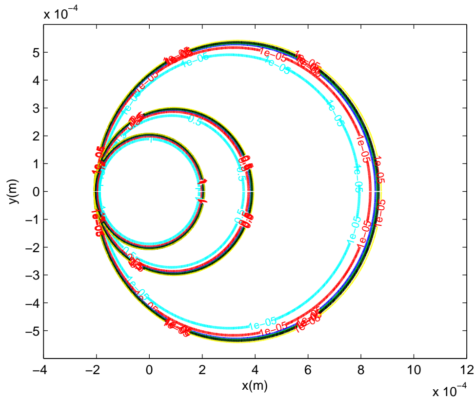
Figure 5.7. \zeta contours. \zeta = 1 is the inner circle, \zeta = 0.5 is the middle circle, \zeta = 1 \times 10^{-5} represents the outer circle. Colours: cyan: k^{\dot{\infty}} = 2.56 \times 10^{-5} (1/s), red: k^{\dot{\infty}} = 1.280 \times 10^{-5} (1/s), blue: k^{\dot{\infty}} = 0.64 \times 10^{-5} (1/s), green: k^{\dot{\infty}} = 0.43 \times 10^{-5} (1/s), black: k^{\dot{\infty}} = 0.32 \times 10^{-5} (1/s) and yellow curve is when the latent heat generation is neglected
