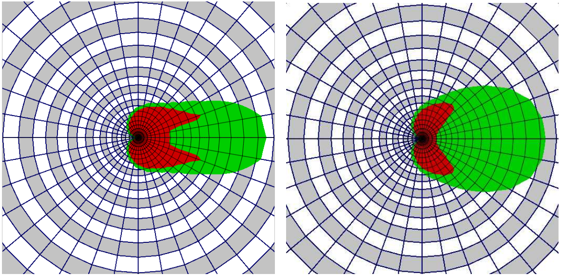
Figure 3.5. Transformation region, red ( \zeta = 1 ), green ( 0 < \zeta < 1 ) and J-Integral contours (white and gray), ( a/W = 0.40 ).
