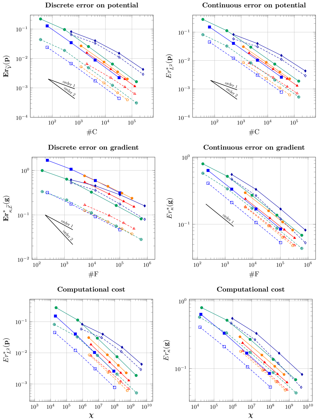
Figure 8.9 – Comparison between HCb-DGA (labels A) and HCb-SUSHI (labels B) schemes of the error on potential (top row), of the error on its gradient (middle row), and of the cost-effectiveness (bottom row).
