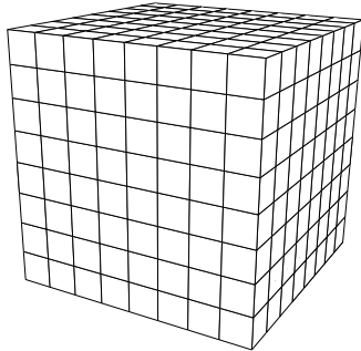
Figure A.1 – Left: Successive refinement of the Hex mesh sequence. Right: Tables collecting the cardinality of primal sets, mesh quality criteria, and the regularity of the barycentric subdivision for the meshes of the Hex mesh sequence.
