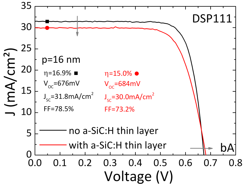
Figure 4-18 – JV characteristics of SHJ solar cells fabricated with and without a thin a-SiC:H layer at the a-Si:H/c-Si interface on flat (111) c-S wafers (as-deposited).
