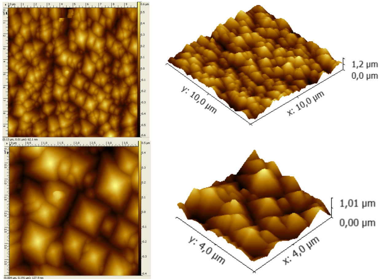
Figure 3-39 – AFM mapping of a 10x10 and 4x4 μm 2 region on a CAL textured wafer.
