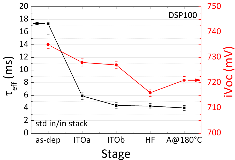
Figure 4-46 – Evolution of the effective lifetime and iV_{\text{oc}} of a symmetrical in/in stack deposited on flat (100) c-Si wafer upon bilateral ITO deposition, removal thereof, and annealing.
