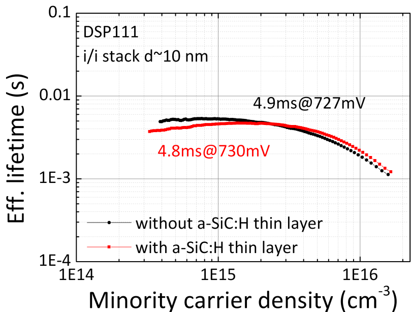
Figure 3-38 – Effective lifetimes of two i/i stacks on flat (111) wafers. One has a thin a-SiC:H layer at the a-Si:H/c-Si interface, the second does not.
