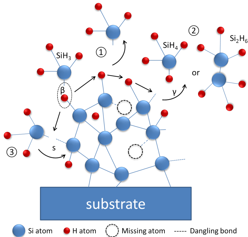
Figure 1-20 — Schematic representation the possible interactions between a SiH 3 radical produced from the dissociation of SiH 4 in a plasma and the surface of the growing a-Si:H layer.
