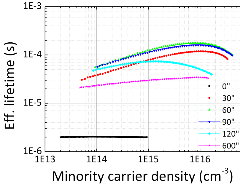
Figure 3-18 – Effective lifetime of an textured Klno c-Si wafer measured after various 2nd HF dip times.
