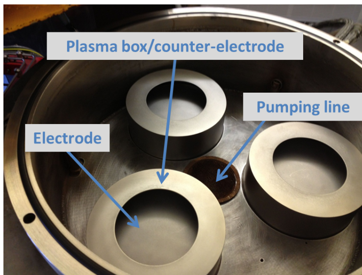
Figure 1-21 — Inside view of the ARCAM reactor. Three plasma confinement boxes can be seen with their RF electrode.
