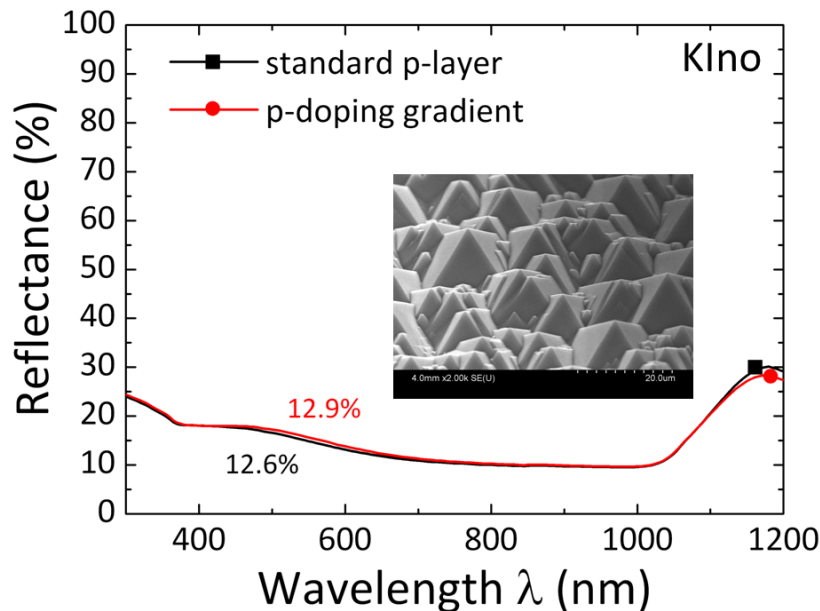
Figure 4-70 – Reflectance as a function of wavelength measured on the emitter side of the Klno cells: with a standard p-layer (black square) and with a graded p-layer (red dot).
