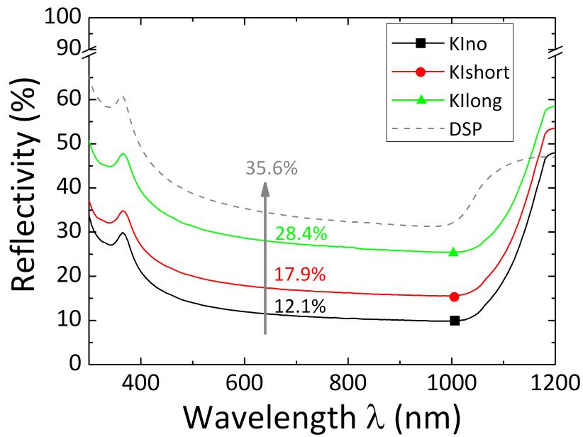
Figure 3-78 – Reflectivity as a function of the light wavelength for a Klno wafer, before and after chemical polishing in a CP133 chemical bath.
