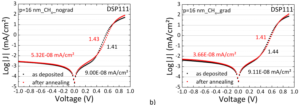
Figure 4-65 – Evolution upon annealing of the dark JV characteristics of SHJ solar cells fabricated a) without and b) with a p-doping gradient on flat (111) c-Si wafers.
