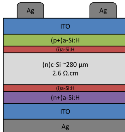
Figure 4-4 – Sketch of an n-type SHJ solar cell fabricated on a flat 2.6 Ω·cm c-Si wafer. The structure is not drawn to scale.
