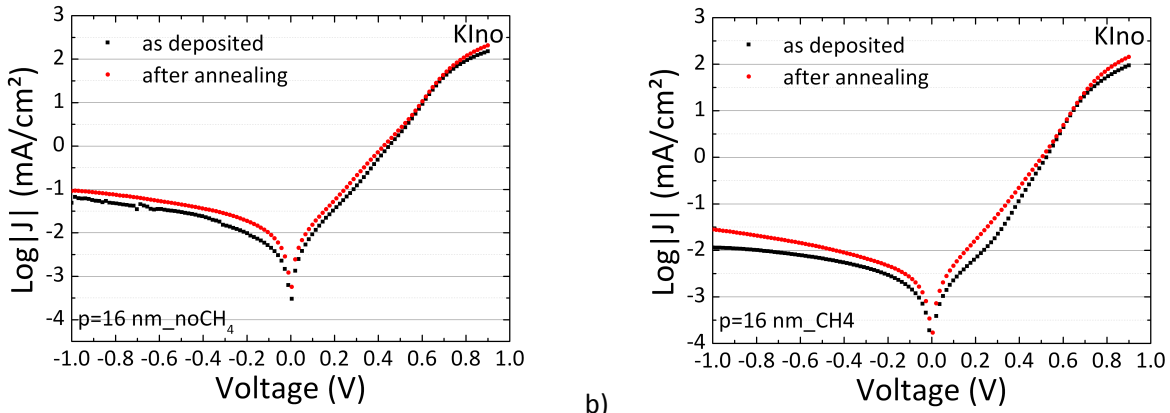
a) b) Figure 4-29 – Evolution upon annealing of the dark JV characteristics of SHJ solar cells fabricated a) without and b) with a thin a-SiC:H layer at the a-Si:H/c-Si interface on KTno textured c-Si wafers.
