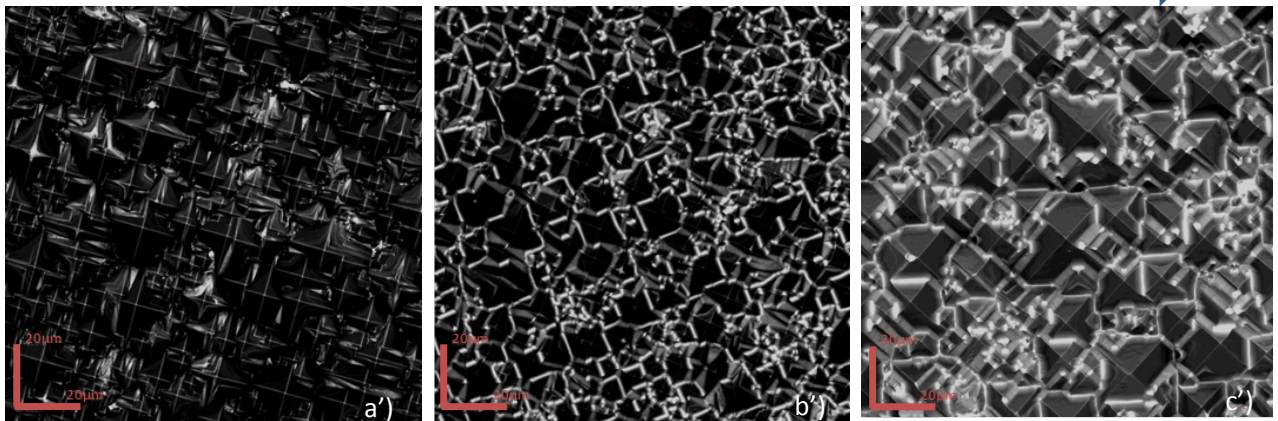
Figure 3-77 – LSM(upper part) and SEM(lower part) images of KOH-IPA before and after chemical polishing in CP133.
