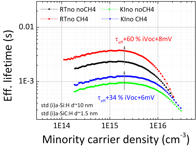
Figure 3-37 – Effective lifetime of RTno and Klno textured wafer passivated by a 10 nm-thick (i)a-Si:H layer with and without a thin a-SiC:H layer at the interface.
