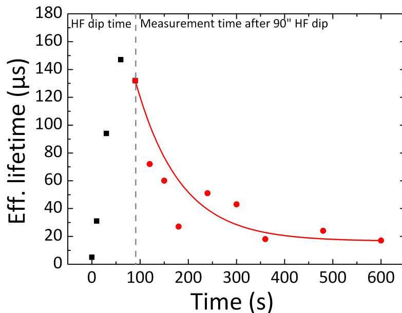
Figure 3-19 – Decay of the effective lifetime of a Klno c-Si wafer after a 90 sec 2nd HF dip.
