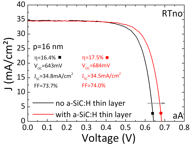
Figure 4-32 – JV characteristics of SHJ solar cells fabricated with and without a thin a-SiC:H layer at the a-Si:H/c-Si interface on RTNo textured c-Si wafers (annealed).
