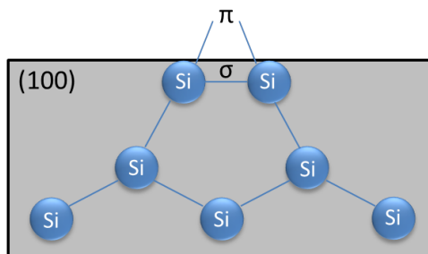
Figure 2-4 – Schematic representation of the Si(100)-(2x1) dimer structures as a result of the interaction between two T_2^0 dangling bond orbitals.
