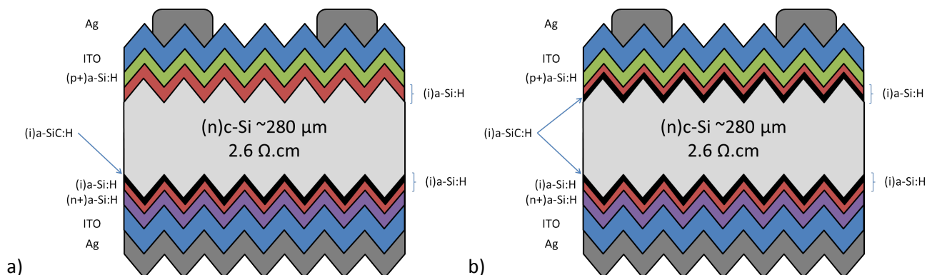
Figure 4-22 – Schematic representation of a classical HiT cell, as developed by Sanyo[240][176] with an additional thin a-SiC:H layer at the back a-Si:H/c-Si interface (left-hand side), and of an “improved” HiT structure containing a thin a-SiC:H layer at the back and at the front a-Si/c-Si interface (right-hand side). These structures are not drawn to scale.
