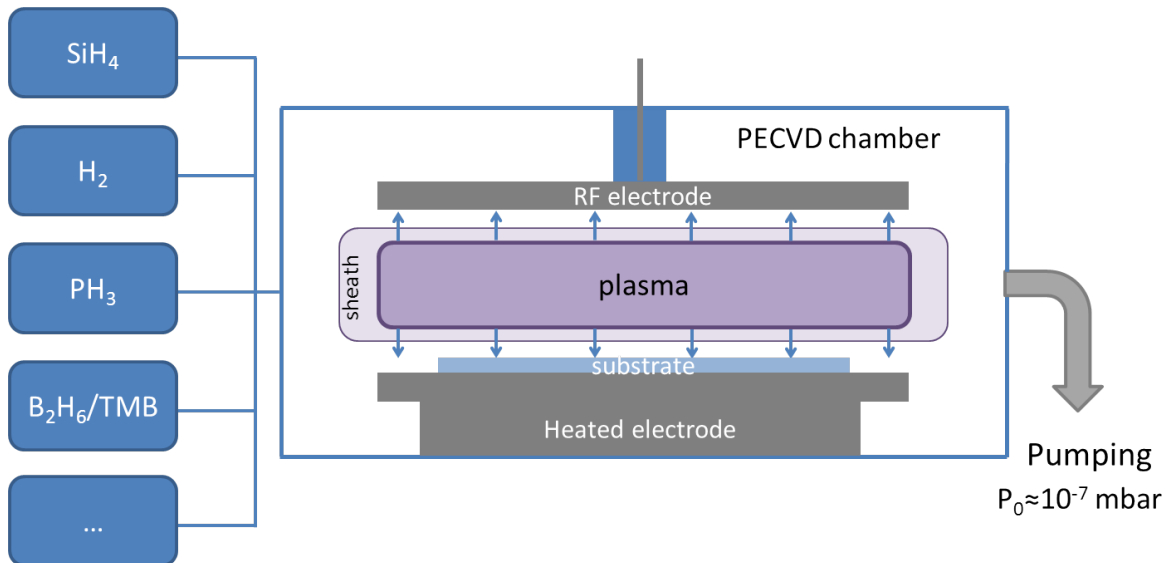
Figure 1-17 — Schematic diagram of basic PECVD deposition reactor. It consists of a gas injection system, a vacuum chamber and of a parallel plate system (RF power electrode + grounded and heated substrate holder). This system has allowed for uniform a-Si:H deposition on substrate sizes up to 5.7 m 2 .
