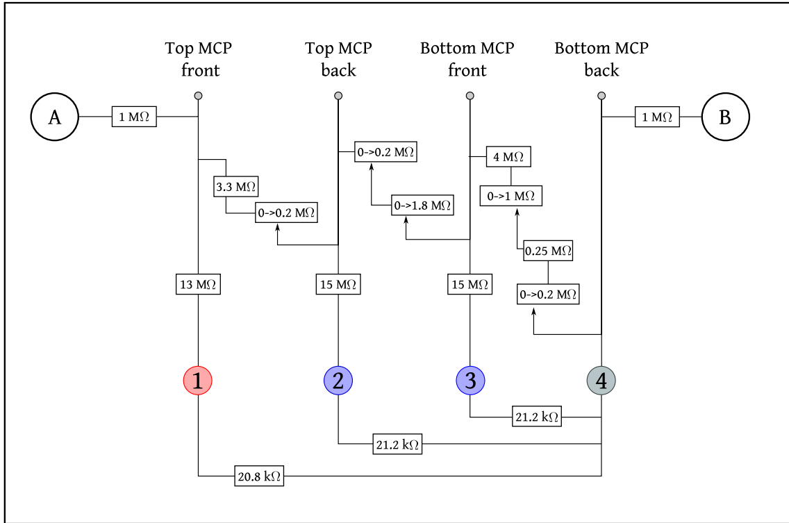
Figure 1.11: The electronics designed by F. Moron, that allow us to divide the total voltage into dV and V_{mcp} . The total voltage is put over A and B, the high voltage going to the MCPs are indicated. The numbered red, blue and black points are where we can measure the voltage over the respective channels. The measured voltage is 1/100 of the true signal, for safety reasons. The electronics are put in a plastic box.
