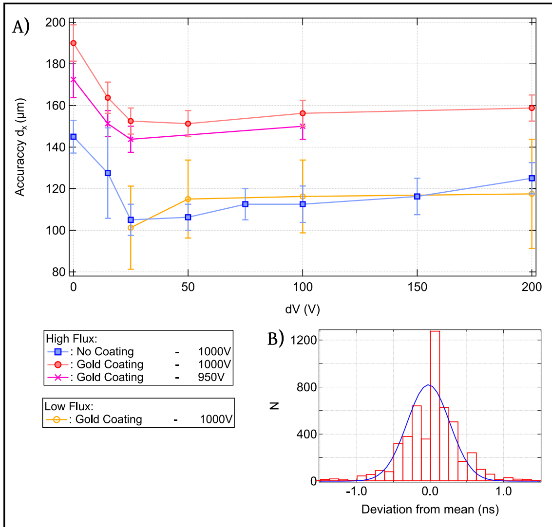
Figure 1.20: A) The accuracy of the detector in \mu\text{m} for different configurations of the detector. B) The distribution of \sigma_D for the point at dV = 25\text{ V} for the non-coated MCP.
