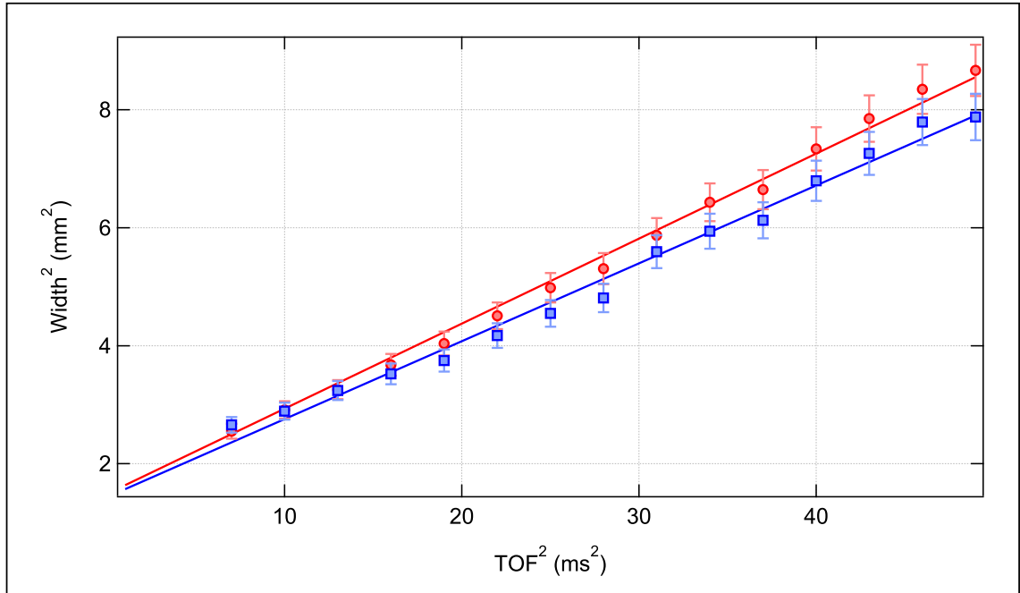
Figure 3.4: A time of flight picture after red molasses. The fit gives a T_x = 134.7 \pm 3.7 \mu\text{K} and T_y = 111, 6 \pm 4.6 \mu\text{K} . For the initial size this gives \sigma_x = 2.4 \pm 0.2 \text{ mm} and \sigma_y = 2.5 \pm 0.2 \text{ mm} .
