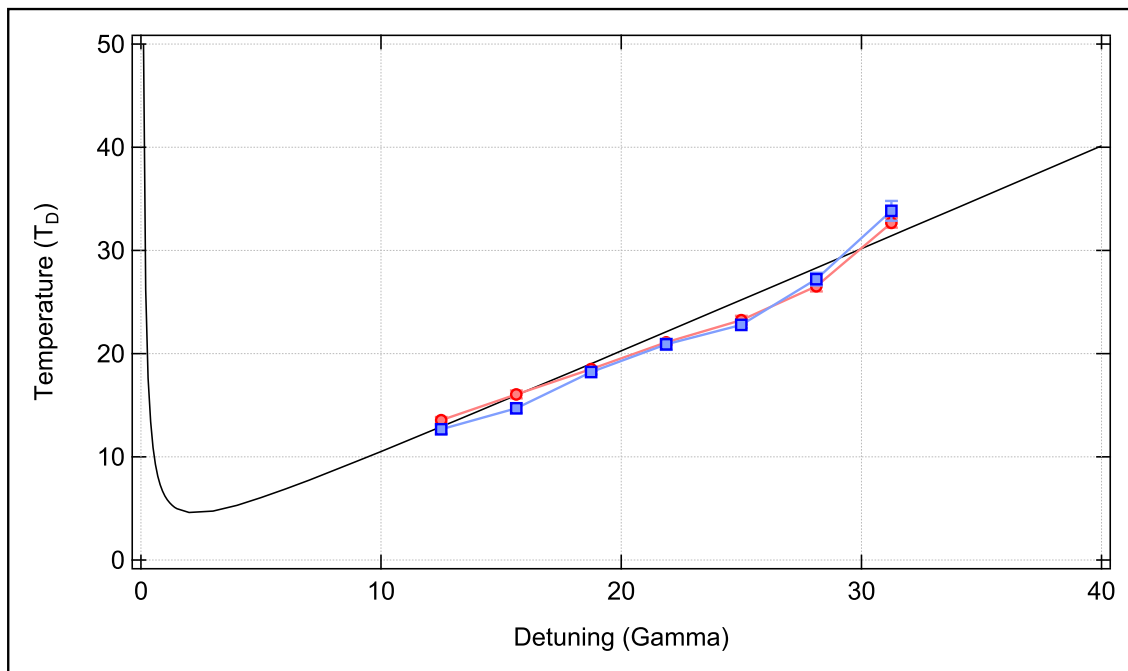
Figure 3.12: The temperature of the cloud of atoms in the MOT for different detunings of the light with I = 4I_{sat} per beam. Red circles: x-direction; Blue squares: y-direction. The line is two-level Doppler theory with the used experimental parameters.
