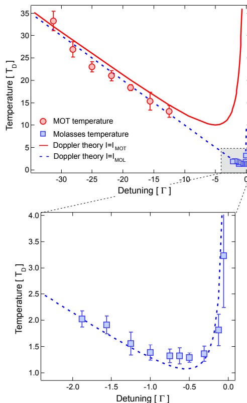
FIG. 1. Temperature in magneto-optical trap and optical molasses as a function of the detuning of the laser cooling beams. Temperatures are extracted from monitoring time-of-flight expansion of the gas. Error bars (one standard deviation) reflect the error from fitting. The total intensity (sum of the six beams) used in the experiment are respectively I_{\text{MOT}} = 100 I_{\text{sat}} and I_{\text{MOL}} = I_{\text{sat}}/10 . The lines are the results of Doppler theory of Eq. 7, for intensities I_{\text{MOT}} (solid line) and I_{\text{MOL}} (dashed line).
