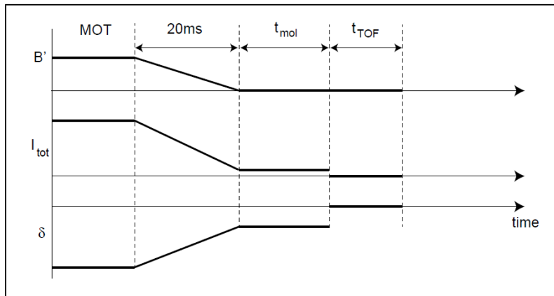
Figure 3.14: The time sequence used to obtain the temperature measurement at lower detunings. After the initial MOT stage the magnetic field gradient, intensity and detuning are ramped down to their desired values in 20 ms. The cloud is left for t_{mol} \simeq 20 ms to equilibrate. Afterwards we take TOF pictures to get the temperature.
