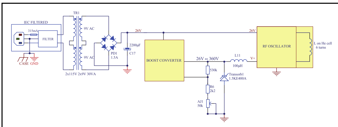
Figure 2.8: The total electrical scheme that is inside the box. The voltage V+ is controlled with the potentiometer, allowing us to manually adjust it.
