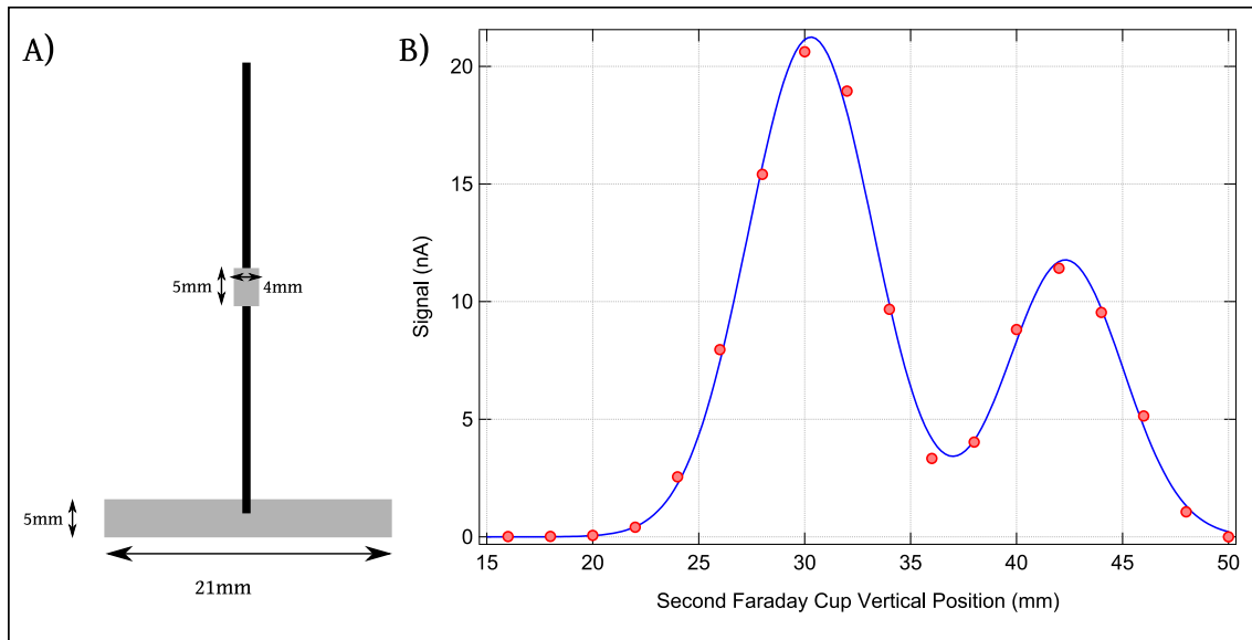
Figure 2.20: A) Schematic view of the second Faraday cup in between the two Zeeman slowers. The small plate is 5 mm by 4 mm, whereas the large plate at the bottom is 5 mm by 21 mm, the wire in between the plates is coated and non-conductive. B) Example measurement taken with the Faraday cup by moving the instrument in the vertical direction. The line is a double Gaussian fit. The lower maximum peak comes from particles collected by the small plate, and the total maximum peak from the particles collected by the larger plate.
