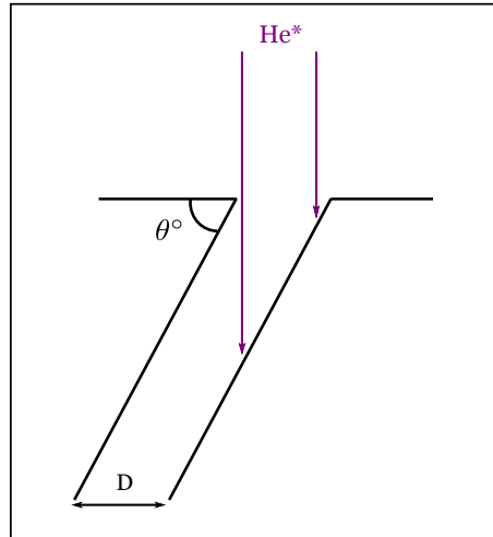
Figure 1.21: The accuracy in the z -direction is determined by the angle \theta of the channels of the MPC and the diameter D : d_z = D/\tan\theta . Particles hitting on the left will get a different arrival time as particles hitting the channel on the right, even though their z -coordinate is the same.
