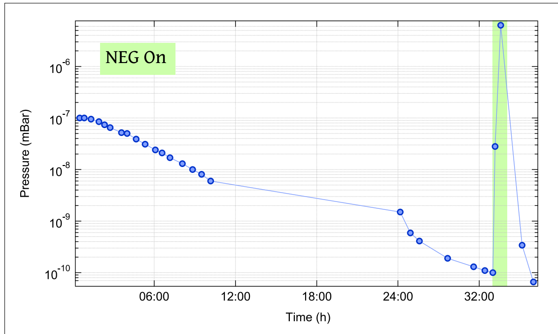
Figure 2.5: The pressure in the science chamber during the cooling down phase of the baking. At t = 0 the chamber is gradually cooled back to room temperature. The activation of the NEG is show in green. The final pressure in the science chamber at room temperature is 6.6 \times 10^{-11} mBar.
