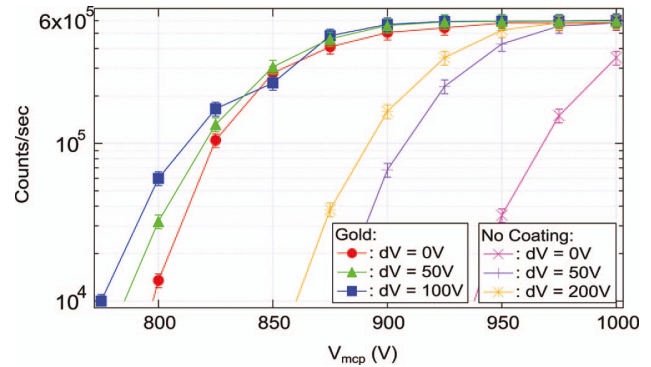
FIG. 4. Count rates as a function of V_{\text{mcp}} for the two pairs of MCPs and for different voltage differences dV . Incoming flux \sim 1.5 \times 10^{11} photons/s.
