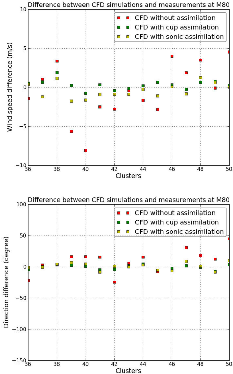
Figure 5.7: Difference between CFD simulations without assimilation and measurements, CFD simulations with cup assimilation and measurement and CFD simulations with sonic assimilation and measurement at M80 (80m) a) wind speed b) direction.
