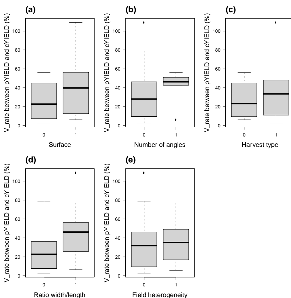
Figure 2.7: Variation rate (V_rate) between plot yield and commercial yield as a function of: a) Field surface; b) Field number of angles; c) Harvest type; d) Field ratio width/length; e) Field heterogeneity
