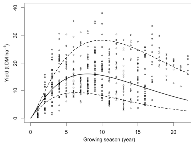
Figure 4. 2: Yield evolution of M. giganteus as a function of crop age.
