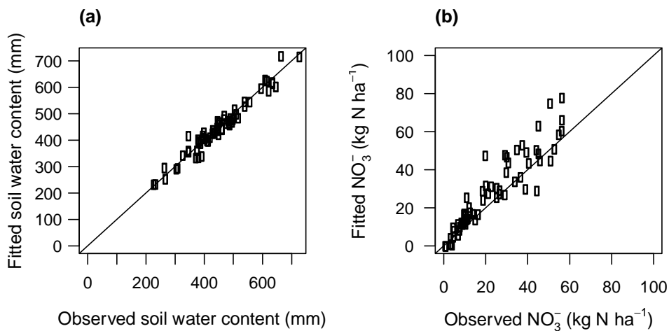
Figure 3.4: Comparison between observed and simulated values of: a) soil water content (mm) and b) soil nitrate ( \text{kg N ha}^{-1} ) in late winter for both years.
