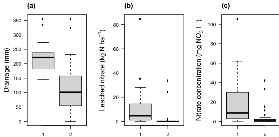
Figure 3. 5: LIXIM simulation results: a) drained water, b) leached nitrate and c) mean nitrate concentration in drained water
