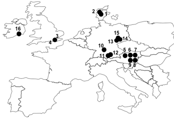
Figure 4. 1: Location of the experimental sites included in the M. giganteus long-term yield database (a site can include several experimental units, cf. Annexe 2).
