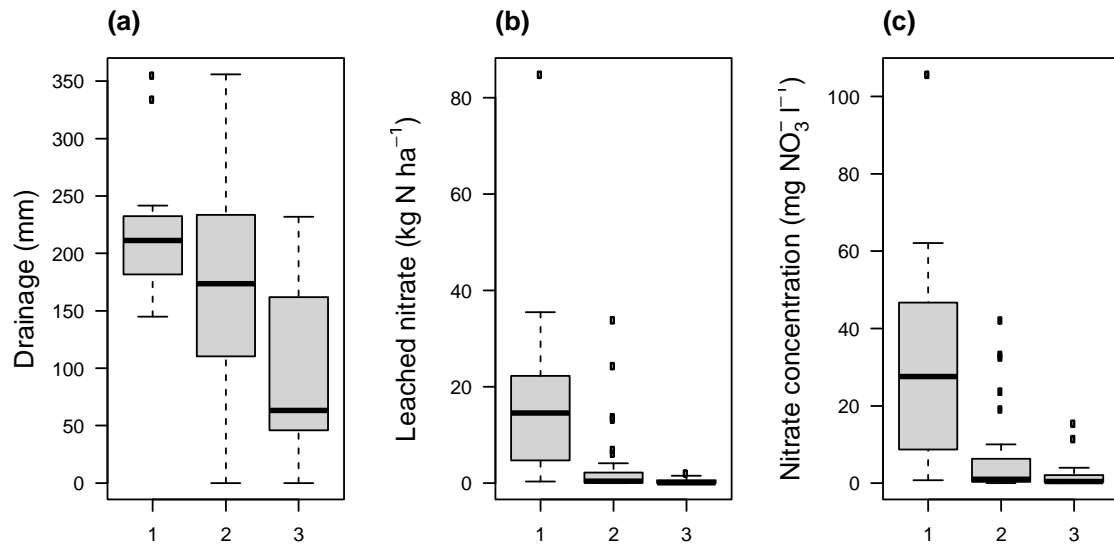
Figure 3. 7: LIXIM simulation results as a function of crop age: a) drained water (mm), b) leached nitrate (kg N ha -1 ) and c) mean nitrate concentration in drained water (mg NO 3 - l -1 ).
