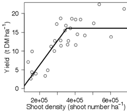
Figure 2. 1: Variation in yield as a function of shoot density for growth years 2 and 3.
