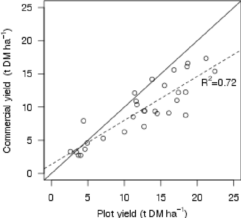
Figure 2. 6: Relationship between commercial yields and plot yields.
