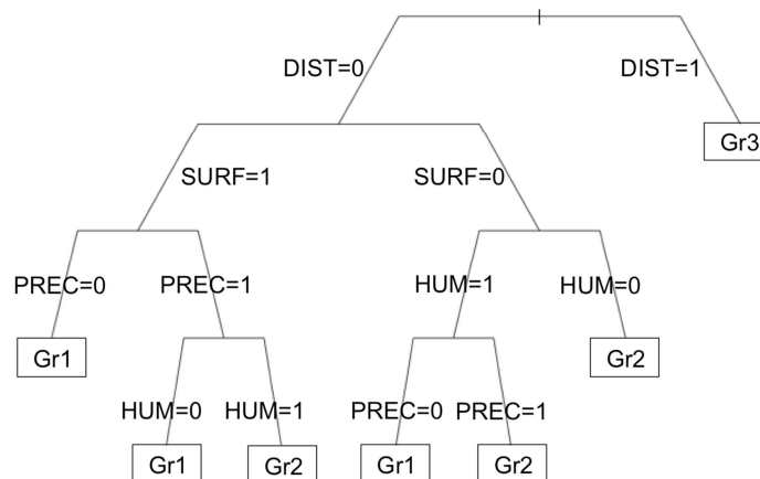
Figure 2. 5: Classification tree of the factors related to the weed cover measured at the end of the establishment year.
