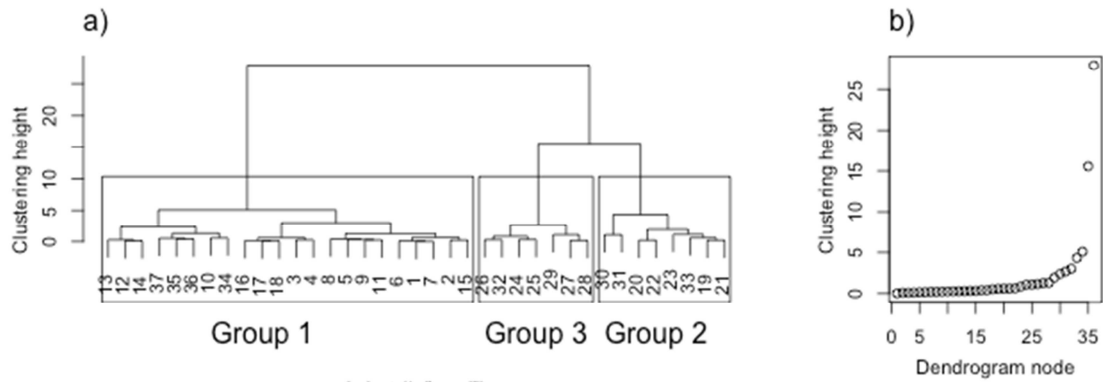
Figure 4. 7: a) Dendrogram of the experimental units and b) node distance graph as basis for grouping them into three groups.
