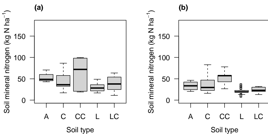
Figure 3.3: Total soil mineral nitrogen measured at the beginning of winter a) 2010 and b) 2011 as a function of soil type.
