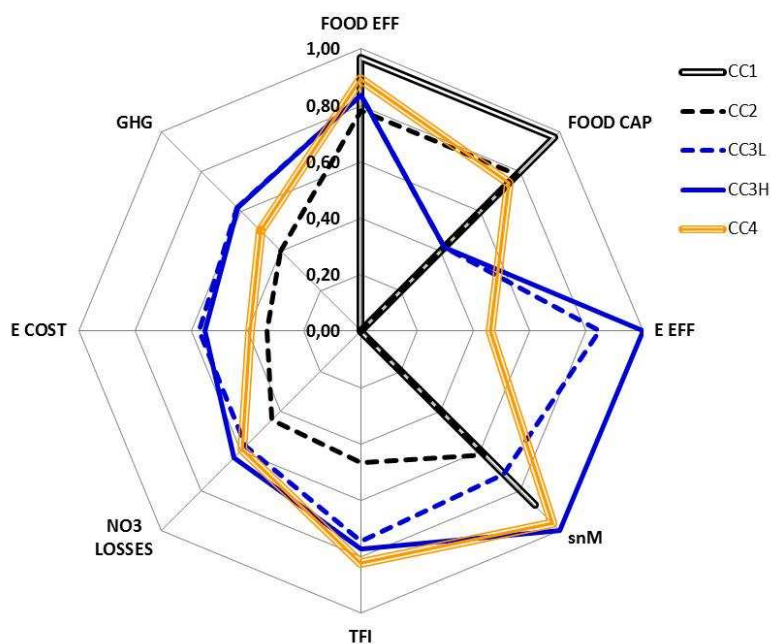
Figure 5. 3: Cropping system multicriteria assessment: a) LC soil; b) CC soil.
