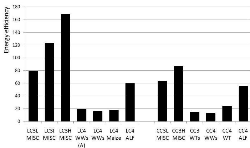
Figure 5. 9: Energy efficiency of the different energy feedstocks.
