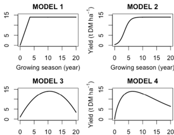
Figure 4. 3: Compared models for long-term yield trends.
