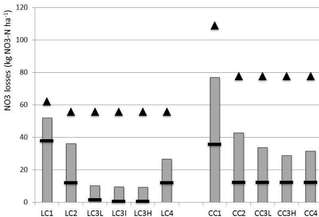
Figure 5. 6: Assessment of nitrate losses (kg N ha -1 ).
