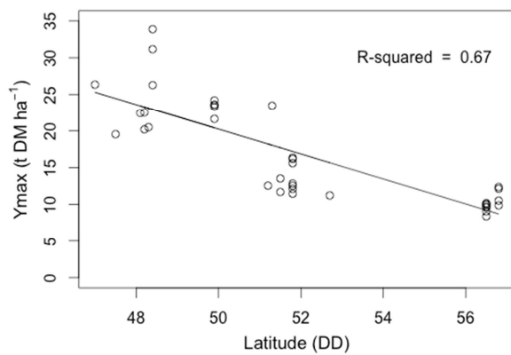
Figure 4. 9: Variation of Ymax as a function of latitude.
