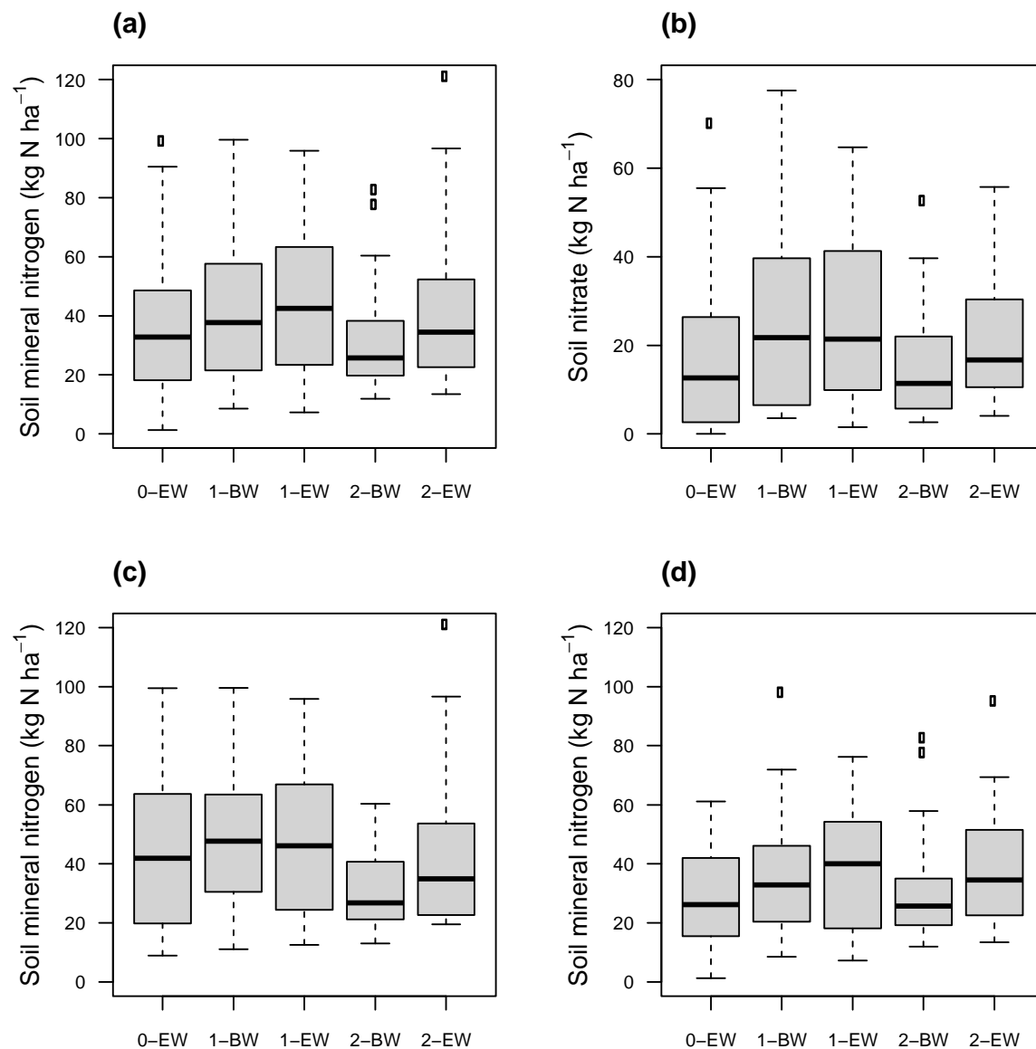
Figure 3. 1: a) Total soil mineral nitrogen (kg N ha -1 ), b) Soil nitrate (kg N ha -1 ), c) Total soil mineral nitrogen for fields which were set-aside before the plantation of M. giganteus (kg N ha -1 ), d) Total soil mineral nitrogen for fields where arable crops were grown before the plantation of M. giganteus (kg N ha -1 ).
