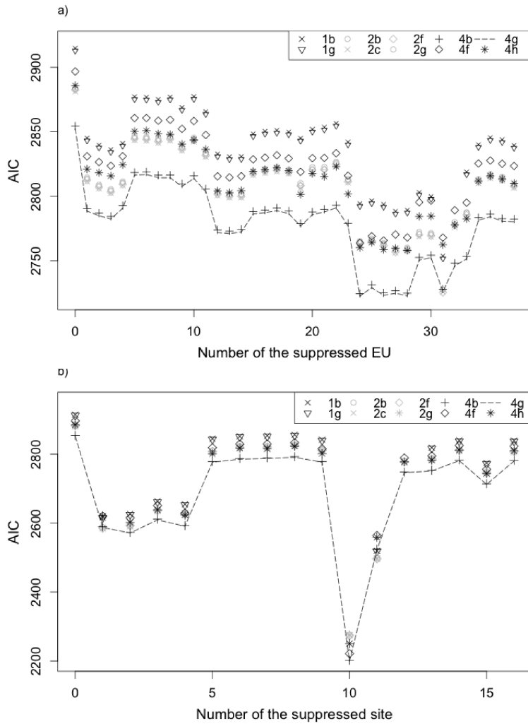
Figure 4. 4: Sensitivity analysis to the data, a) at the experimental unit level (EU) and b) at the site level.
