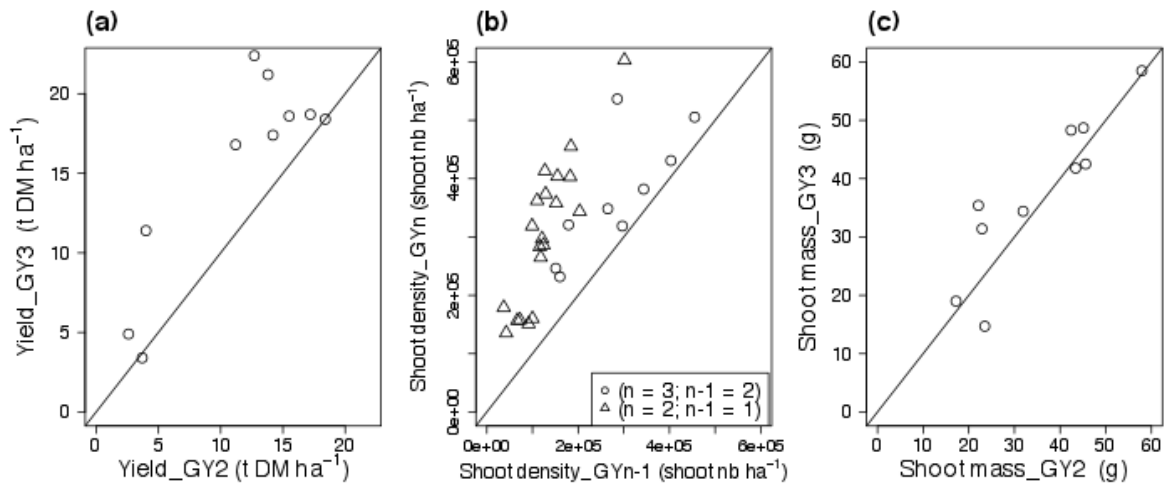
Figure 2. 2: Inter-annual relationships between a) yields, b) shoot densities and c) shoot masses.
