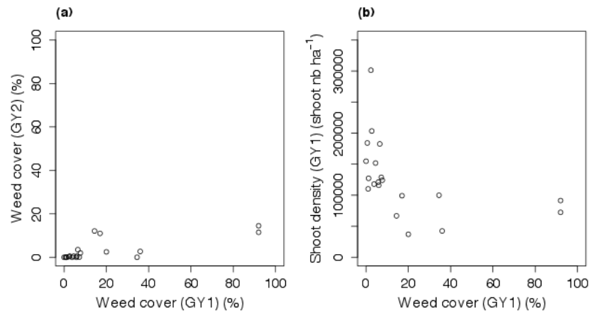
Figure 2. 4: Influence of weed cover: a) evolution of weed cover between growth year 1 and growth year 2; b) shoot density as a function of weed cover at the end of GY1.
