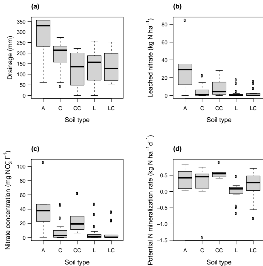
Figure 3. 4: LIXIM simulation results as a function of soil type: a) drained water; b) leached nitrate; c) mean nitrate concentration in drained water; d) potential N mineralization rate.
