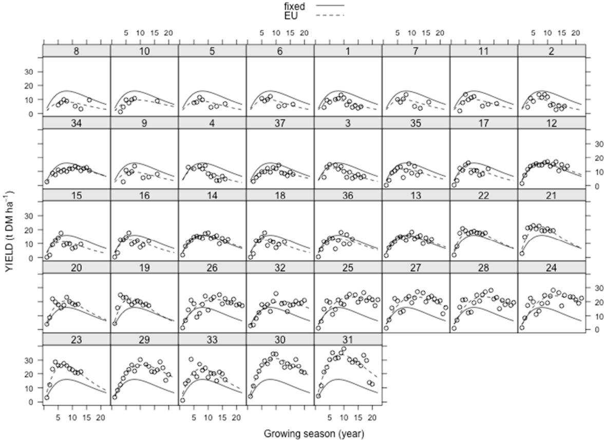
Figure 4. 6: Mean predictions (solid line) and experimental unit (EU) adjusted predictions (dashed line) of M. giganteus yield trends from the selected growth model (4g).
