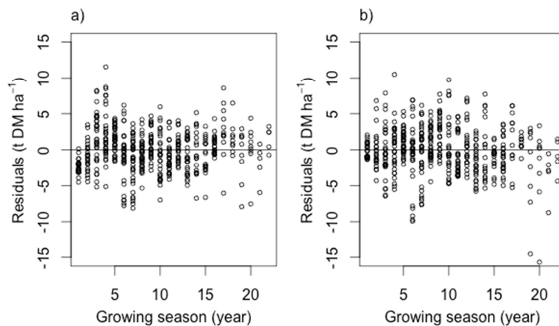
Figure 4. 5: Residual distributions for a) model (4g) and b) model (2c).
