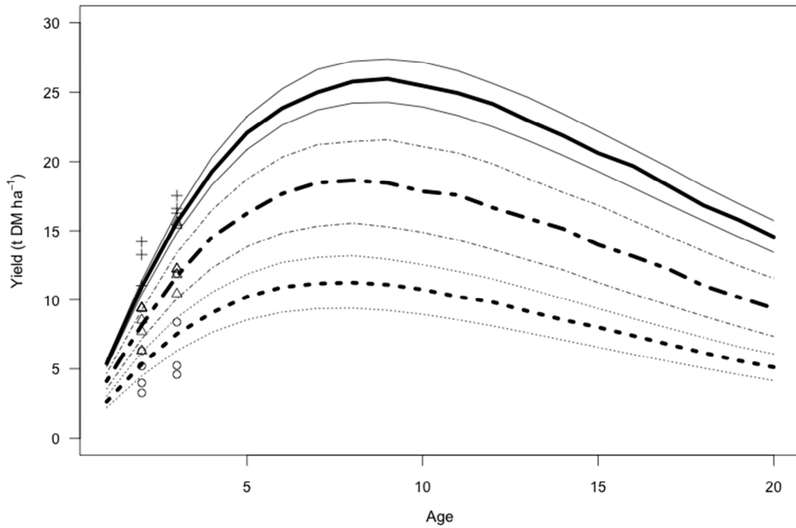
Figure 5. 2: Yield scenarios for M. giganteus .
