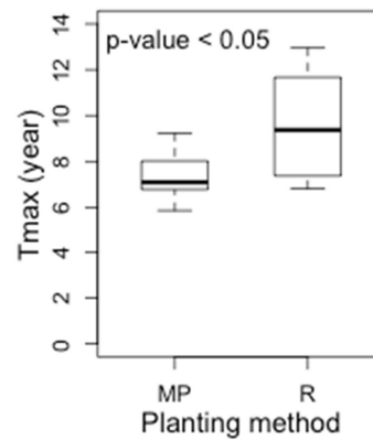
Figure 4. 10: Variation of Tmax as a function of the planting mode.
