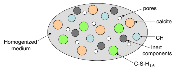
Figure 1. Representation of the cement paste REV.
