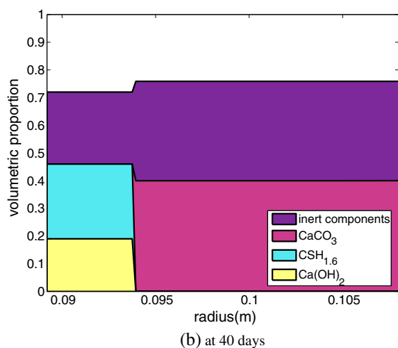
Figure 3. Spatial repartition of molar quantities of the CH, C-S-H and CaCO 3 under CO 2 injection at different times.
