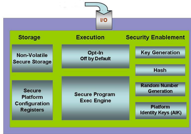
FIGURE 5.3 – Composition d'un module TPM.
