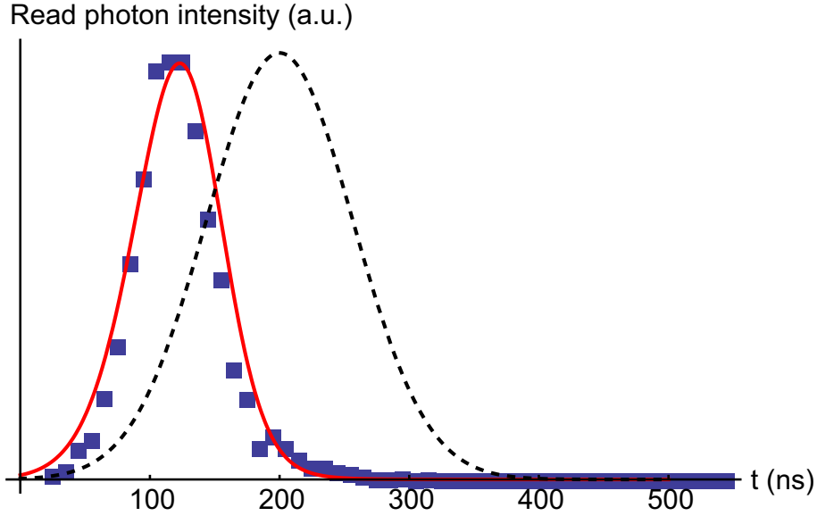
Figure 9.9: Histogram of arrival times of the Read photons (blue squares), superimposed with the form \Gamma_{cav}(t)e^{-\int^t \xi\Gamma_{cav}(t')dt'} for approximate experimental parameters (solid red) and corresponding Read pulse profile (dashed black).
