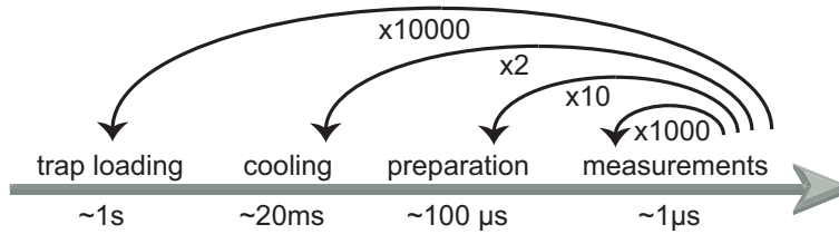
Figure 4.3: Typical sequence behaviour. The measurements themselves are made of short periods ( \sim 1\mu\text{s} ) repeated a large number of times ( \sim 1000 ) which have to be alternated with preparation steps regularly, and maybe integrated into some larger loop of re-cooling the atoms, before having to reload the trap. The generation and data acquisition inside a measurement step must be resolved on \sim 10\text{ ns} timescale.
