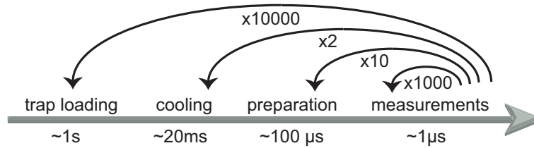
Figure 4.3: Typical sequence behaviour. The measurements themselves are made of short periods ( \sim 1\ \mu\text{s} ) repeated a large number of times ( \sim 1000 ) which have to be alternated with preparation steps regularly, and maybe integrated into some larger loop of re-cooling the atoms, before having to reload the trap. The generation and data acquisition inside a measurement step must be resolved on \sim 10\ \text{ns} timescale.
