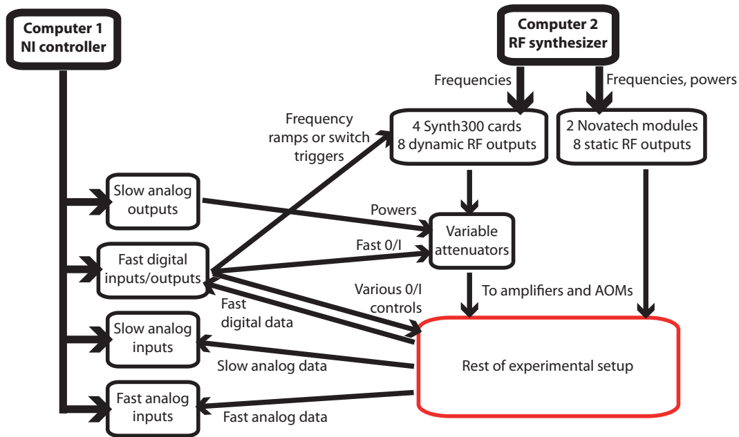
Figure 4.2: Schematic of the structure of our complete control and acquisition system.
