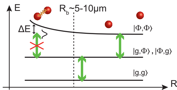
Figure 5: Rydberg blockade mechanism. In the two-atom basis, the system starts from its ground state |g, g\rangle , and due to a laser excitation with a finite linewidth (green arrows), each atom can be excited from |g\rangle to a Rydberg state |\Phi\rangle . However, from the singly excited state, the interactions shift the doubly excited one |\Phi, \Phi\rangle out of resonance for interatomic distances R below a certain blockade radius R_b .
