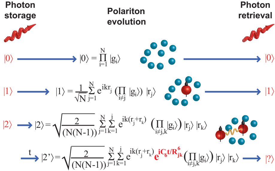
Figure 13.3: Illustration of the “quantum scissors” effect by letting the polaritons dephase before readout. When photonic quantum states |0\rangle or |1\rangle are stored, interactions have no effect, the state remains phase-matched and can be readout. However when two excitations are stored initially, each component of the state where atoms j and k , separated by a distance R_{jk} , are excited acquires a phase C_6 t/R_{jk}^6 , which quickly ruins the phase-matching and prevents the excitations from being readout.
