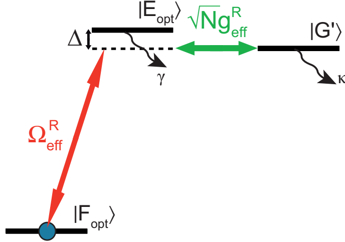
Figure 8.3: {N atoms+cavity field} states considered in the treatment of the Read step from the optimally coupled state.
